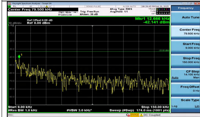
Band5_1.4MHz_QPSK_20643_6RB#0_0.009~0.15_0.009~0.15
