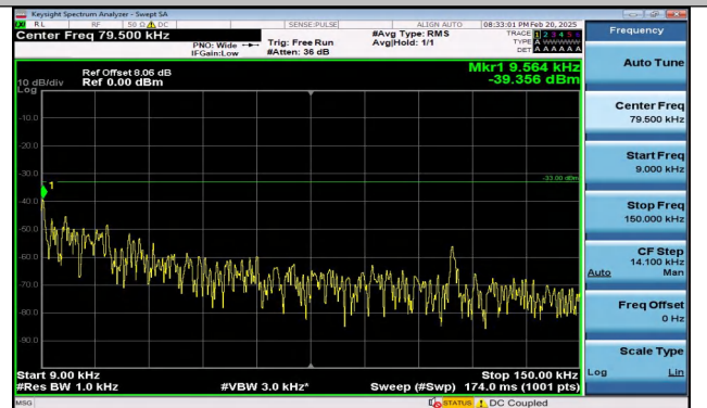
Band5_1.4MHz_QPSK_20525_1RB#5_0.009~0.15_0.009 ~0.15
