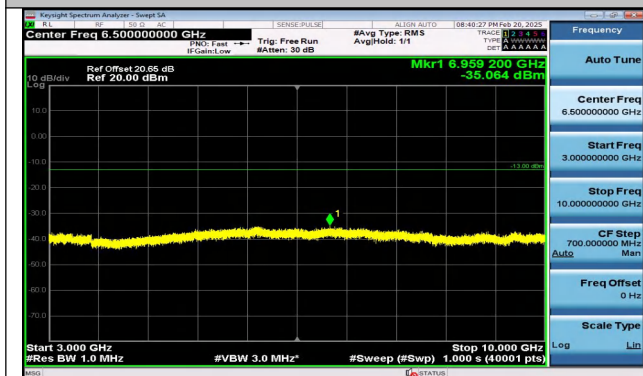
Band5_1.4MHz_QPSK_20643_6RB#0_3000~10000_3000~10000
