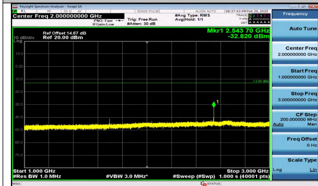
Band5_1.4MHz_16QAM_20643_1RB#0_1000~3000_1000
