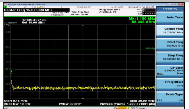
Band5_1.4MHz_16QAM_20643_1RB#5_0.15~30_0.15~3
