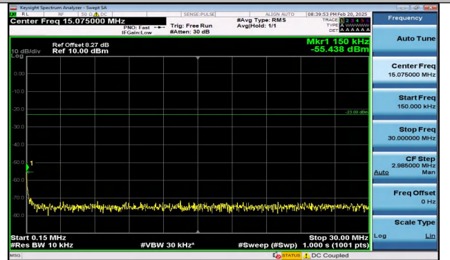
Band5_1.4MHz_QPSK_20643_6RB#0_0.15~30_0.15~30
