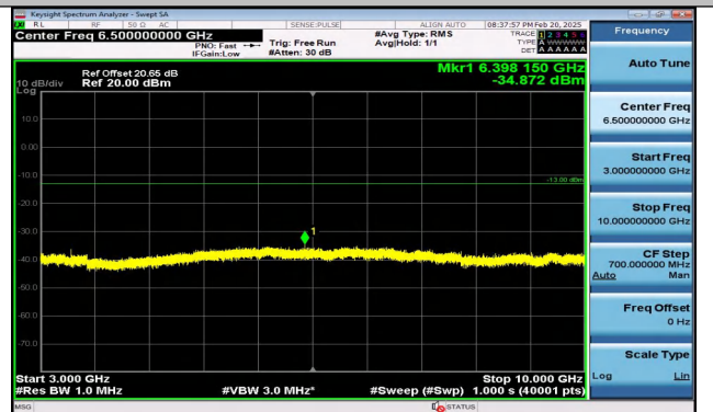
Band5_1.4MHz_16QAM_20643_1RB#0_3000~10000_300
