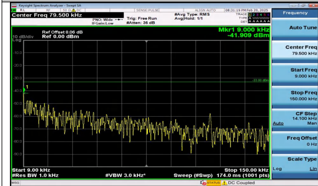
Band5_1.4MHz_QPSK_20525_1RB#0_0.009~0.15_0.009 ~0.15
