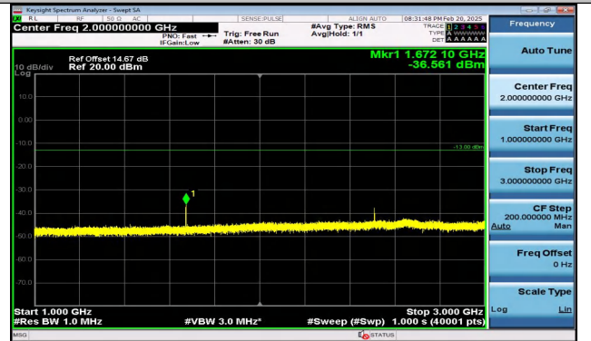
Band5_1.4MHz_QPSK_20525_1RB#0_1000~3000_1000~3000
