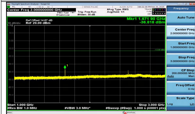
Band5_1.4MHz_16QAM_20525_1RB#0_1000~3000_1000 ~3000
