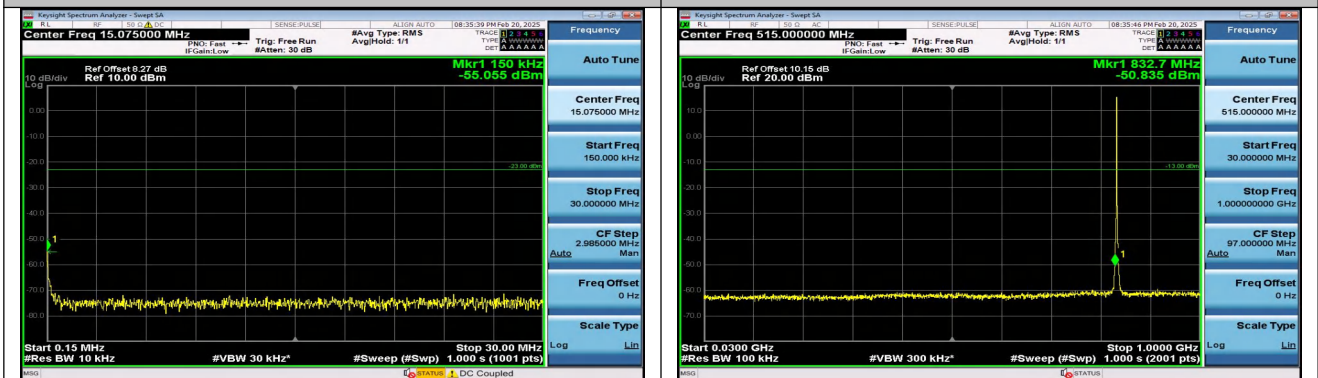
Band5_1.4MHz_16QAM_20525_6RB#0_0.15~30_0.15~30
