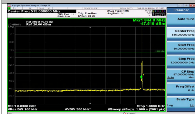
Band5_1.4MHz_16QAM_20643_1RB#5_30~1000_30~10
