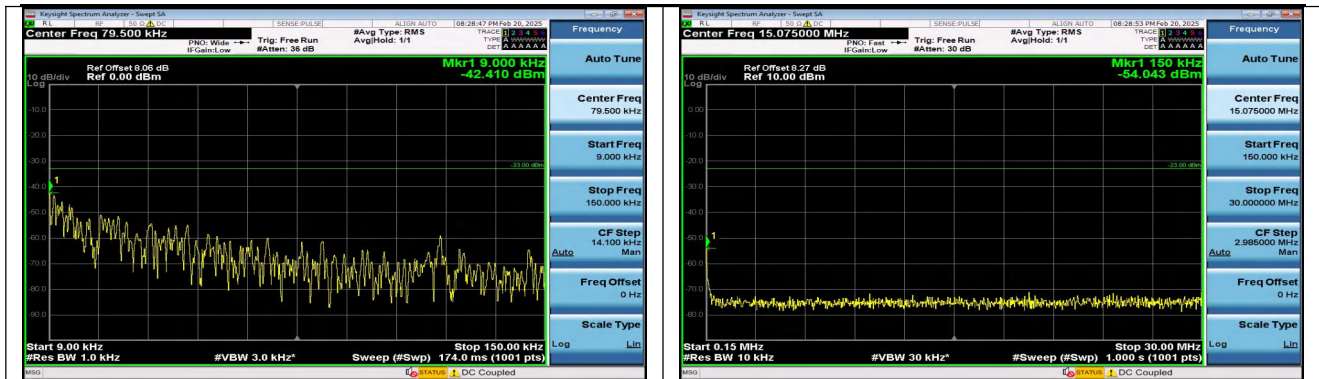
Band5_1.4MHz_16QAM_20407_1RB#5_0.009~0.15_0.00 9~0.15
