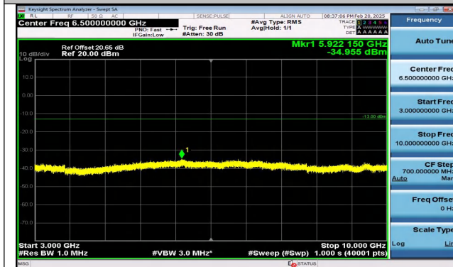
Band5_1.4MHz_QPSK_20643_1RB#0_3000~10000_3000 ~10000
