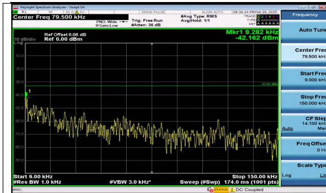
Band5_1.4MHz_QPSK_20643_1RB#0_0.009~0.15_0.009 ~0.15
