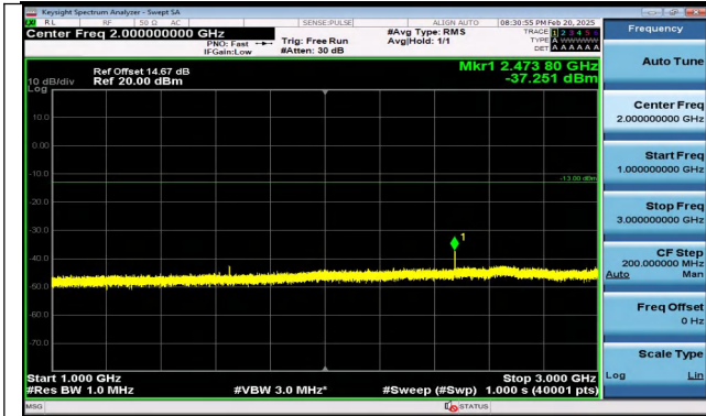
Band5_1.4MHz_16QAM_20407_6RB#0_1000~3000_1000 ~3000
