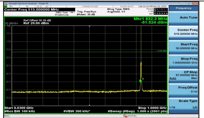
Band5_1.4MHz_16QAM_20525_1RB#0_30~1000_30~10 00
