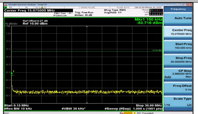
Band5_1.4MHz_16QAM_20525_1RB#5_0.15~30_0.15~3 0
