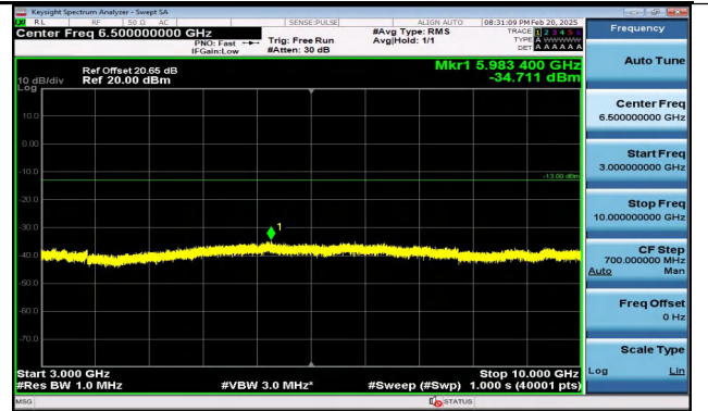
Band5_1.4MHz_16QAM_20407_6RB#0_3000~10000_300 0~10000
