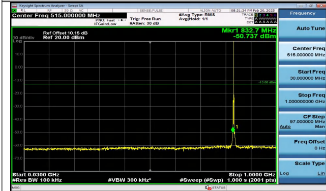
Band5_1.4MHz_QPSK_20525_1RB#0_30~1000_30~1000
