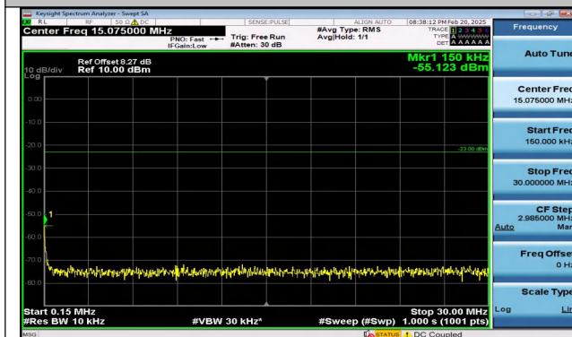
Band5_1.4MHz_QPSK_20643_1RB#5_0.15~30_0.15~30
