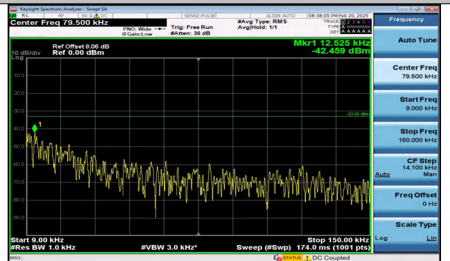
Band5_1.4MHz_QPSK_20643_1RB#5_0.009~0.15_0.009 ~0.15
