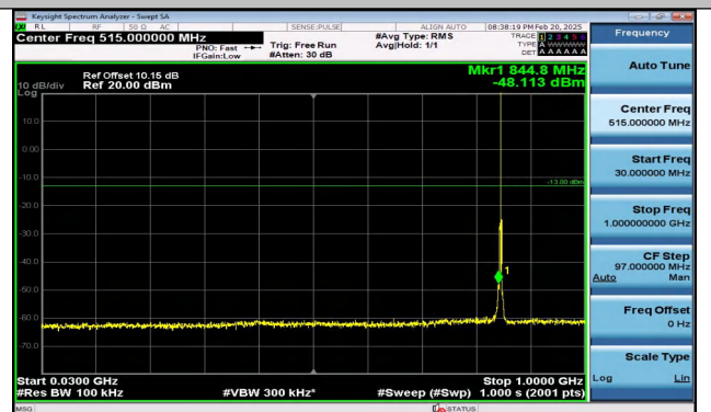
Band5_1.4MHz_QPSK_20643_1RB#5_30~1000_30~1000
