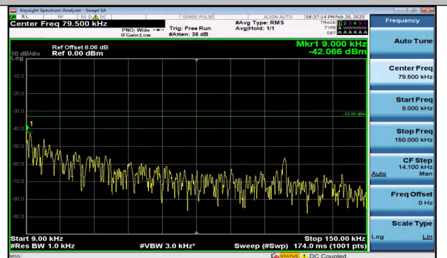
Band5_1.4MHz_16QAM_20643_1RB#0_0.009~0.15_0.009~0.15
