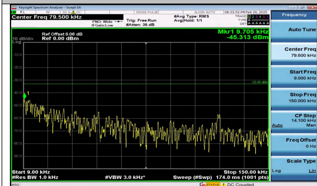
Band5_1.4MHz_16QAM_20525_1RB#5_0.009~0.15_0.00 9~0.15
