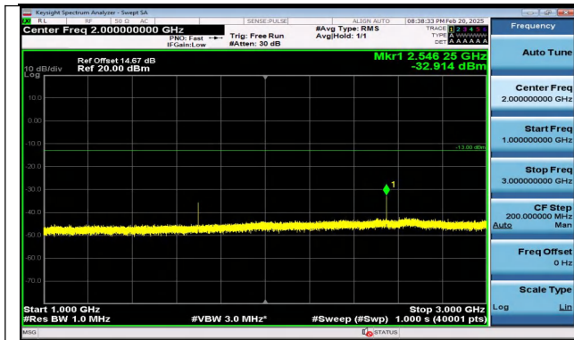
Band5_1.4MHz_QPSK_20643_1RB#5_1000~3000_1000~3000
