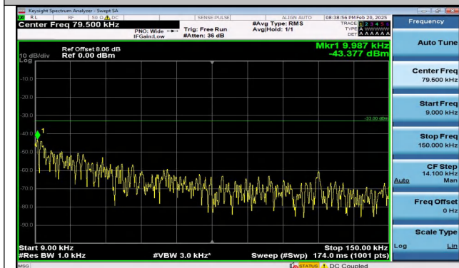
Band5_1.4MHz_16QAM_20643_1RB#5_0.009~0.15_0.00
