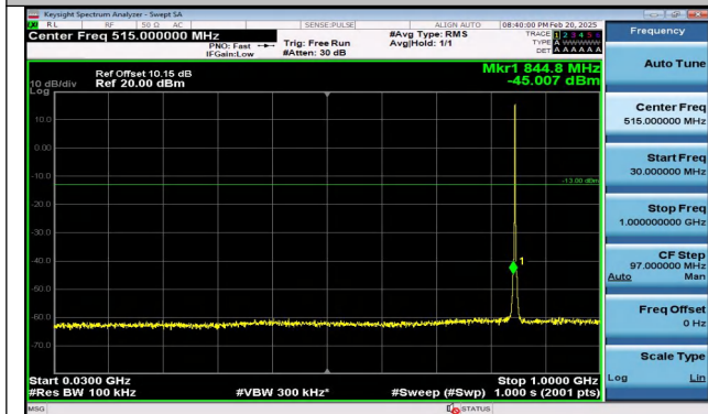
Band5_1.4MHz_QPSK_20643_6RB#0_30~1000_30~1000
