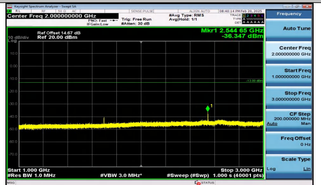
Band5_1.4MHz_QPSK_20643_6RB#0_1000~3000_1000~3000
