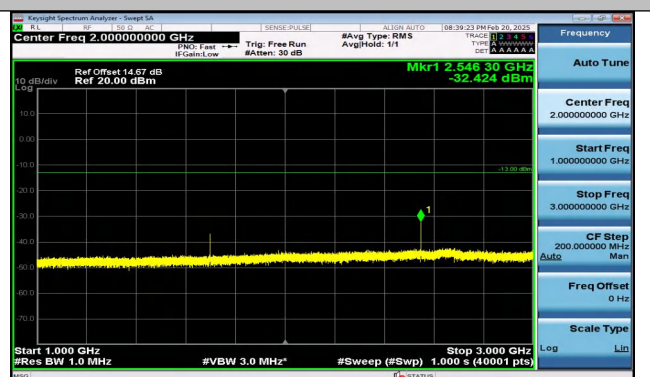
Band5_1.4MHz_16QAM_20643_1RB#5_1000~3000_1000
