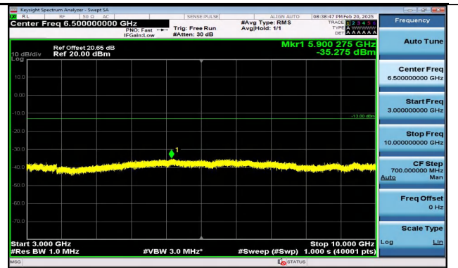
Band5_1.4MHz_QPSK_20643_1RB#5_3000~10000_3000~10000
