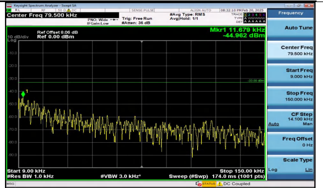
Band5_1.4MHz_16QAM_20525_1RB#0_0.009~0.15_0.00 9~0.15
