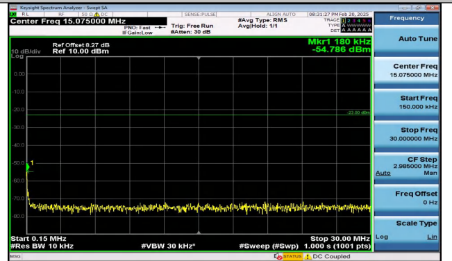
Band5_1.4MHz_QPSK_20525_1RB#0_0.15~30_0.15~30
