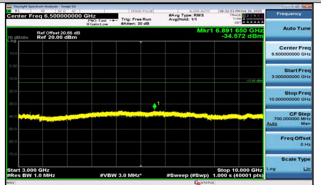
Band5_1.4MHz_16QAM_20525_1RB#0_3000~10000_300 0~10000
