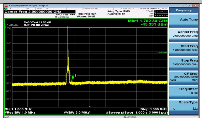
Band4_20MHz_QPSK_20050_1RB#0_1000~3000_1000~
