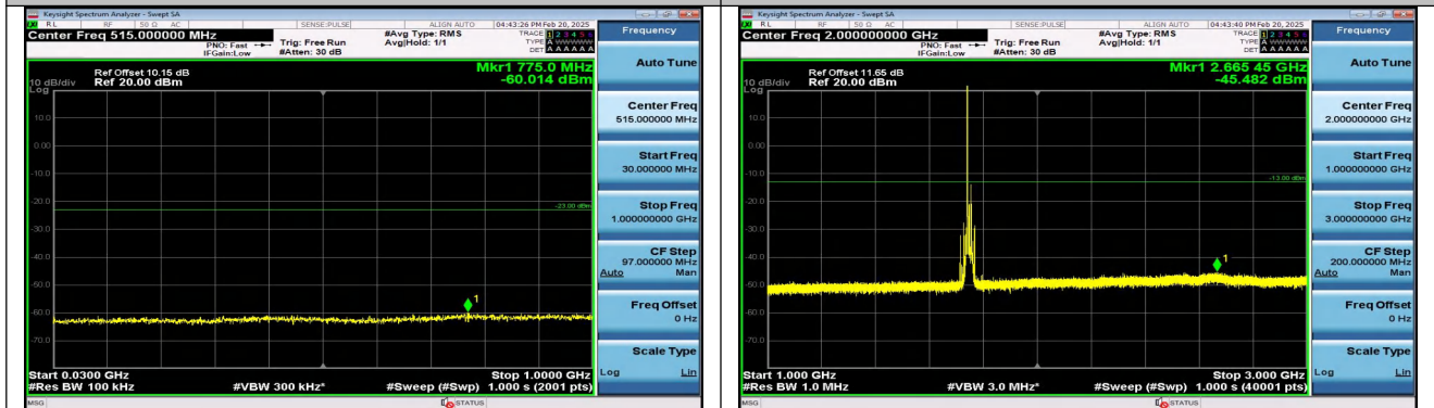
Band4_15MHz_16QAM_20325_1RB#0_30~1000_30~100 0
