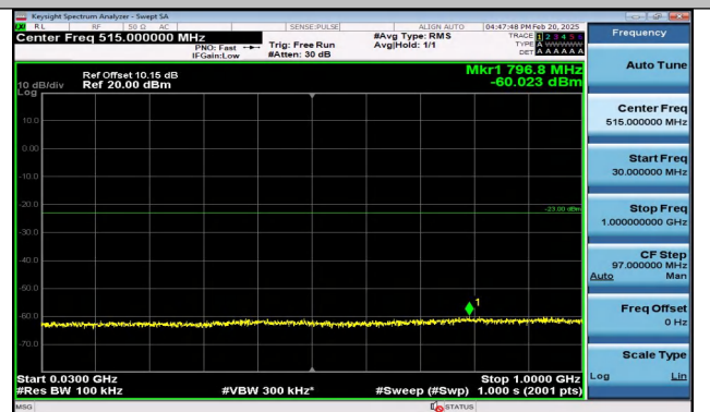
Band4_15MHz_QPSK_20325_75RB#0_30~1000_30~100 0
