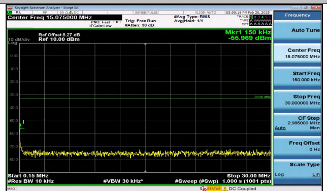
Band4_20MHz_QPSK_20050_1RB#0_0.15~30_0.15~30
