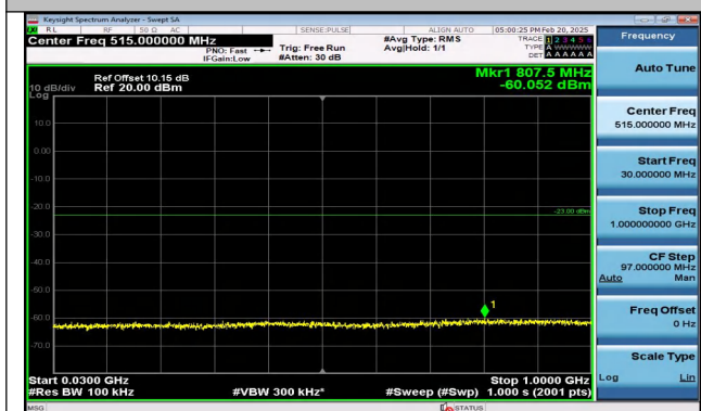
Band4_20MHz_QPSK_20050_1RB#0_30~1000_30~1000
