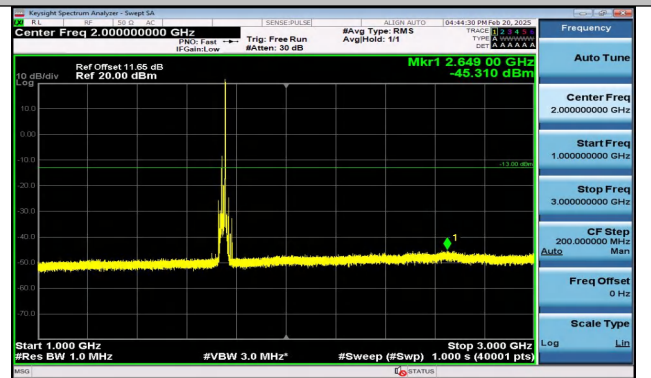
Band4_15MHz_QPSK_20325_1RB#74_1000~3000_1000 ~3000
