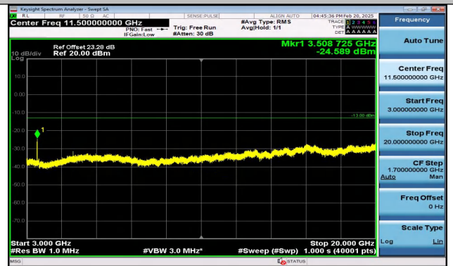
Band4_15MHz_16QAM_20325_1RB#74_3000~20000_30
