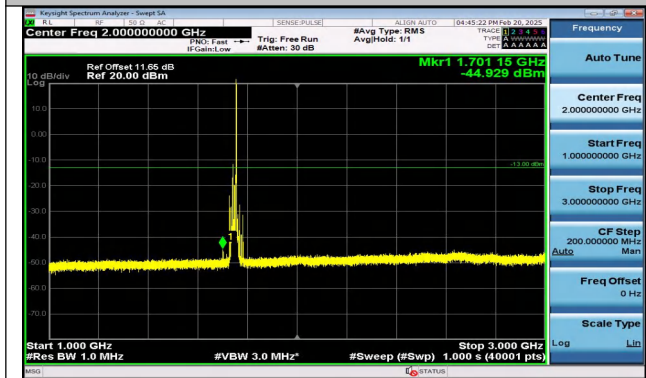
Band4_15MHz_16QAM_20325_1RB#74_1000~3000_100
