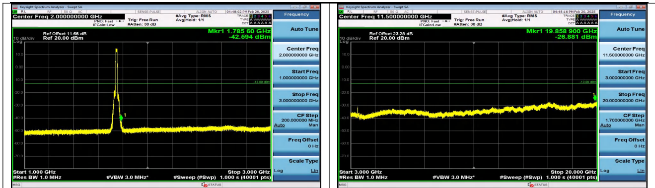
Band4_15MHz_QPSK_20325_75RB#0_1000~3000_1000 ~3000
