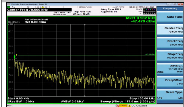
Band4_20MHz_QPSK_20050_1RB#0_0.009~0.15_0.009~
