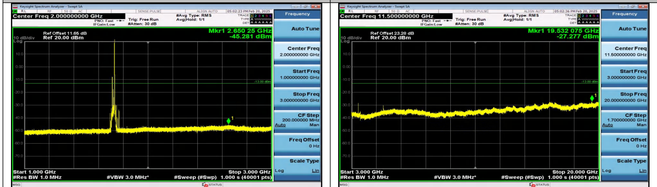
Band4_20MHz_QPSK_20050_1RB#99_1000~3000_1000 ~3000
