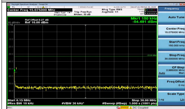
Band4_15MHz_QPSK_20325_75RB#0_0.15~30_0.15~30
