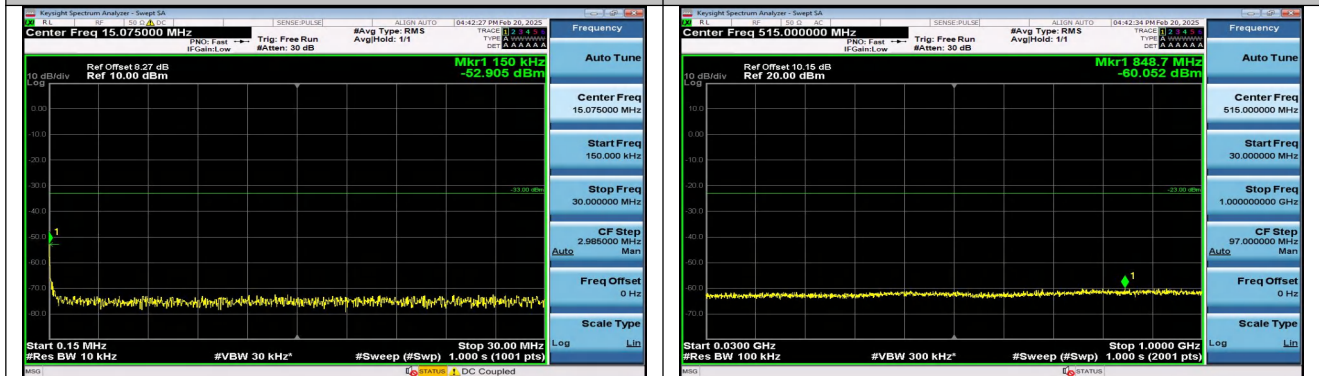
Band4_15MHz_QPSK_20325_1RB#0_0.15~30_0.15~30
