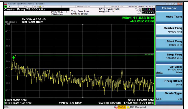
Band4_15MHz_QPSK_20325_75RB#0_0.009~0.15_0.009 ~0.15
