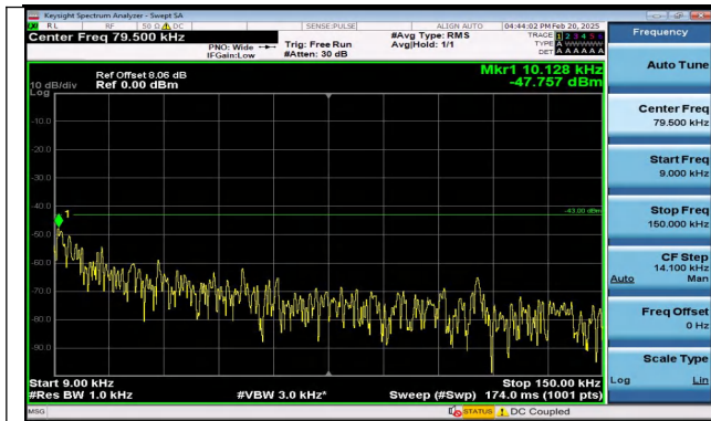
Band4_15MHz_QPSK_20325_1RB#74_0.009~0.15_0.009 ~0.15
