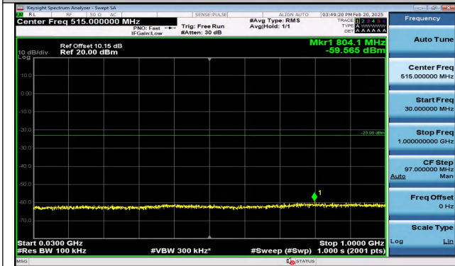
Band4_5MHz_QPSK_20375_1RB#0_30~1000_30~1000
