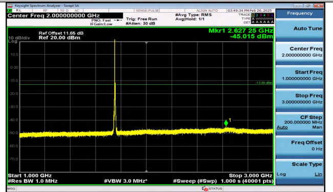
Band4_5MHz_QPSK_20375_1RB#0_1000~3000_1000~3000
