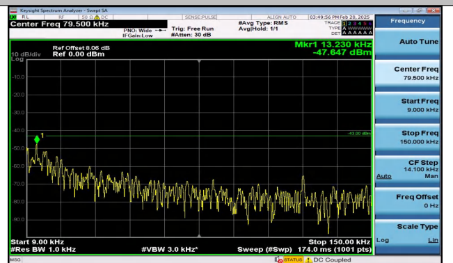
Band4_5MHz_16QAM_20375_1RB#0_0.009~0.15_0.009~0.15
