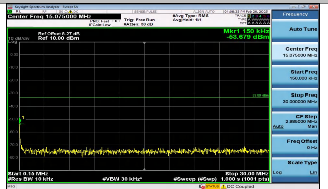
Band4_10MHz_QPSK_20000_1RB#0_0.15~30_0.15~30
