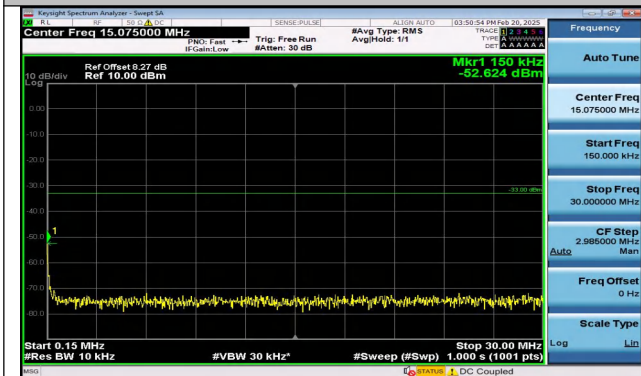
Band4_5MHz_QPSK_20375_1RB#24_0.15~30_0.15~30
