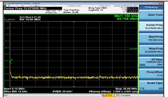
Band4_5MHz_QPSK_20375_25RB#0_0.15~30_0.15~30
