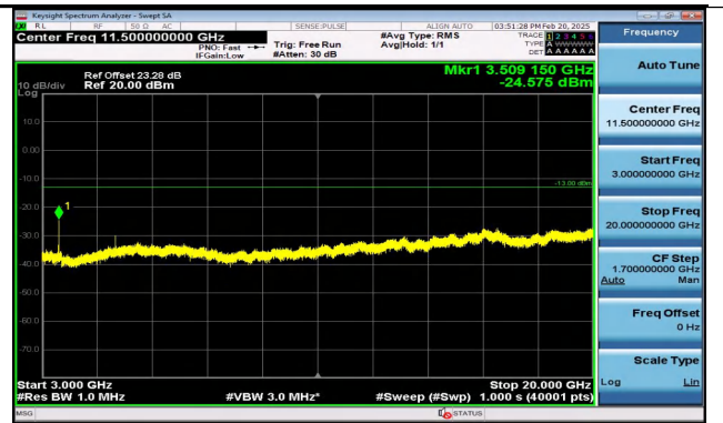
Band4_5MHz_QPSK_20375_1RB#24_3000~20000_3000~20000
