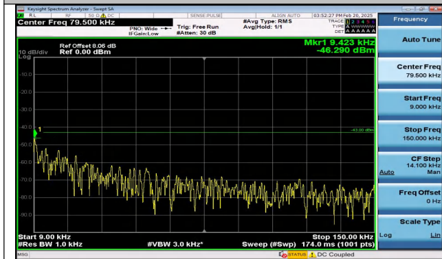
Band4_5MHz_QPSK_20375_25RB#0_0.009~0.15_0.009~0.15
