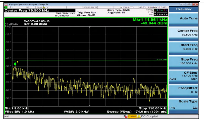
Band4_5MHz_16QAM_20375_25RB#0_0.009~0.15_0.009 ~0.15
