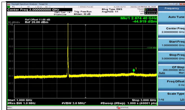
Band4_5MHz_QPSK_20375_1RB#24_1000~3000_1000~3000
