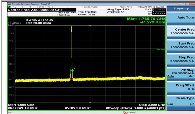
Band4_5MHz_16QAM_20375_25RB#0_1000~3000_1000 ~3000
