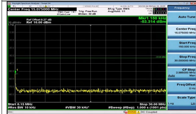
Band4_5MHz_16QAM_20375_25RB#0_0.15~30_0.15~30
