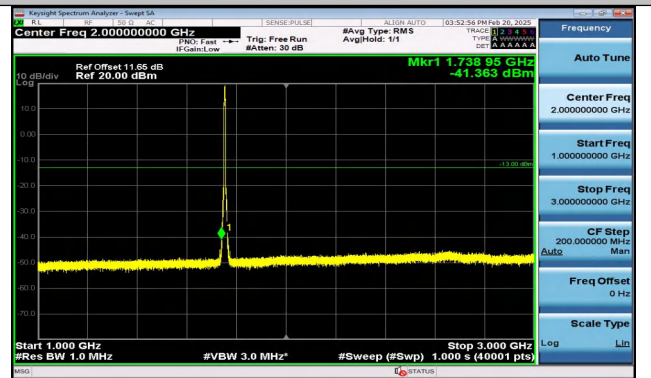
Band4_5MHz_QPSK_20375_25RB#0_1000~3000_1000~3000
