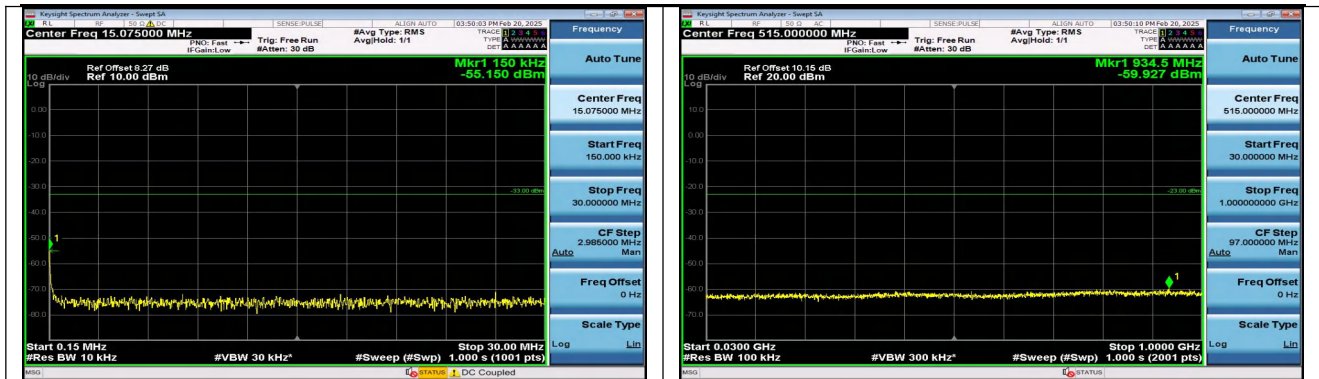
Band4_5MHz_16QAM_20375_1RB#0_0.15~30_0.15~30
