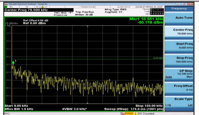
Band4_5MHz_QPSK_20375_1RB#24_0.009~0.15_0.009~0.15
