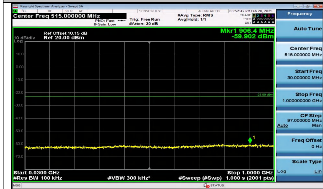
Band4_5MHz_QPSK_20375_25RB#0_30~1000_30~1000
