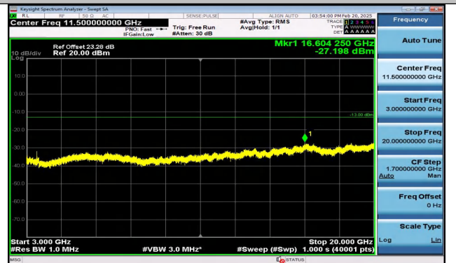
Band4_5MHz_16QAM_20375_25RB#0_3000~20000_300 0~20000
