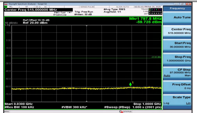
Band4_5MHz_QPSK_20375_1RB#24_30~1000_30~1000
