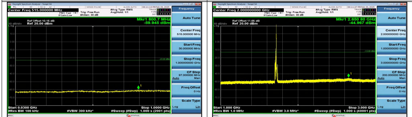
Band4_10MHz_16QAM_20000_1RB#49_30~1000_30~10 00
