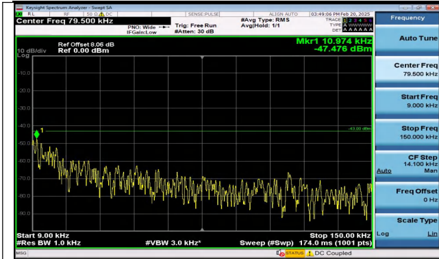
Band4_5MHz_QPSK_20375_1RB#0_0.009~0.15_0.009~0.15
