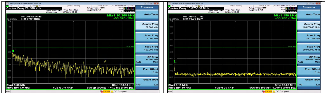
Band4_10MHz_QPSK_20000_50RB#0_0.009~0.15_0.009 ~0.15
