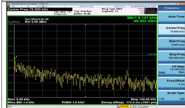
Band4_10MHz_QPSK_20000_1RB#0_0.009~0.15_0.009~0.15
