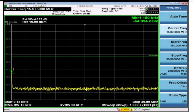
Band4_5MHz_QPSK_20375_1RB#0_0.15~30_0.15~30
