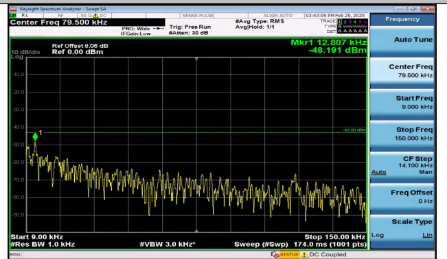
Band4_5MHz_16QAM_19975_25RB#0_0.009~0.15_0.009 ~0.15
