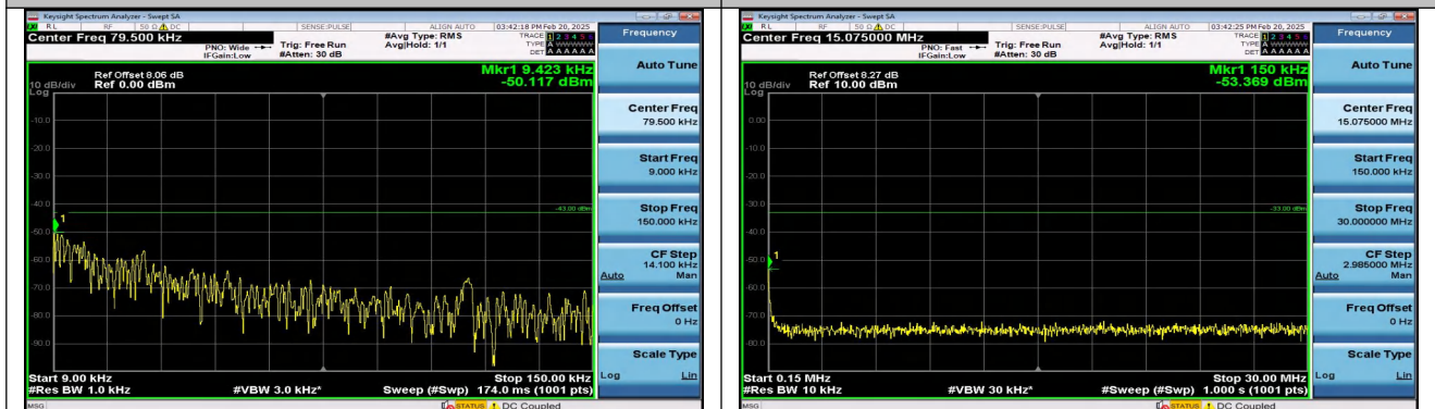
Band4_5MHz_QPSK_19975_25RB#0_0.009~0.15_0.009~0.15
