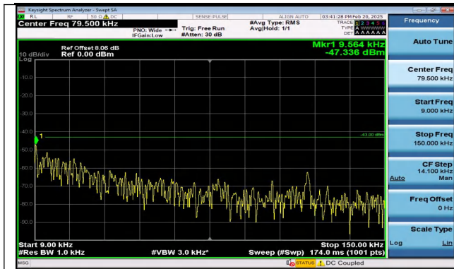
Band4_5MHz_16QAM_19975_1RB#24_0.009~0.15_0.009 ~0.15
