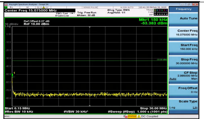
Band4_5MHz_16QAM_19975_1RB#24_0.15~30_0.15~30
