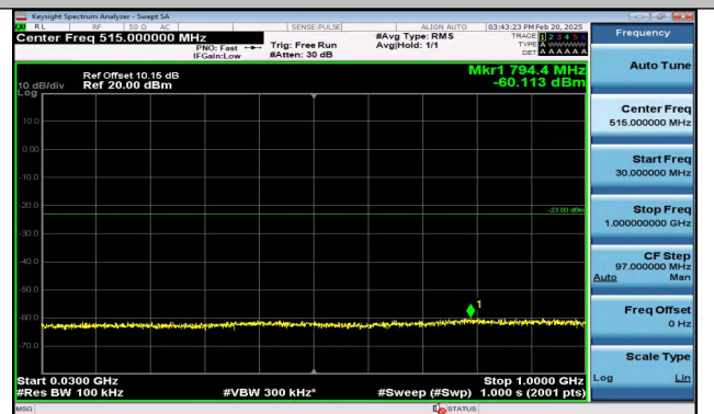
Band4_5MHz_16QAM_19975_25RB#0_30~1000_30~100 0
