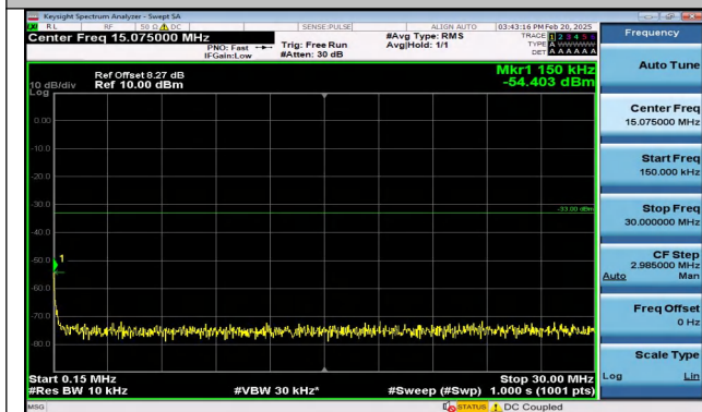
Band4_5MHz_16QAM_19975_25RB#0_0.15~30_0.15~30
