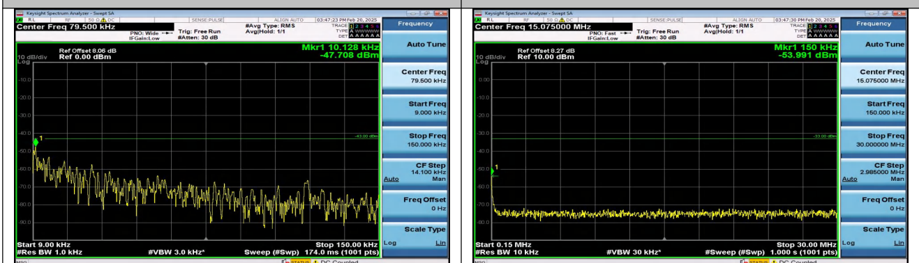
Band4_5MHz_QPSK_20175_25RB#0_0.009~0.15
