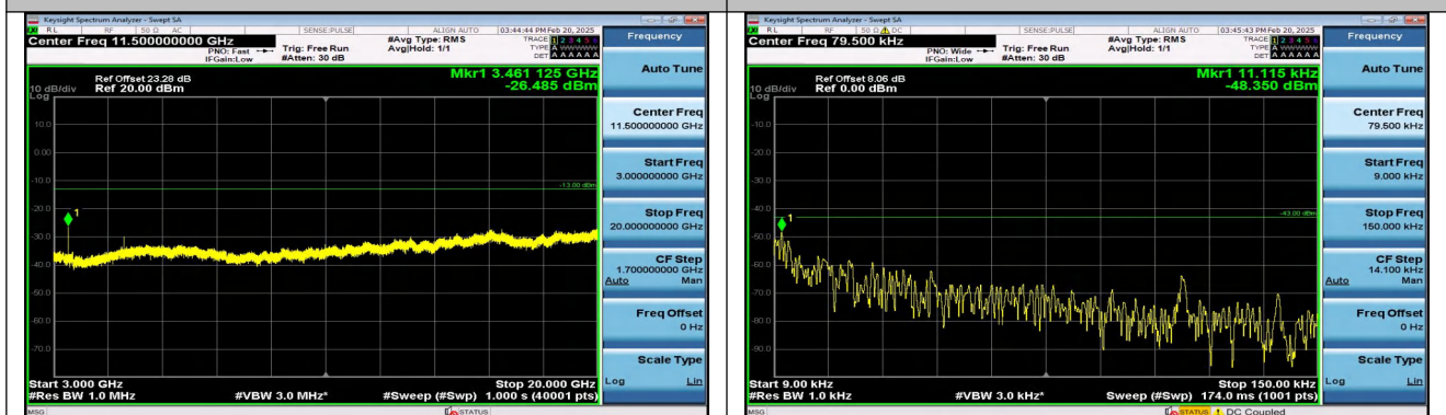
Band4_5MHz_QPSK_20175_1RB#0_3000~20000_3000~ 20000
