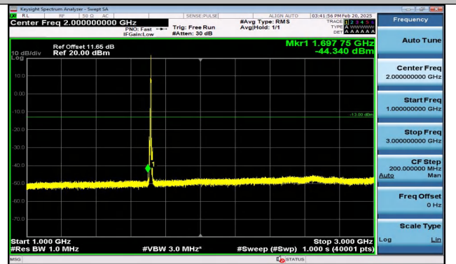
Band4_5MHz_16QAM_19975_1RB#24_1000~3000_1000 ~3000
