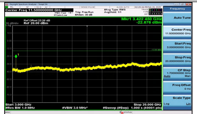
Band4_1.4MHz_QPSK_19957_1RB#5_3000~20000_3000~20000
