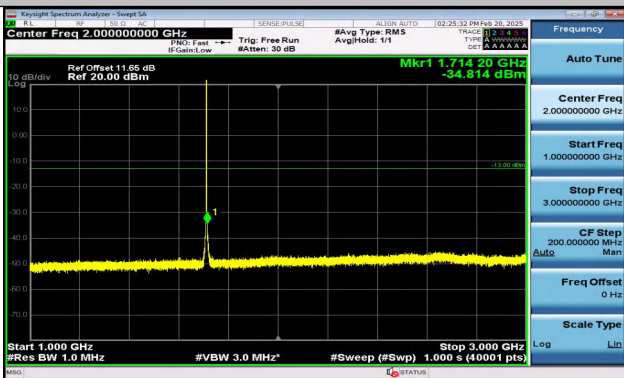
Band4_1.4MHz_QPSK_19957_1RB#5_1000~3000_1000~3000
