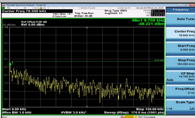
Band4_1.4MHz_QPSK_19957_6RB#0_0.009~0.15_0.009~0.15
