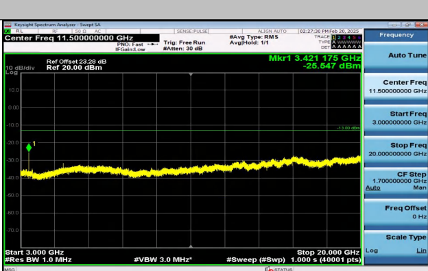
Band4_1.4MHz_QPSK_19957_6RB#0_3000~20000_3000~20000
