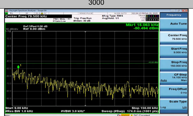
Band4_1.4MHz_16QAM_19957_1RB#0_0.009~0.15_0.009~0.15
