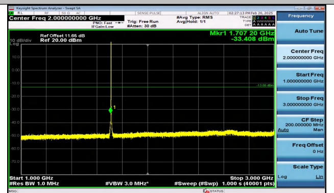
Band4_1.4MHz_QPSK_19957_6RB#0_1000~3000_1000~3000
