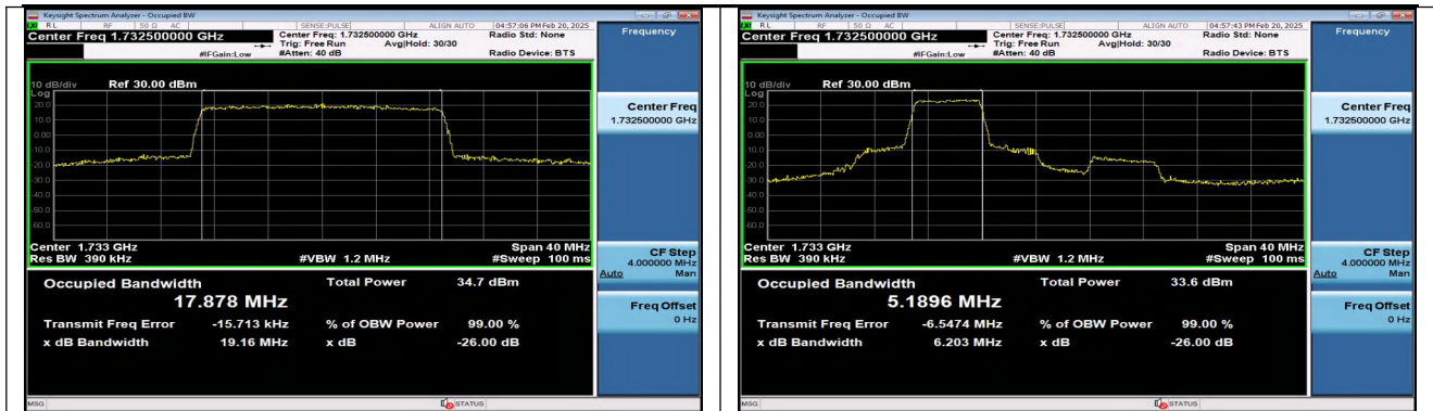
Band4-20MHz-QPSK-20175-100RB#0-PASS
