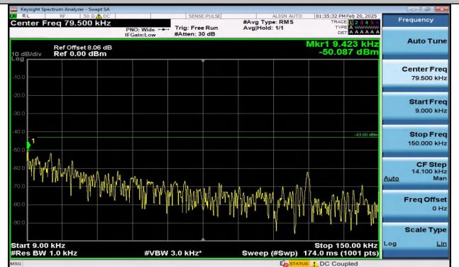
Band2_15MHz_QPSK_19125_75RB#0_0.009~0.15_0.009 ~0.15
