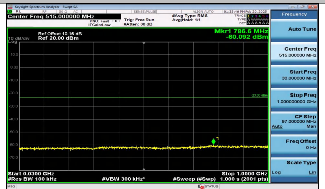
Band2_15MHz_QPSK_19125_75RB#0_30~1000_30~100 0
