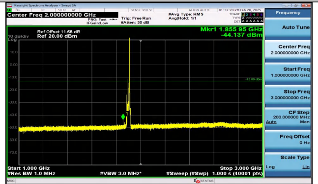
Band2_15MHz_QPSK_19125_1RB#74_1000~3000_1000 ~3000
