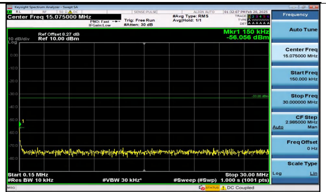
Band2_15MHz_QPSK_19125_1RB#74_0.15~30_0.15~30
