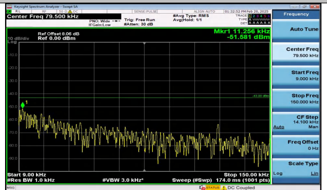
Band2_15MHz_16QAM_19125_1RB#74_0.009~0.15_0.00 9~0.15
