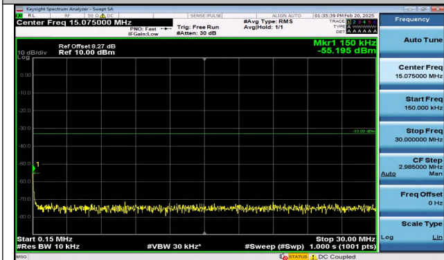
Band2_15MHz_QPSK_19125_75RB#0_0.15~30_0.15~30
