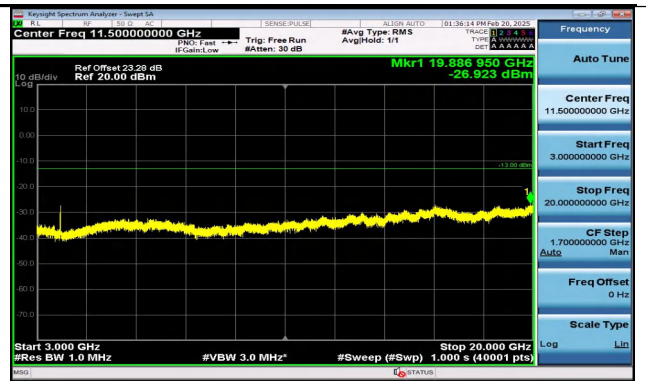
Band2_15MHz_QPSK_19125_75RB#0_3000~20000_300 0~20000
