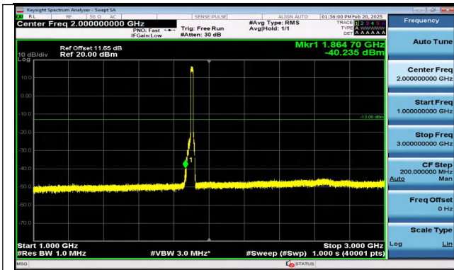
Band2_15MHz_QPSK_19125_75RB#0_1000~3000_1000 ~3000
