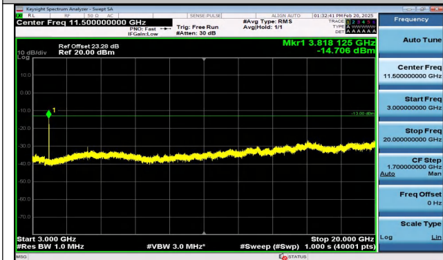
Band2_15MHz_QPSK_19125_1RB#74_3000~20000_300 0~20000
