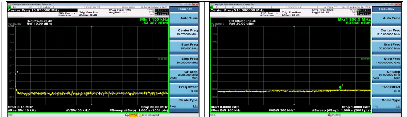
Band2_15MHz_QPSK_18900_1RB#74_30~1000_30~1000
