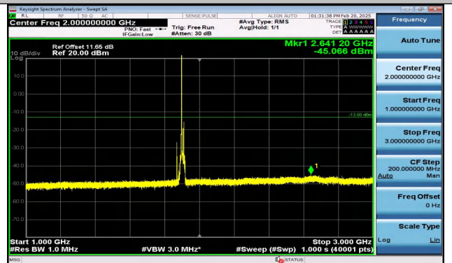
Band2_15MHz_16QAM_19125_1RB#0_1000~3000_1000 ~3000
