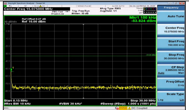
Band2_15MHz_16QAM_19125_1RB#0_0.15~30_0.15~30
