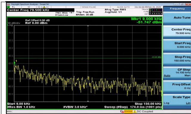
Band2_15MHz_QPSK_19125_1RB#74_0.009~0.15_0.009 ~0.15
