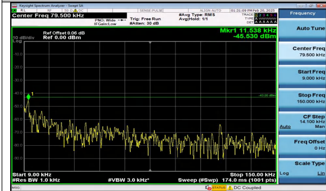
Band2_15MHz_16QAM_19125_1RB#0_0.009~0.15_0.009 ~0.15
