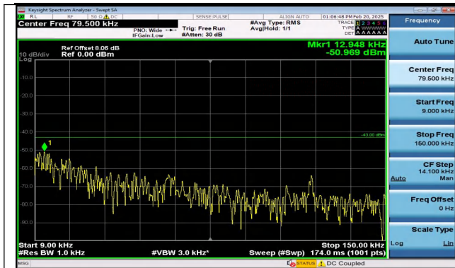
Band2_10MHz_QPSK_18650_50RB#0_0.009~0.15_0.009 ~0.15
