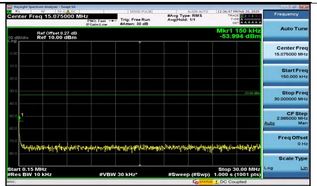
Band2_5MHz_QPSK_19175_1RB#0_0.15~30_0.15~30
