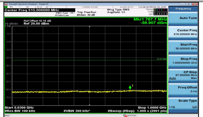
Band2_5MHz_QPSK_19175_1RB#24_30~1000_30~1000
