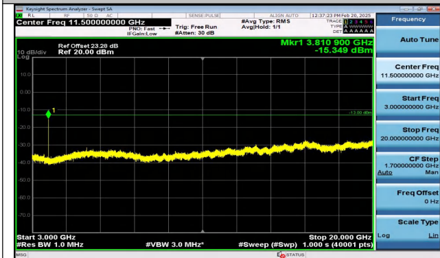
Band2_5MHz_QPSK_19175_1RB#0_3000~20000_3000~20000
