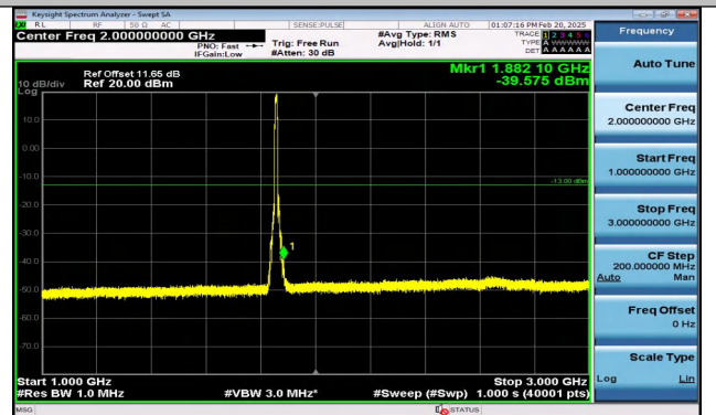
Band2_10MHz_QPSK_18650_50RB#0_1000~3000_1000 ~3000
