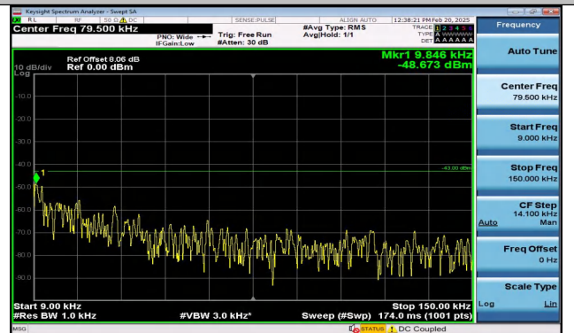
Band2_5MHz_QPSK_19175_1RB#24_0.009~0.15_0.009~0.15
