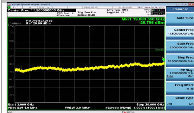
Band2_10MHz_QPSK_18650_50RB#0_3000~20000_300 0~20000
