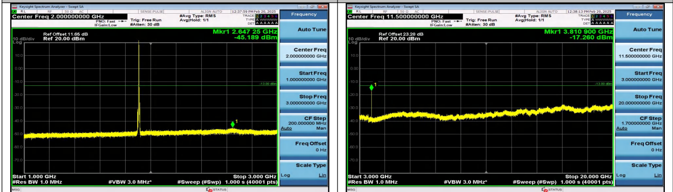
Band2_5MHz_16QAM_19175_1RB#0_1000~3000_1000~3000
