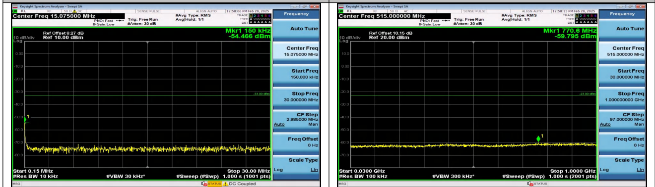
Band2_10MHz_QPSK_18650_1RB#49_30~1000_30~1000
