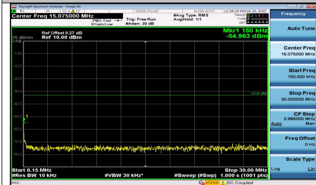
Band2_5MHz_QPSK_19175_1RB#24_0.15~30_0.15~30
