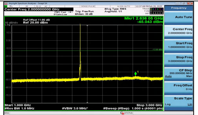
Band2_5MHz_QPSK_19175_1RB#0_1000~3000_1000~3000
