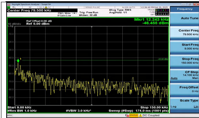
Band2_5MHz_QPSK_19175_1RB#0_0.009~0.15_0.009~0.15
