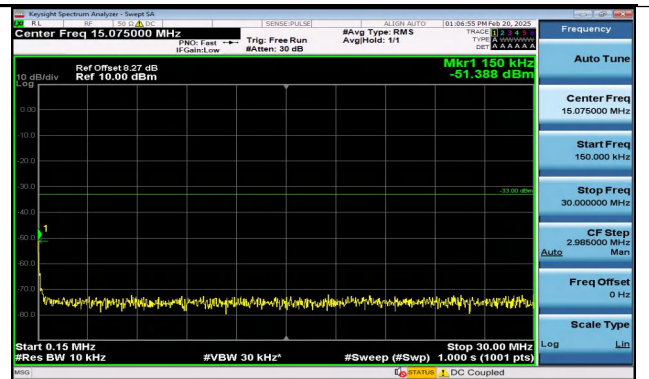
Band2_10MHz_QPSK_18650_50RB#0_0.15~30_0.15~30
