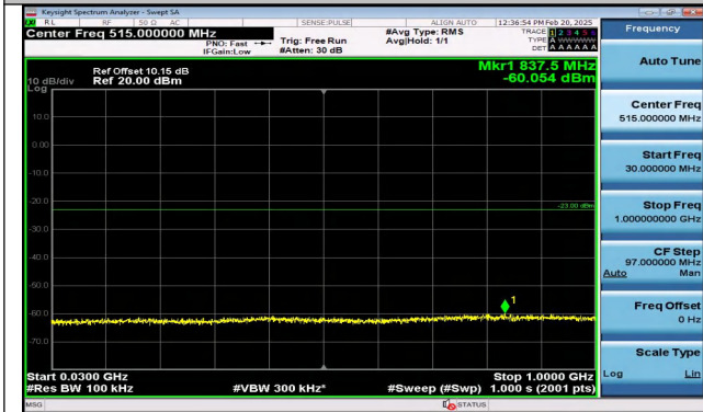
Band2_5MHz_QPSK_19175_1RB#0_30~1000_30~1000
