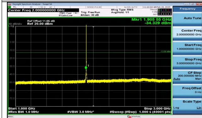
Band2_1.4MHz_16QAM_19193_1RB#0_1000~3000_1000~3000
