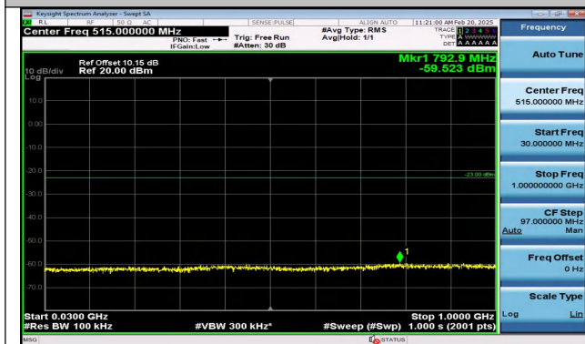
Band2_1.4MHz_QPSK_19193_1RB#0_30~1000_30~1000
