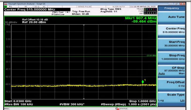
Band2_1.4MHz_16QAM_18900_1RB#0_30~1000_30~10 00
