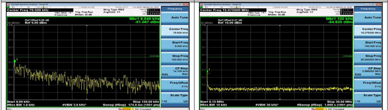
Band2_1.4MHz_QPSK_19193_6RB#0_0.009~0.15_0.009 ~0.15
