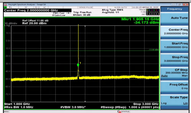
Band2_1.4MHz_QPSK_19193_1RB#0_1000~3000_1000~
