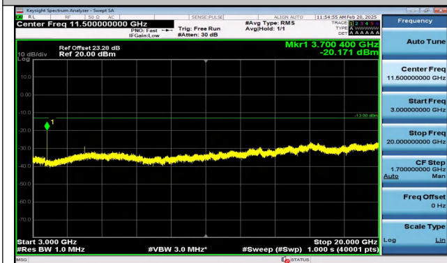
Band2_3MHz_QPSK_18615_1RB#0_3000~20000_3000~20000 20000
