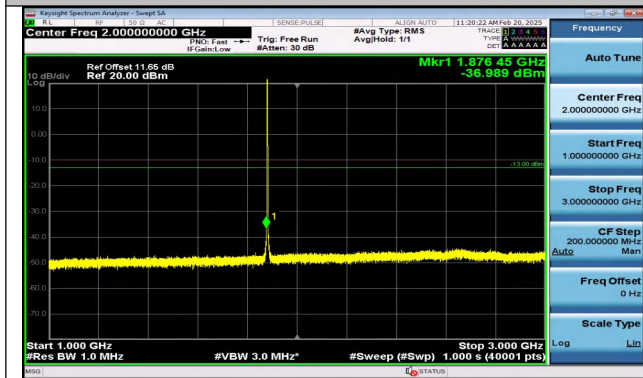
Band2_1.4MHz_16QAM_18900_6RB#0_1000~3000_1000
