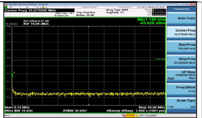
Band2_1.4MHz_QPSK_18900_6RB#0_0.15~30_0.15~30
