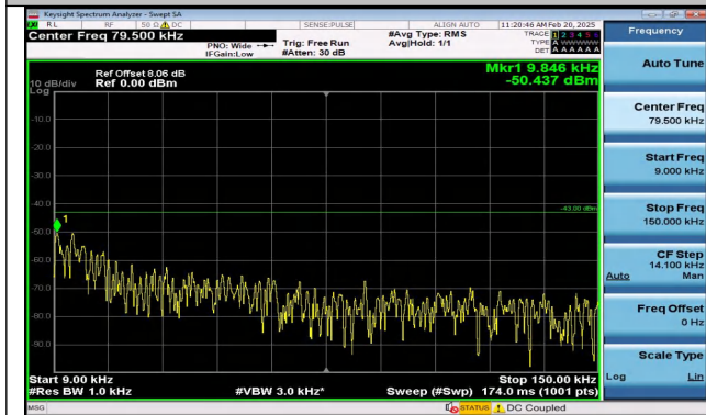
Band2_1.4MHz_QPSK_19193_1RB#0_0.009~0.15_0.009
