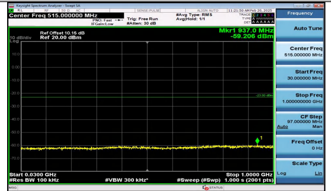
Band2_1.4MHz_16QAM_19193_1RB#0_30~1000_30~1000
