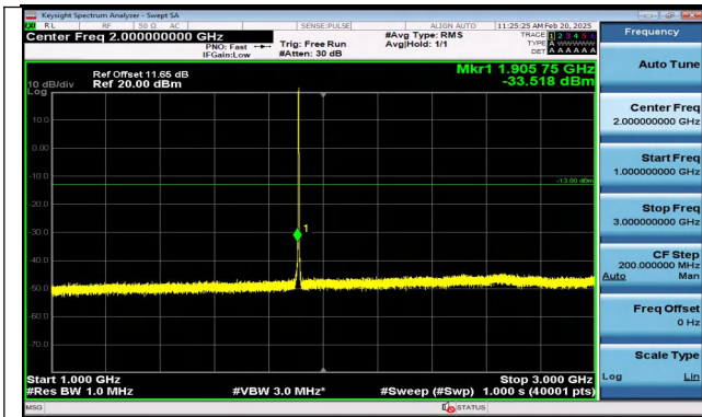
Band2_1.4MHz_16QAM_19193_6RB#0_1000~3000_1000 ~3000
