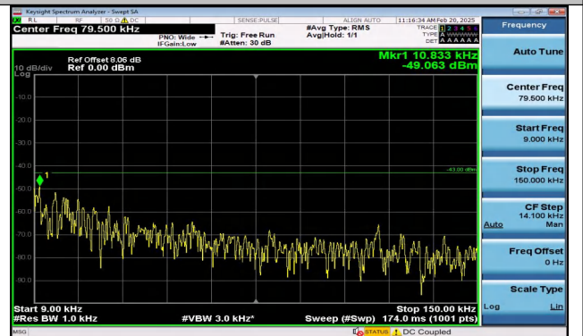
Band2_1.4MHz_16QAM_18900_1RB#0_0.009~0.15_0.00 9~0.15
