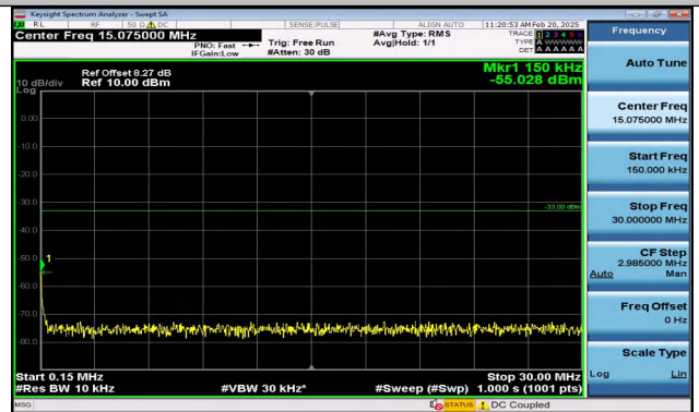
Band2_1.4MHz_QPSK_19193_1RB#0_0.15~30_0.15~30
