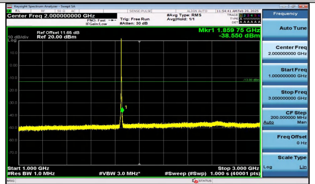
Band2_3MHz_QPSK_18615_1RB#0_1000~3000_1000~3000 000
