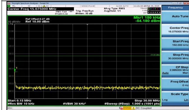
Band2_1.4MHz_16QAM_19193_1RB#0_0.15~30_0.15~30
