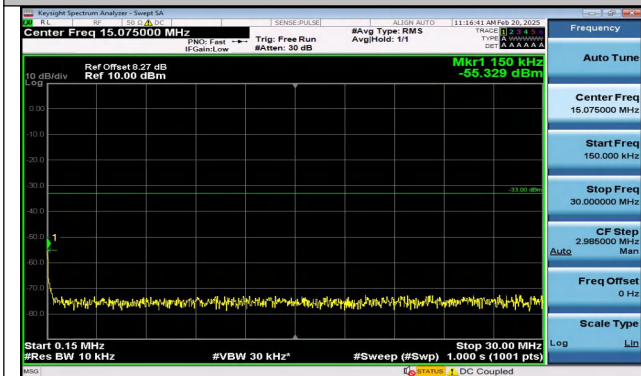
Band2_1.4MHz_16QAM_18900_1RB#0_0.15~30_0.15~30 0
