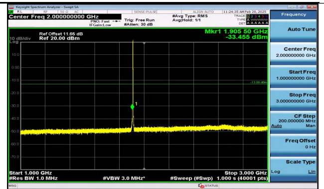
Band2_1.4MHz_QPSK_19193_6RB#0_1000~3000_1000~3000
