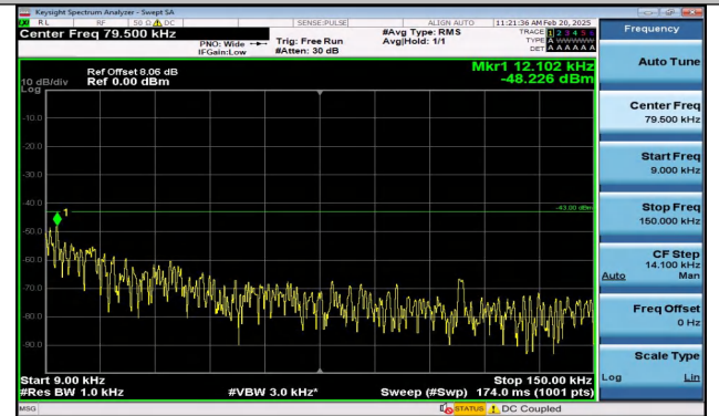
Band2_1.4MHz_16QAM_19193_1RB#0_0.009~0.15_0.009~0.15
