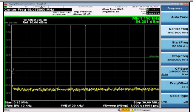
Band2_3MHz_QPSK_18615_1RB#0_0.15~30_0.15~30
