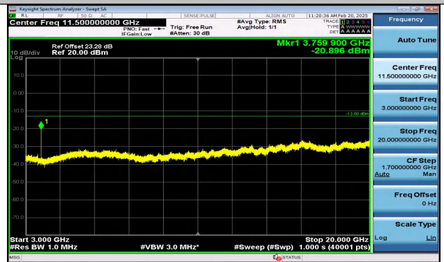
Band2_1.4MHz_16QAM_18900_6RB#0_3000~20000_300
