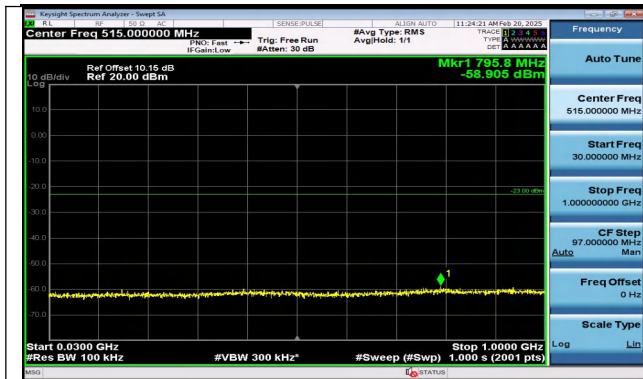
Band2_1.4MHz_QPSK_19193_6RB#0_30~1000_30~1000
