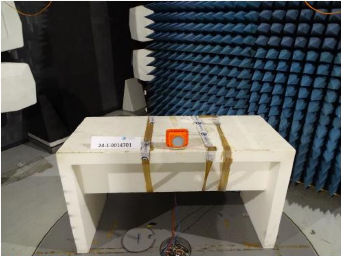
Picture 1 : Radiated Emission - Setup close up view
