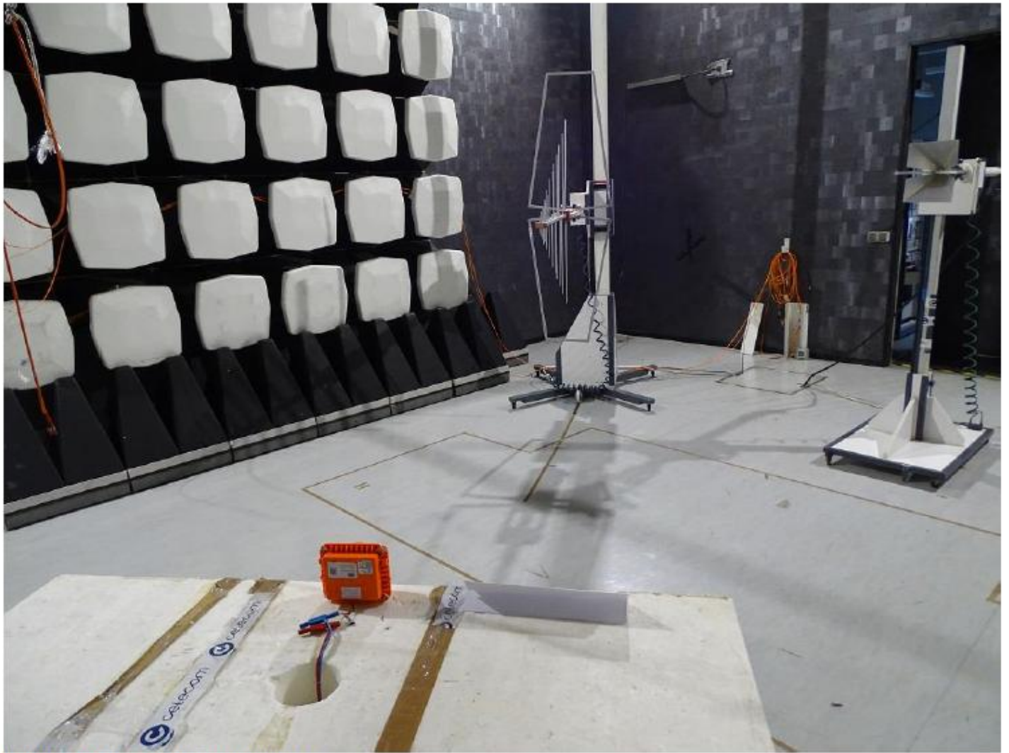
Picture 3 : Radiated Emission - Setup rear side
