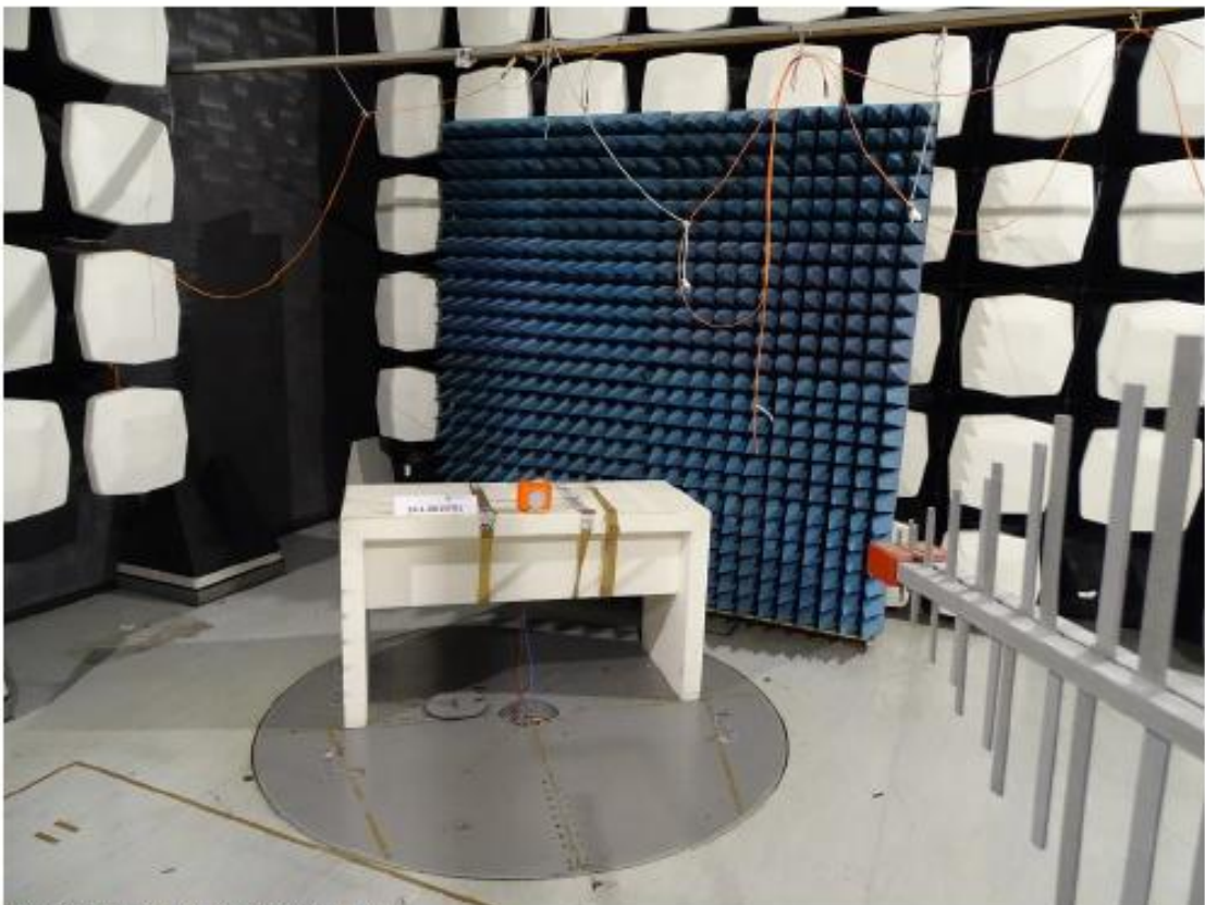
Picture 2 : Radiated Emission - Setup overall view
