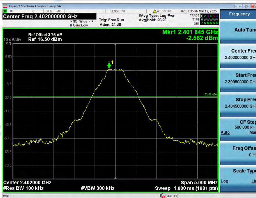
1_Reference_Level_NVNT_ANT1_1-DH5_2402_00
