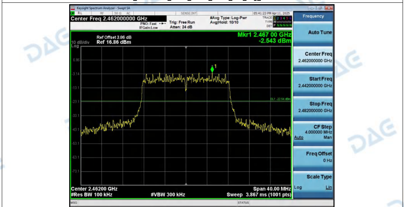
2_Spurious_Emission_NVNT_ANT1_802_11g_2462
