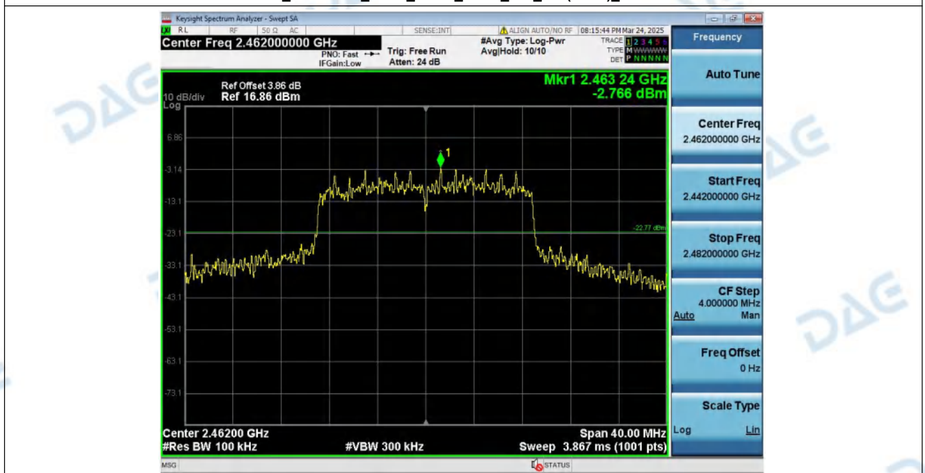
2_Spurious_Emission_NVNT_ANT1_802_11n(HT20)_2462
