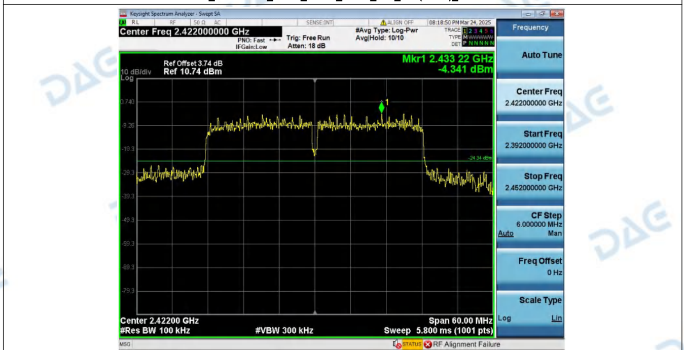
2_Spurious_Emission_NVNT_ANT1_802_11n(HT40)_2422
