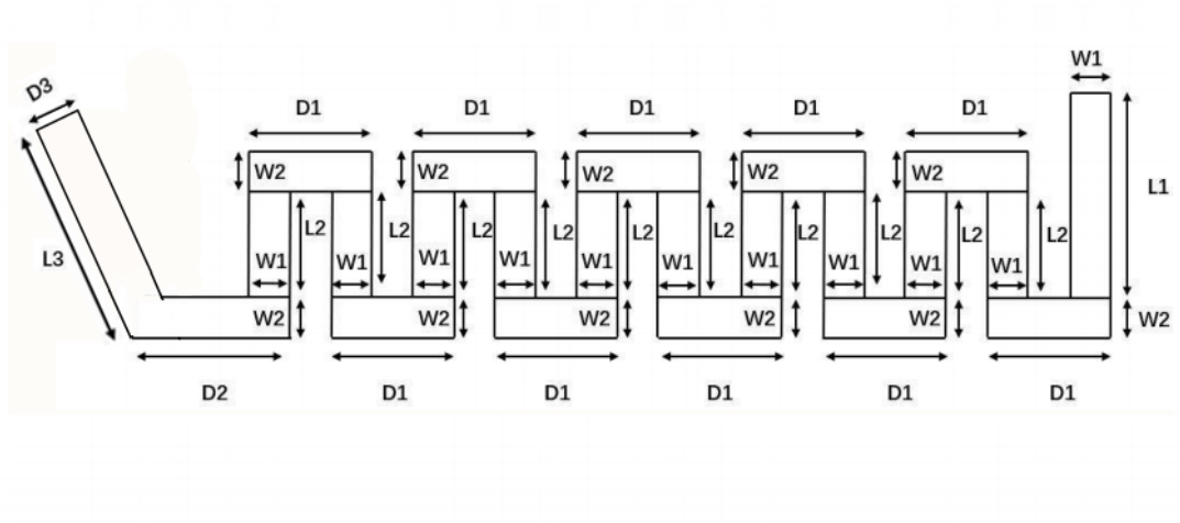
Antenna Dimensions
