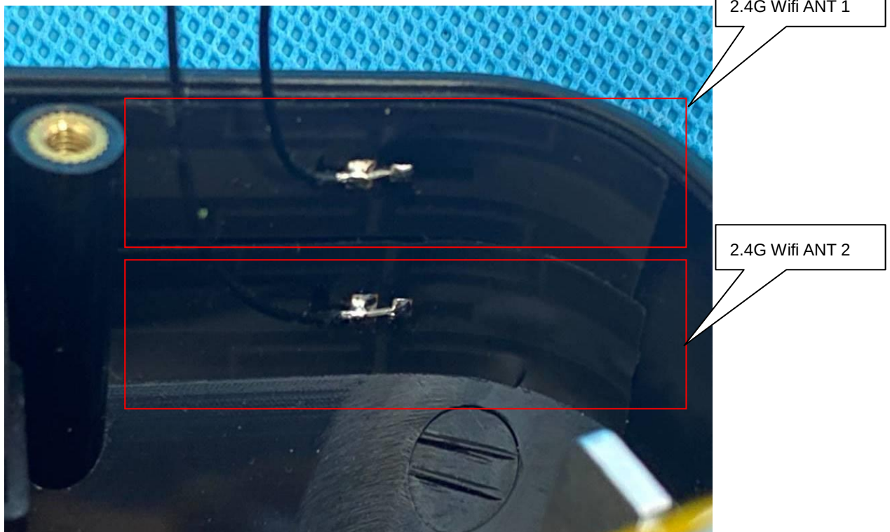
INTERNAL VIEW OF EUT (FIGURE 1)
