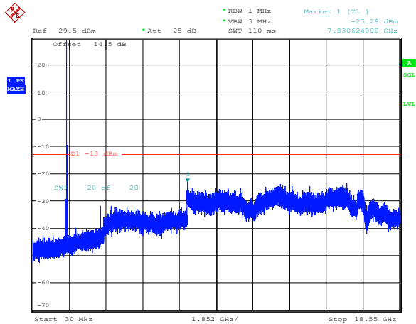
20MHz_Middle_16QAM_1@0(30MHz~18.55GHz)
