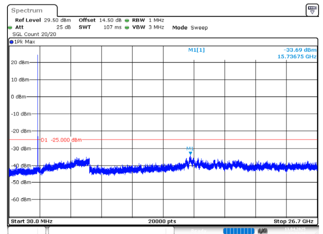
10MHz_Low_16QAM_1@0(30MHz~26.7GHz)
