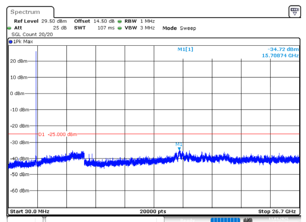
5MHz_High_QPSK_1@0(30MHz~26.7GHz)
