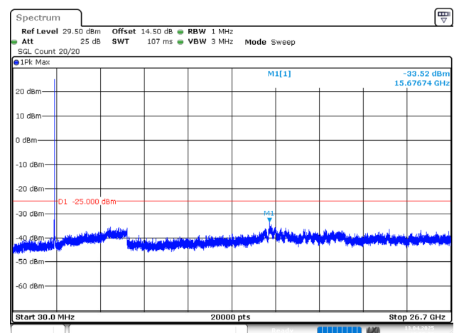
10MHz_High_16QAM_1@0(30MHz~26.7GHz)
