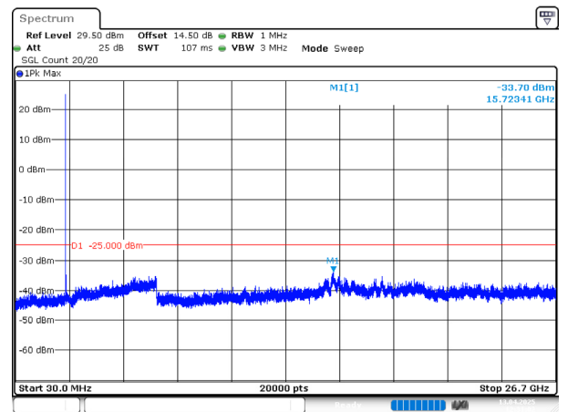
5MHz_Low_QPSK_1@0(30MHz~26.7GHz)
