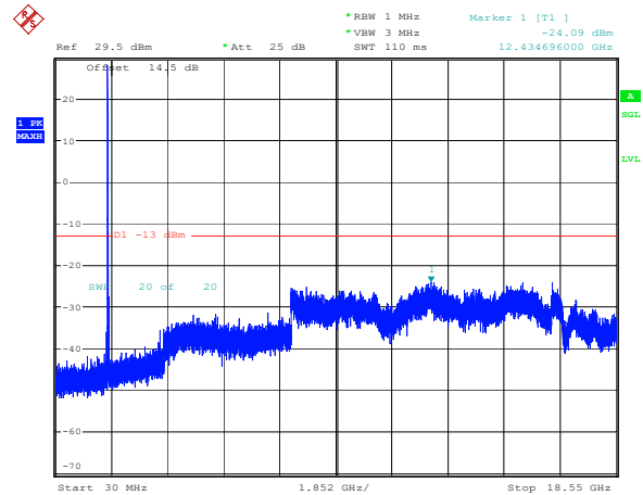
20MHz_High_QPSK_1@0(30MHz~18.55GHz)
