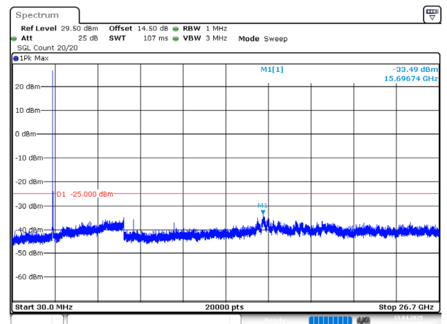
10MHz_Middle_16QAM_1@0(30MHz~26.7GHz)
