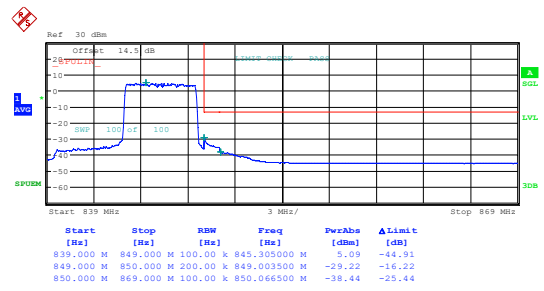
10MHz_High_16QAM_25@25
