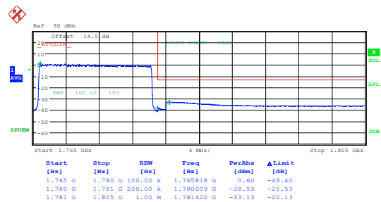
15MHz_High_QPSK_75@0
