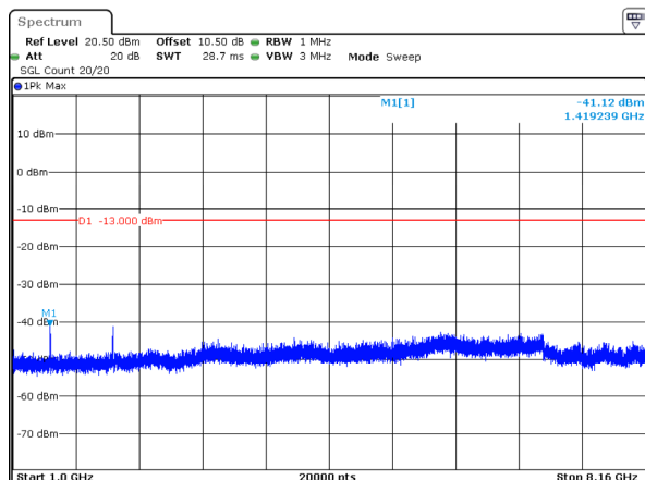
5MHz_Middle_QPSK_25@0(1GHz~8.16GHz)
