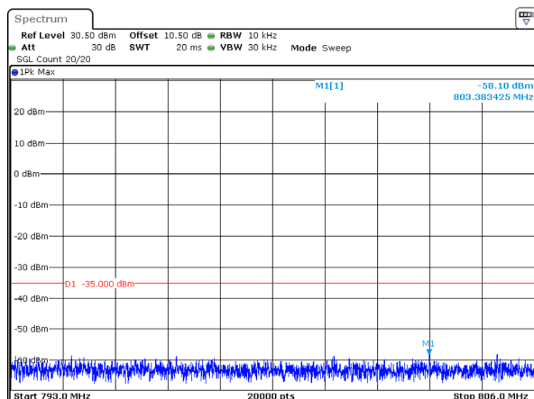
5MHz_Low_QPSK_1@0(793MHz~806MHz)
