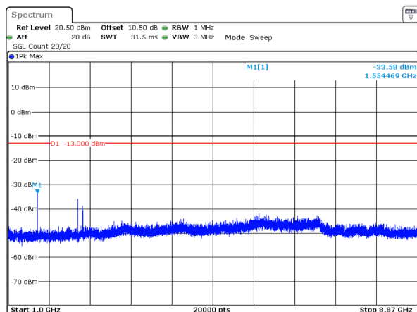
5MHz_Low_QPSK_1@0(1GHz~8.87GHz)
