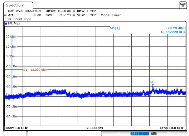
1.4MHz_Low_QPSK_1@0(1GHz~18.8GHz)
