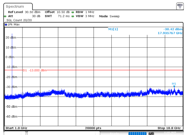
1.4MHz_Middle_QPSK_1@0(1GHz~18.8GHz)
