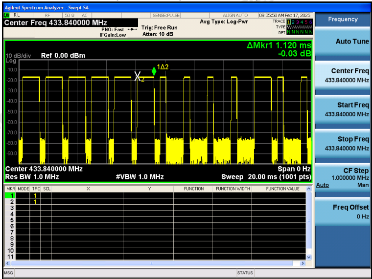
(Time per burst: 1.120ms*17pcs)
