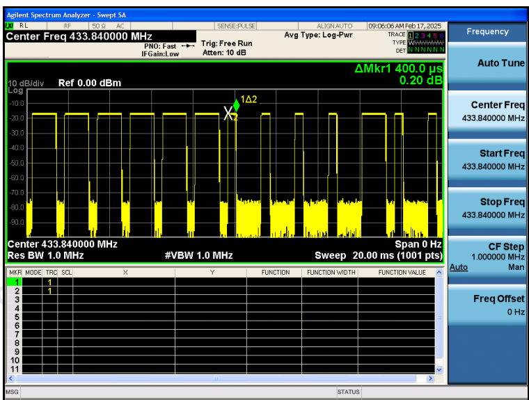
(Time per burst: 0.40 ms*8pcs)
