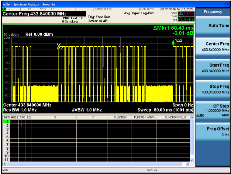
(Transmit cycle 50.40ms)
