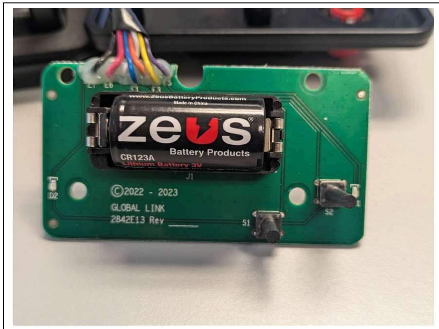
Battery Board Front
