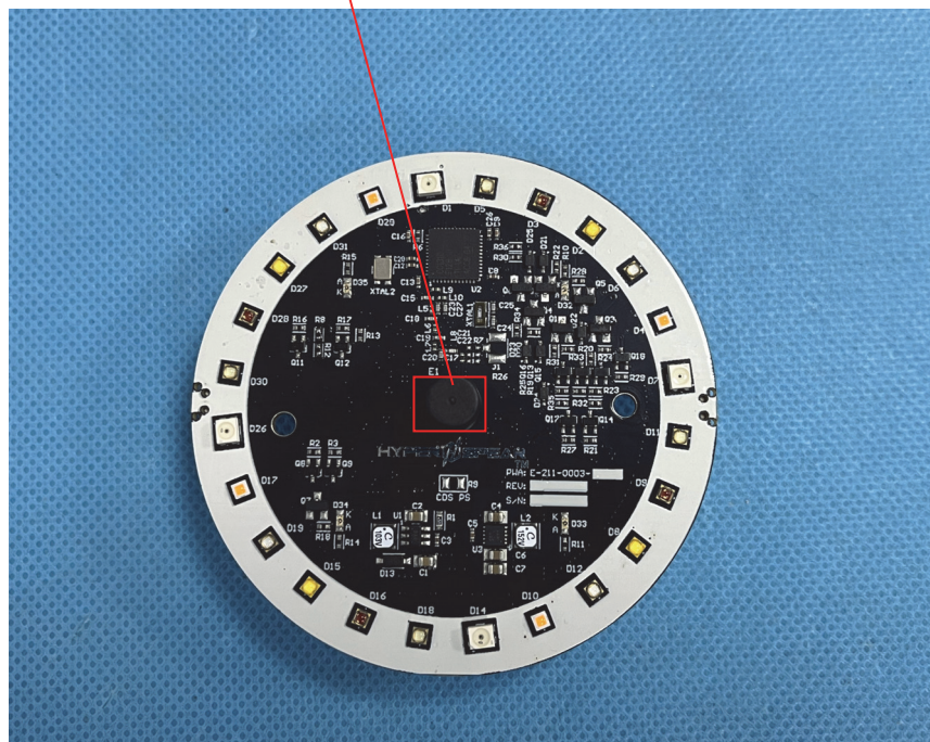
916MHz Transmit Antenna
