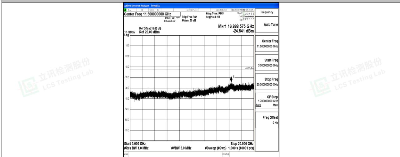
Band66_20MHz_QPSK_132572_1RB#0_3000~20000_3000~20000
