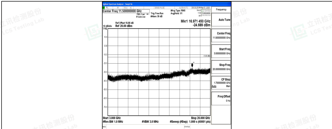
Band66_20MHz_16QAM_132322_1RB#0_3000~20000_3000~20000
