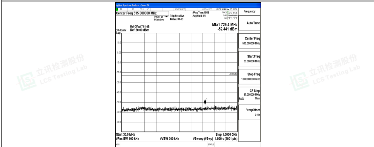
Band66_20MHz_QPSK_132322_1RB#0_30~1000_30~1000
