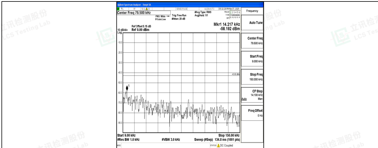
Band66_20MHz_QPSK_132322_1RB#0_0.009~0.15_0.009~0.15
