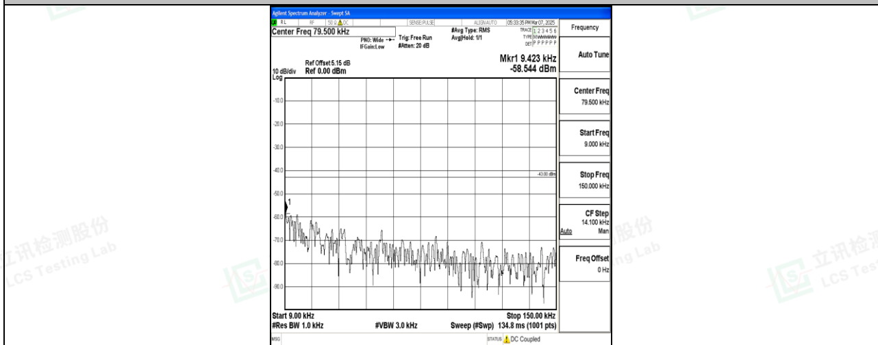
Band66_20MHz_QPSK_132572_1RB#0_0.009~0.15_0.009~0.15
