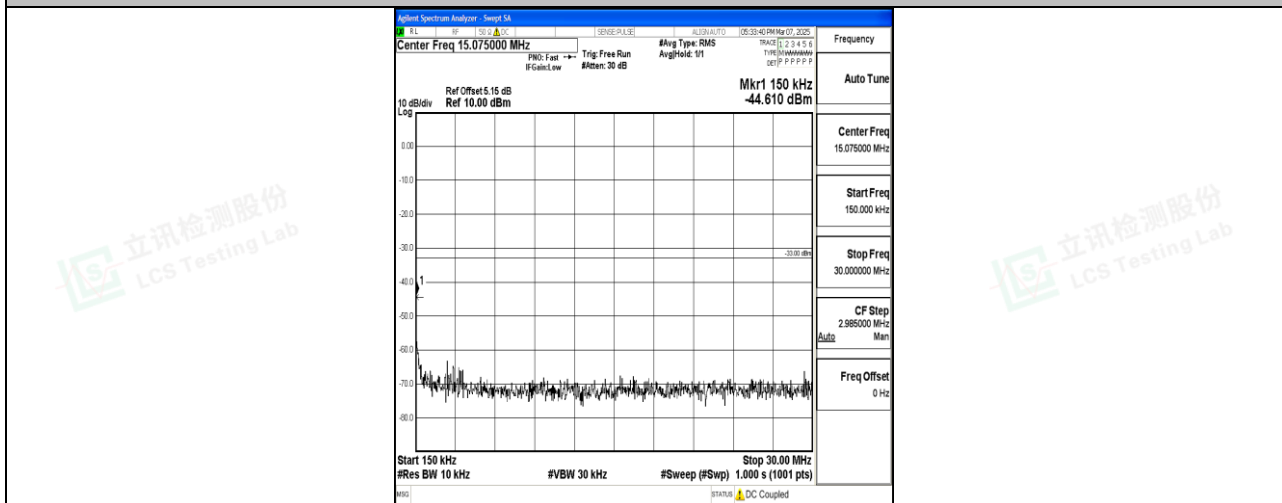
Band66_20MHz_QPSK_132572_1RB#0_0.15~30_0.15~30
