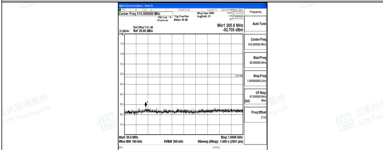
Band66_5MHz_16QAM_132322_1RB#0_30~1000_30~1000
