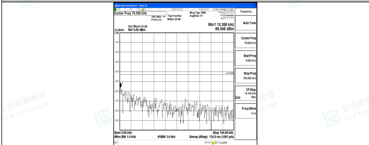
Band66_5MHz_QPSK_132647_1RB#0_0.009~0.15_0.009~0.15
