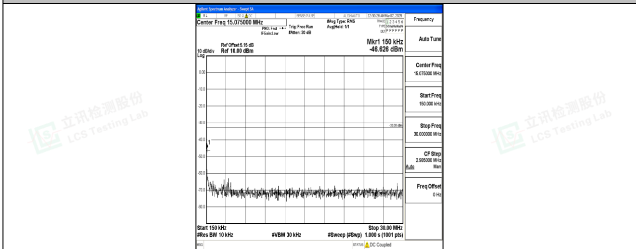
Band66_5MHz_16QAM_131997_1RB#0_0.15~30_0.15~30
