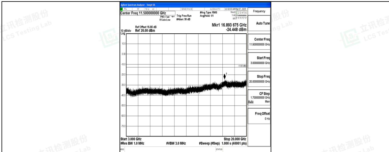
Band66_5MHz_16QAM_132322_1RB#0_3000~20000_3000~20000
