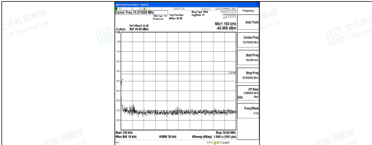
Band66_10MHz_16QAM_132322_1RB#0_0.15~30_0.15~30
