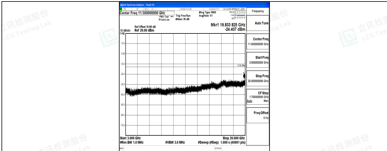
Band66_15MHz_16QAM_132322_1RB#0_3000~20000_3000~20000
