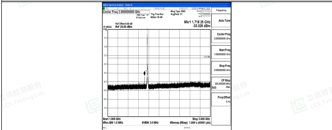
Band66_10MHz_QPSK_132622_1RB#0_1000~3000_1000~3000
