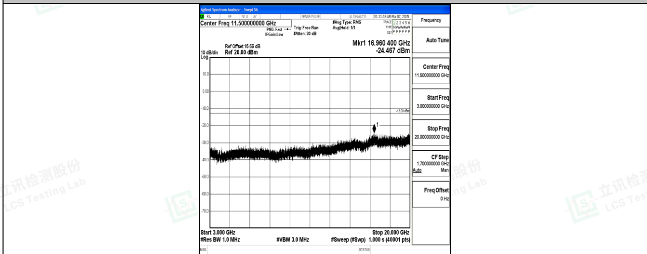
Band66_15MHz_16QAM_132597_1RB#0_3000~20000_3000~20000
