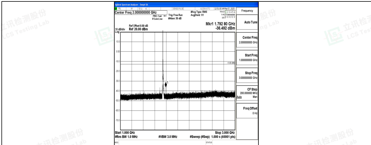
Band66_10MHz_QPSK_132322_1RB#0_1000~3000_1000~3000
