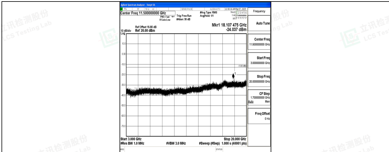
Band66_5MHz_QPSK_131997_1RB#0_3000~20000_3000~20000
