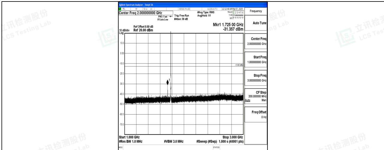
Band66_3MHz_16QAM_132657_1RB#0_1000~3000_1000~3000
