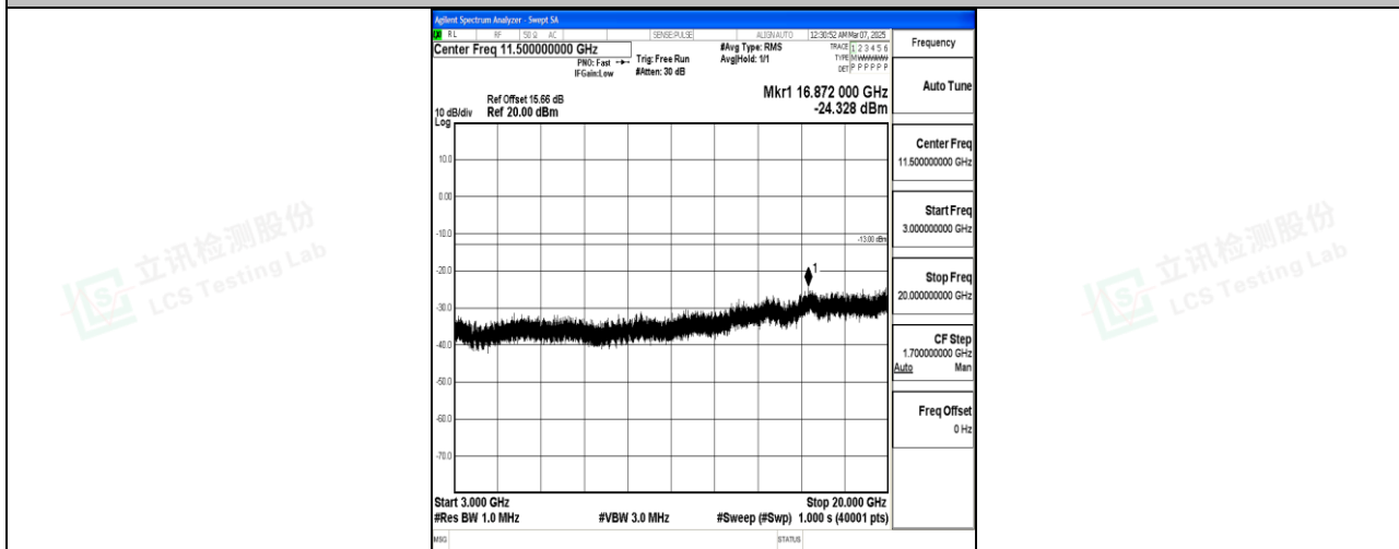
Band66_5MHz_16QAM_131997_1RB#0_3000~20000_3000~20000
