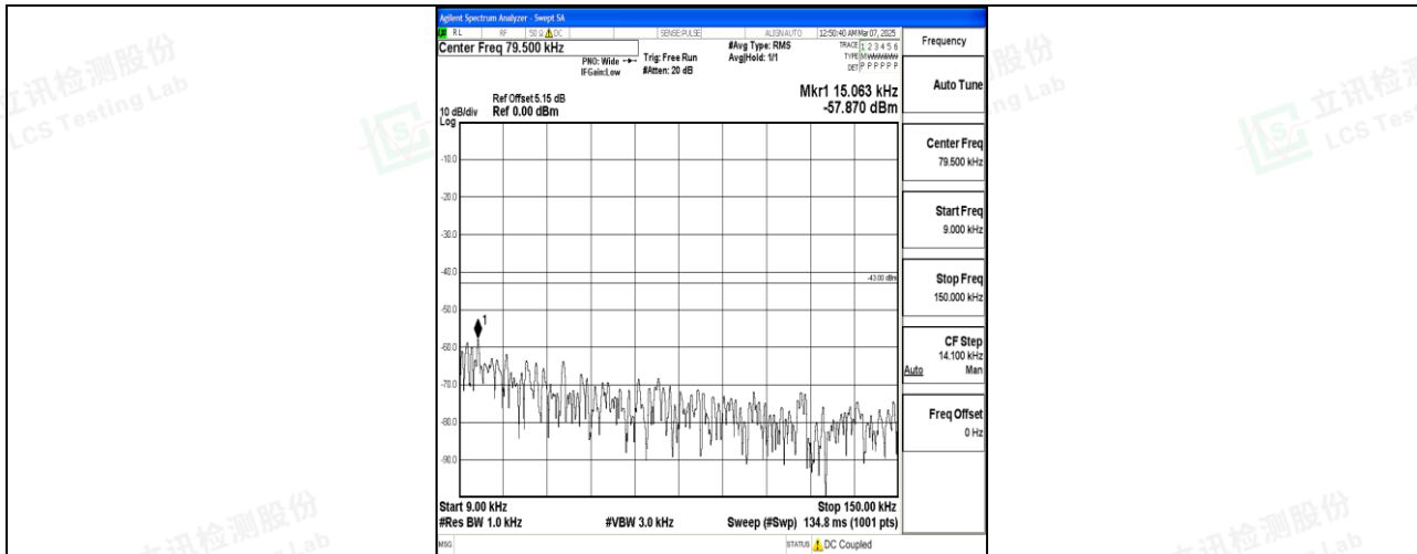
Band66_10MHz_QPSK_132322_1RB#0_0.009~0.15_0.009~0.15
