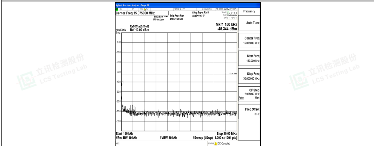
Band66_10MHz_16QAM_132022_1RB#0_0.15~30_0.15~30
