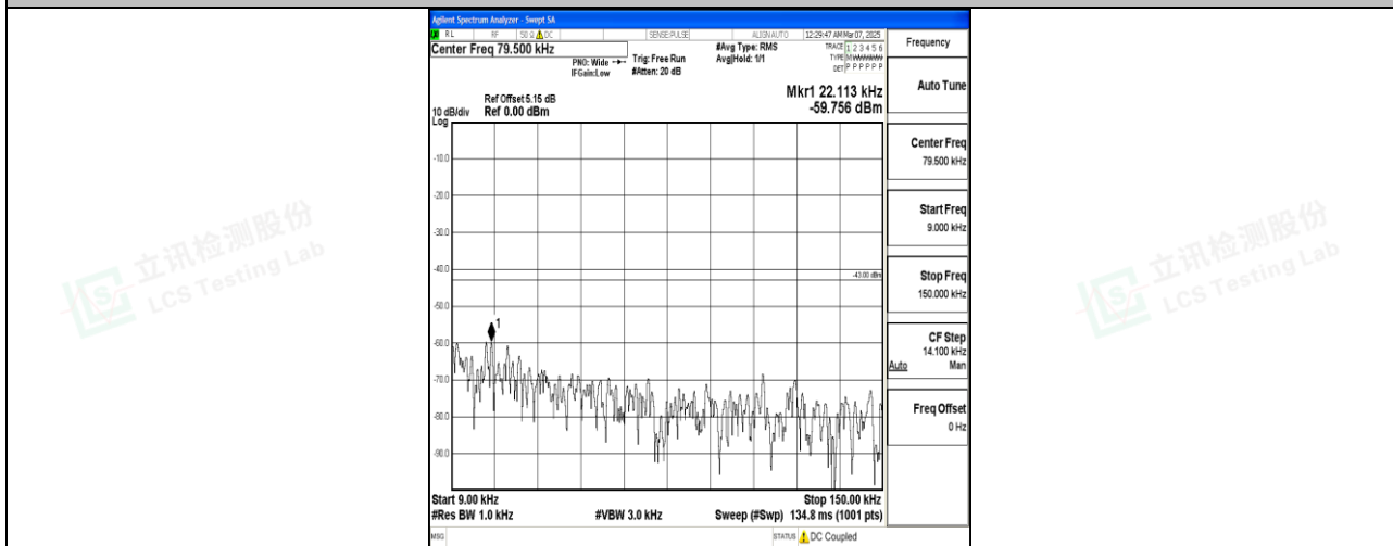
Band66_5MHz_QPSK_131997_1RB#0_0.009~0.15_0.009~0.15
