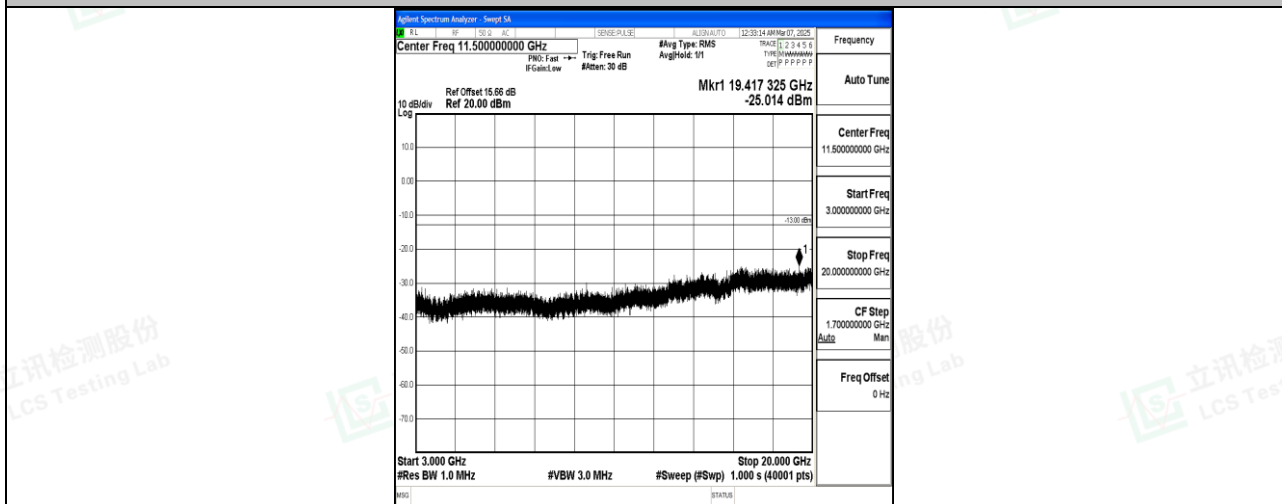
Band66_5MHz_16QAM_132647_1RB#0_3000~20000_3000~20000
