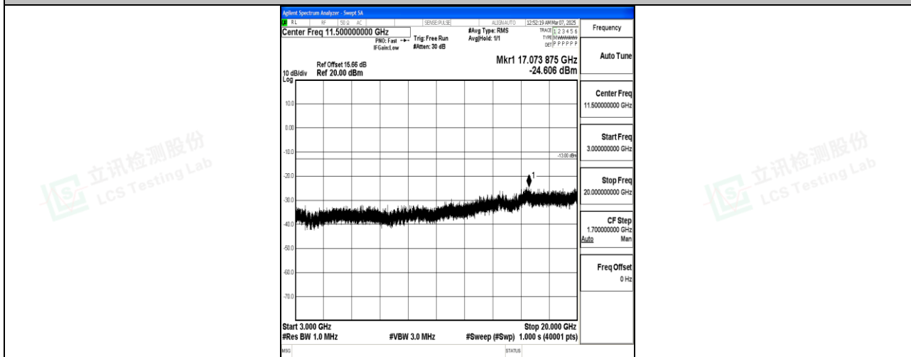
Band66_10MHz_QPSK_132622_1RB#0_3000~20000_3000~20000
