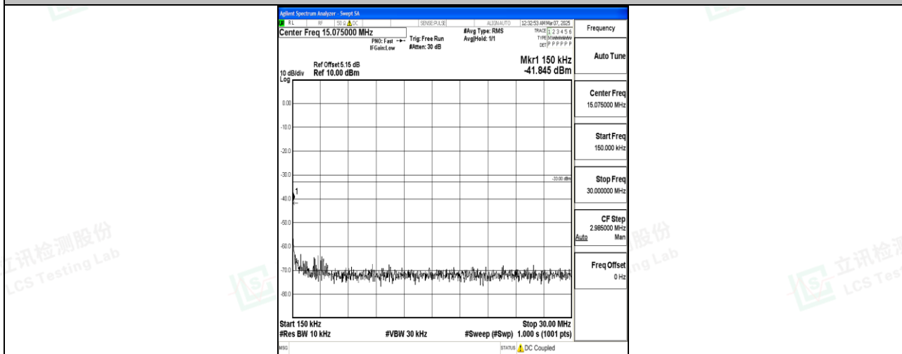
Band66_5MHz_16QAM_132647_1RB#0_0.15~30_0.15~30
