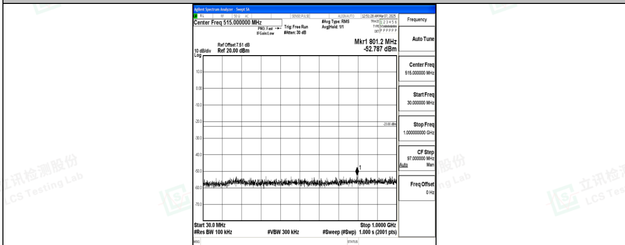
Band66_10MHz_16QAM_132322_1RB#0_30~1000_30~1000
