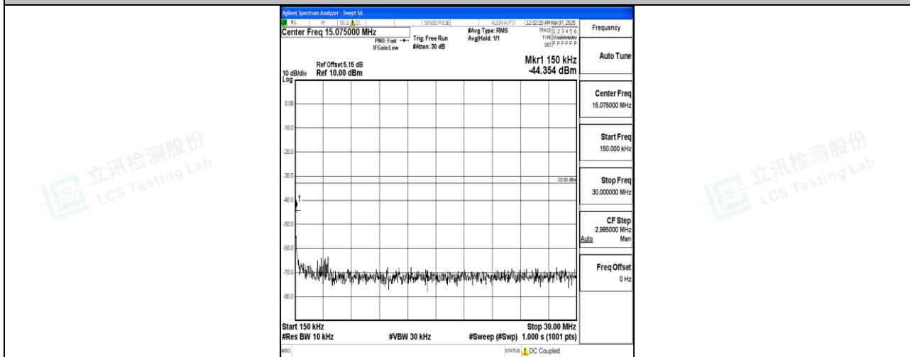
Band66_5MHz_QPSK_132647_1RB#0_0.15~30_0.15~30
