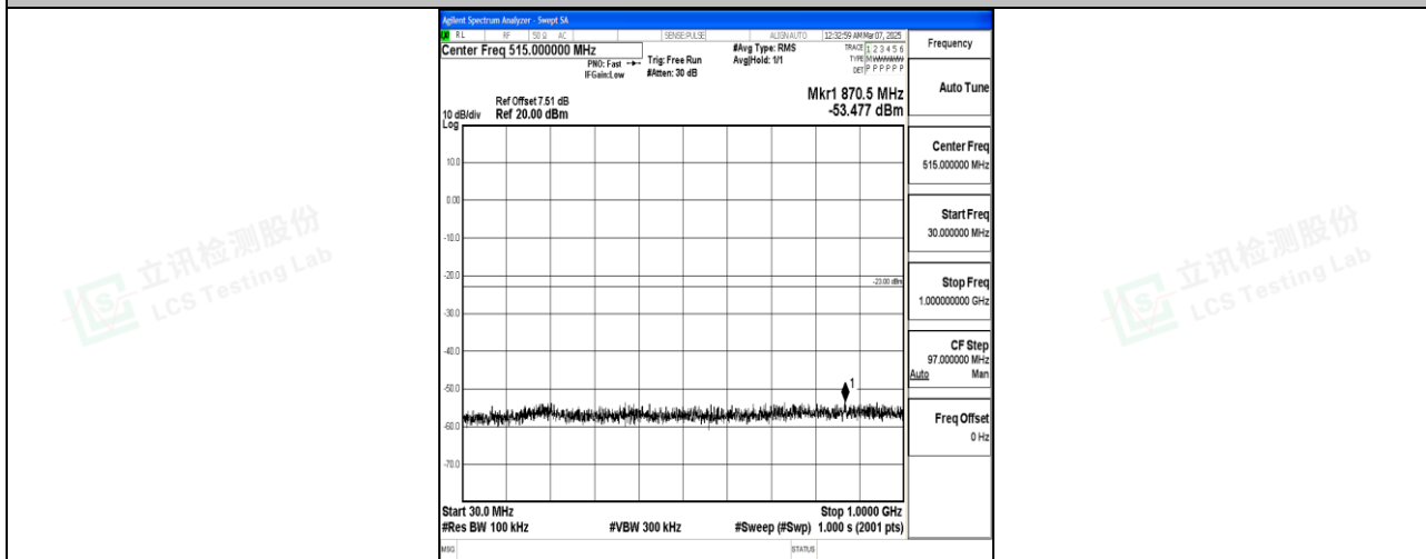
Band66_5MHz_16QAM_132647_1RB#0_30~1000_30~1000
