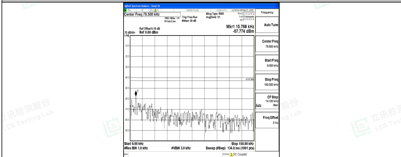
Band66_10MHz_16QAM_132022_1RB#0_0.009~0.15_0.009~0.15
