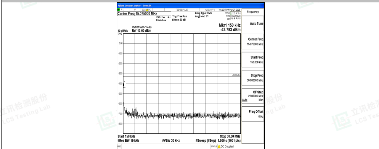
Band66_15MHz_16QAM_132597_1RB#0_0.15~30_0.15~30
