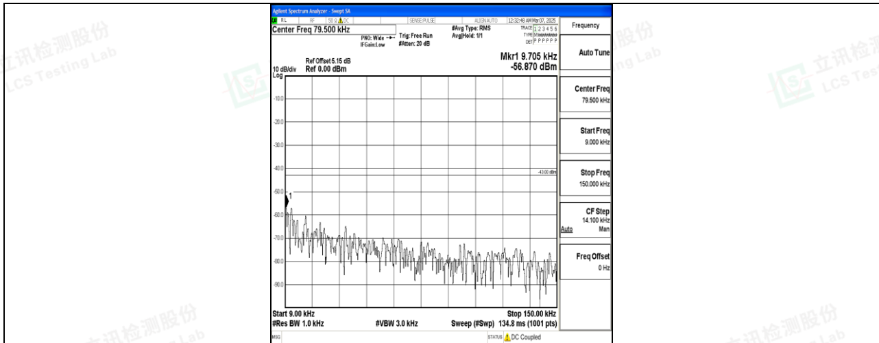
Band66_5MHz_16QAM_132647_1RB#0_0.009~0.15_0.009~0.15
