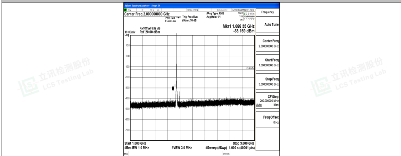
Band66_10MHz_16QAM_132322_1RB#0_1000~3000_1000~3000
