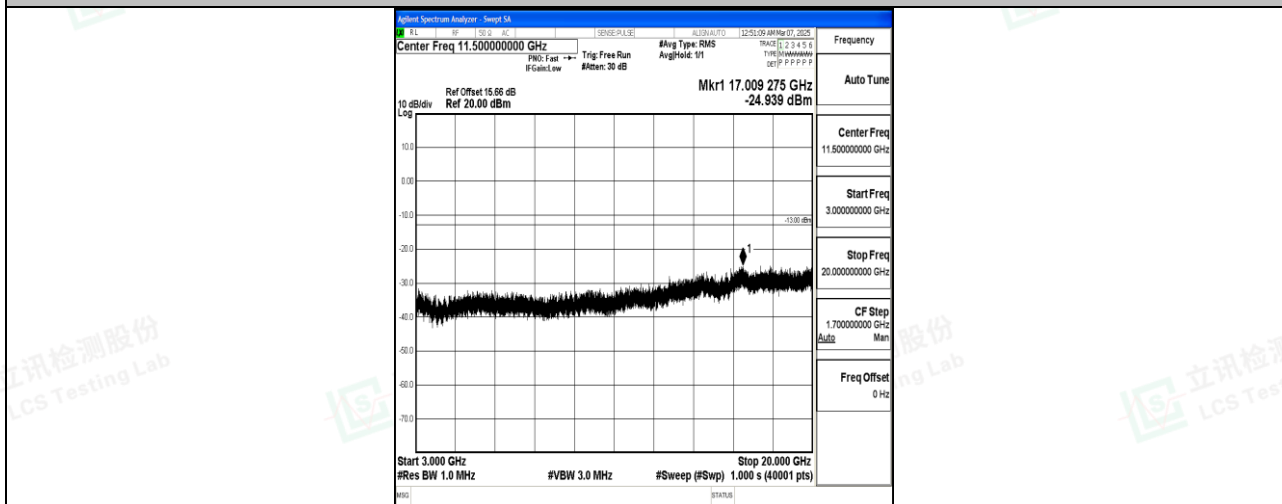
Band66_10MHz_QPSK_132322_1RB#0_3000~20000_3000~20000
