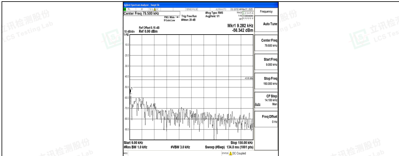
Band66_15MHz_16QAM_132597_1RB#0_0.009~0.15_0.009~0.15
