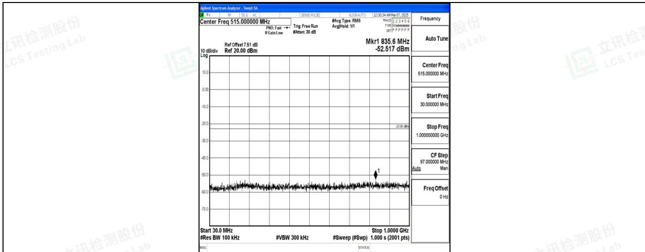
Band66_5MHz_16QAM_131997_1RB#0_30~1000_30~1000
