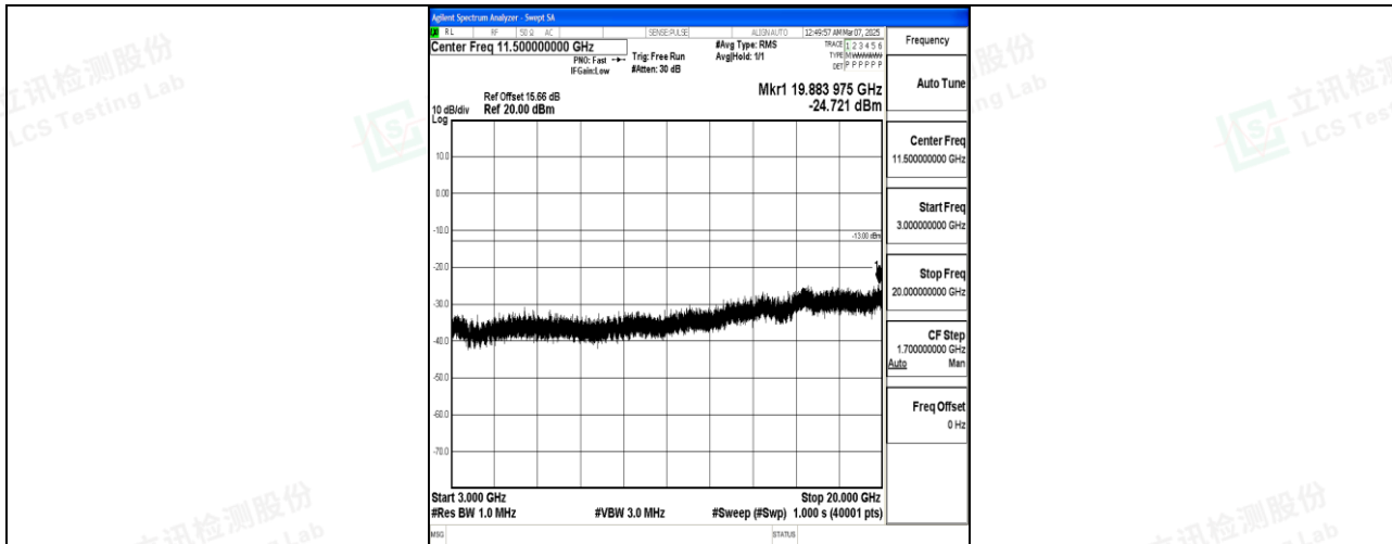
Band66_10MHz_QPSK_132022_1RB#0_3000~20000_3000~20000
