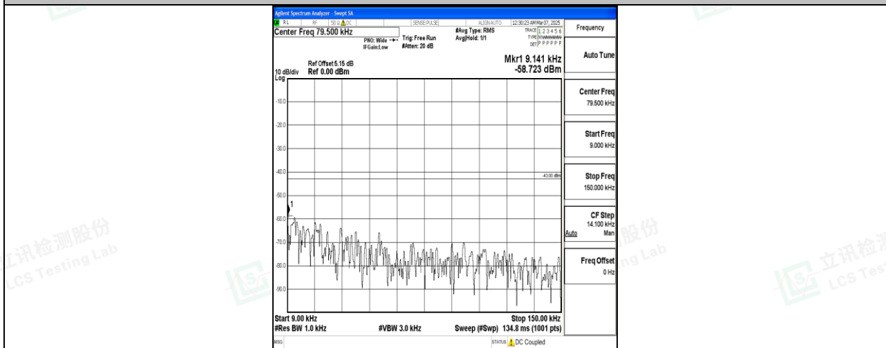
Band66_5MHz_16QAM_131997_1RB#0_0.009~0.15_0.009~0.15
