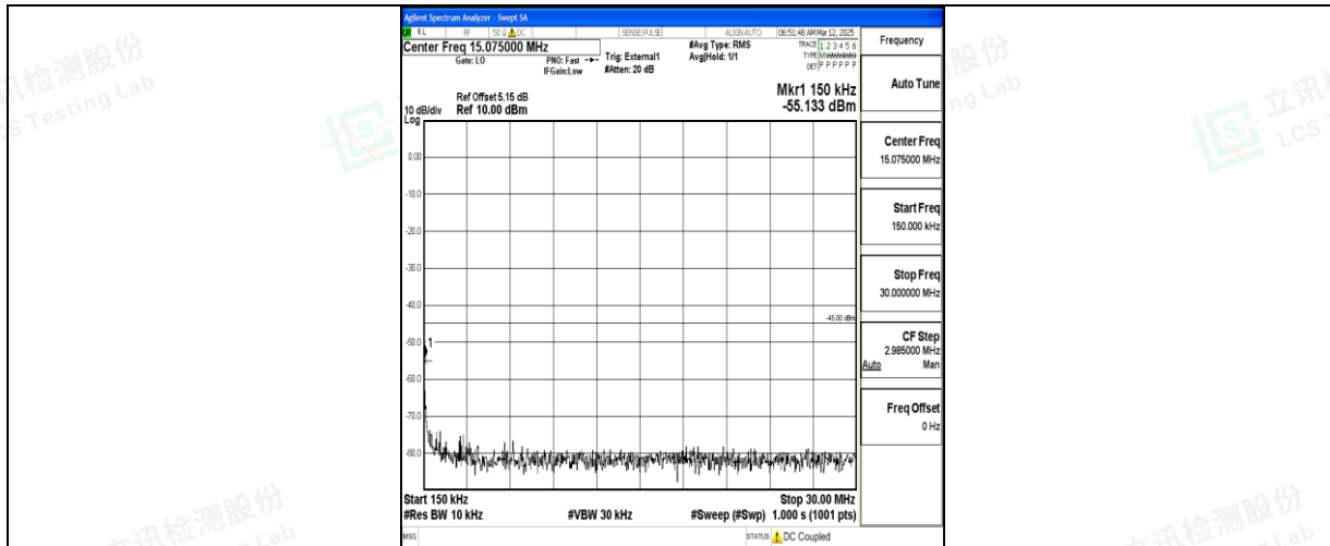
Band41_15MHz_QPSK_41515_1RB#0_0.15~30_0.15~30
