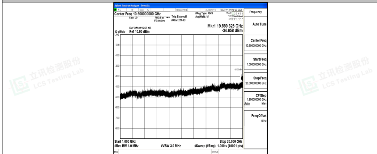
Band41_5MHz_QPSK_41565_1RB#0_1000~20000_1000~20000
