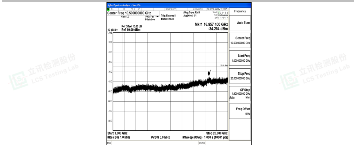
Band41_15MHz_QPSK_41515_1RB#0_1000~20000_1000~20000
