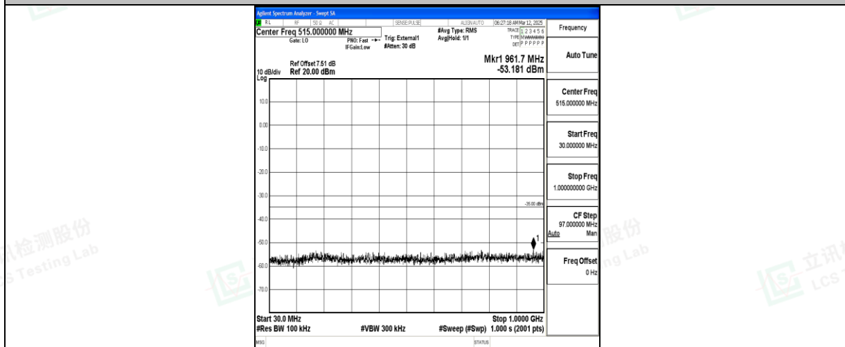
Band41_5MHz_QPSK_41565_1RB#0_30~1000_30~1000
