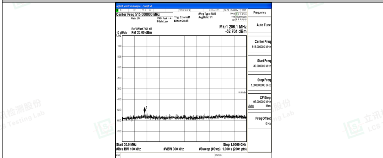
Band41_15MHz_QPSK_41515_1RB#0_30~1000_30~1000
