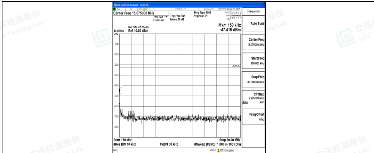
Band26_15MHz_QPSK_26965_1RB#0_0.15~30_0.15~30
