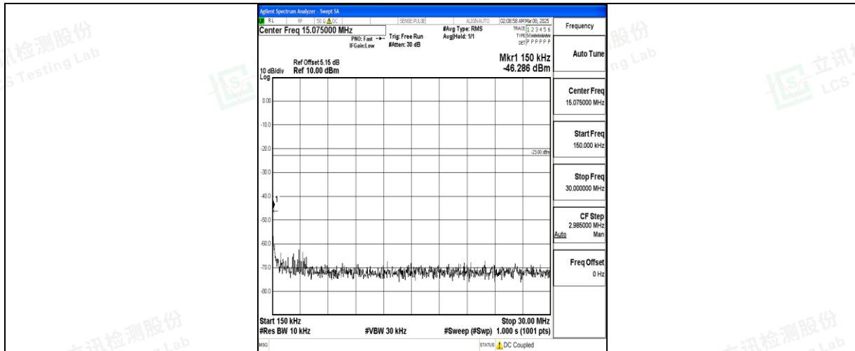
Band26_10MHz_QPSK_26990_1RB#0_0.15~30_0.15~30
