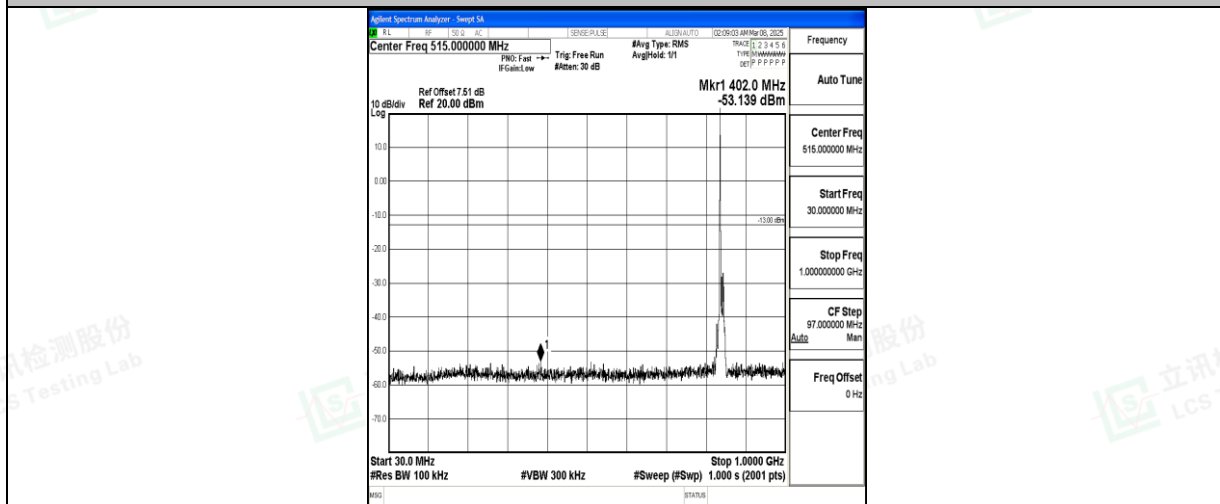
Band26_10MHz_QPSK_26990_1RB#0_30~1000_30~1000
