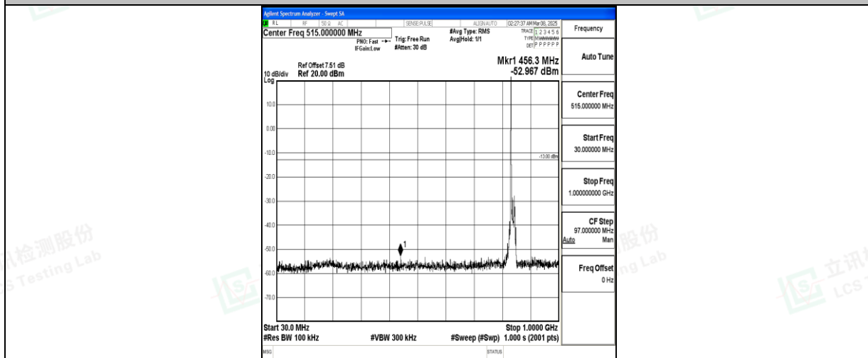
Band26_15MHz_QPSK_26965_1RB#0_30~1000_30~1000
