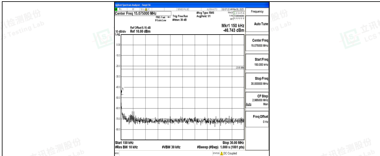
Band26_10MHz_16QAM_26840_1RB#0_0.15~30_0.15~30
