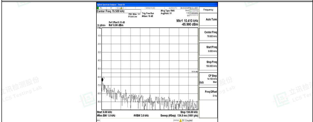
Band7_20MHz_QPSK_21350_1RB#0_0.009~0.15_0.009~0.15
