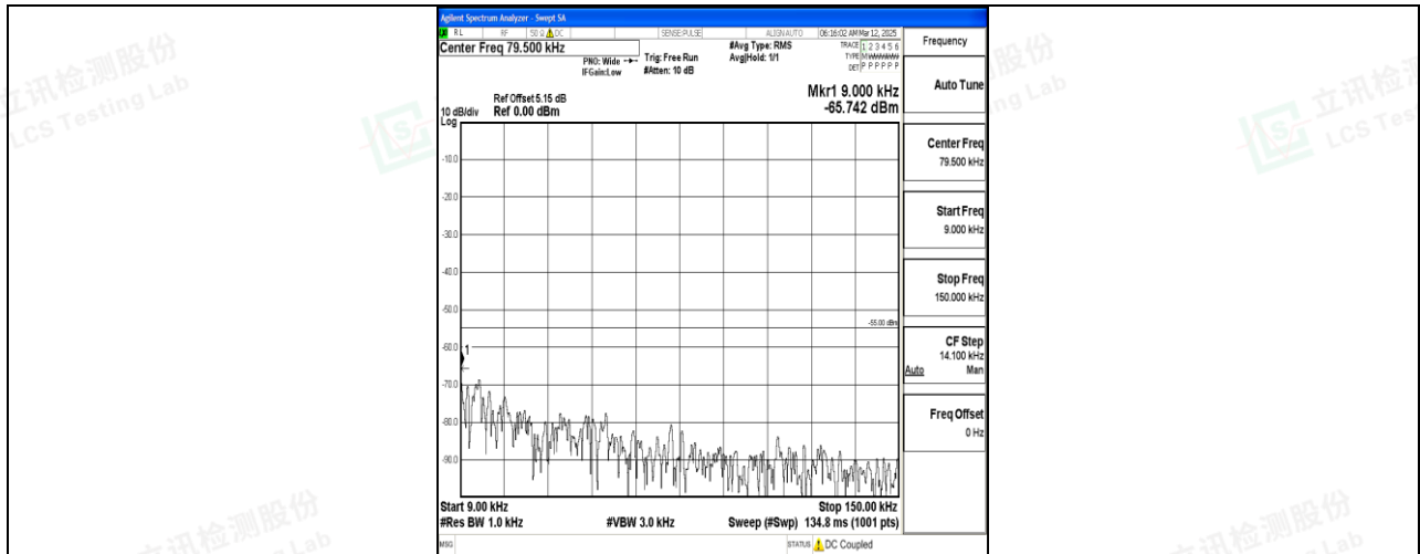
Band7_20MHz_16QAM_21350_1RB#0_0.009~0.15_0.009~0.15
