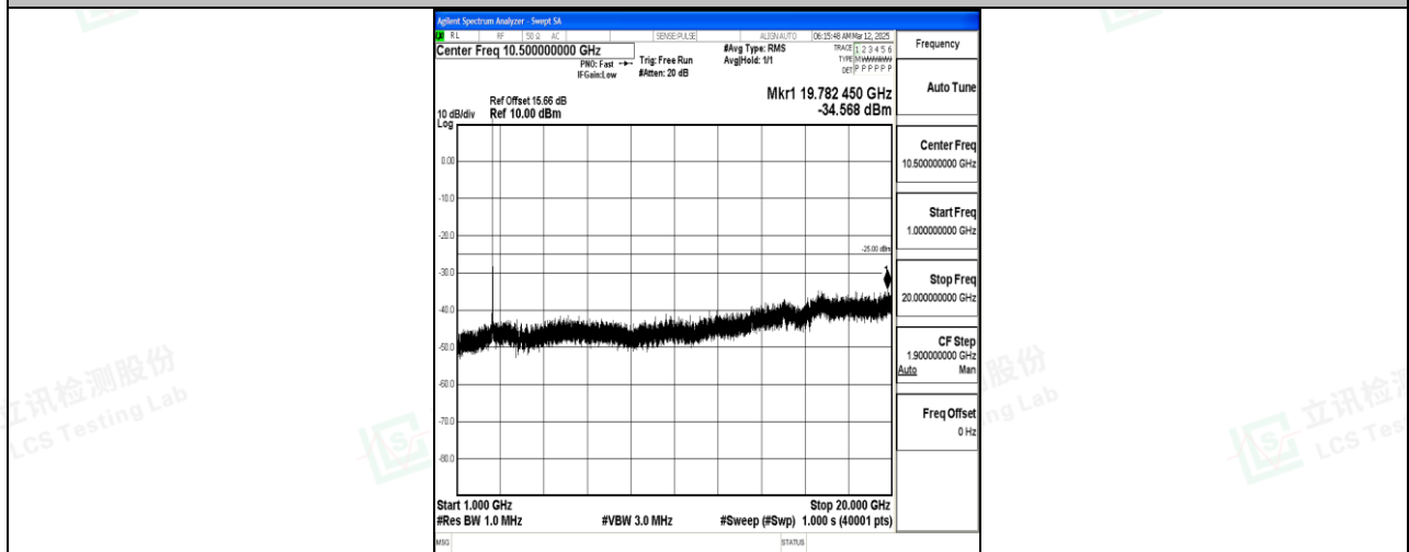
Band7_20MHz_QPSK_21350_1RB#0_1000~20000_1000~20000
