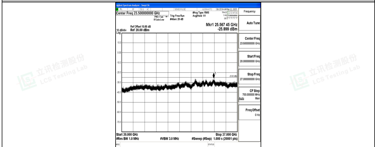
Band7_20MHz_QPSK_21350_1RB#0_20000~27000_20000~27000
