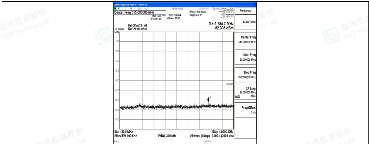
Band7_20MHz_QPSK_21350_1RB#0_30~1000_30~1000
