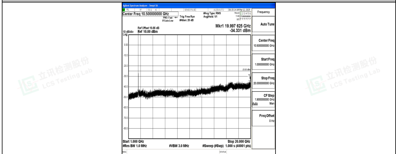
Band7_20MHz_16QAM_21100_1RB#0_1000~20000_1000~20000
