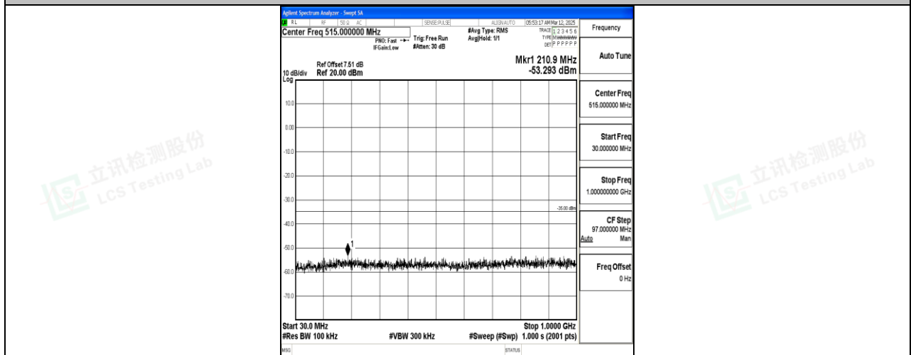
Band7_5MHz_16QAM_21425_1RB#0_30~1000_30~1000
