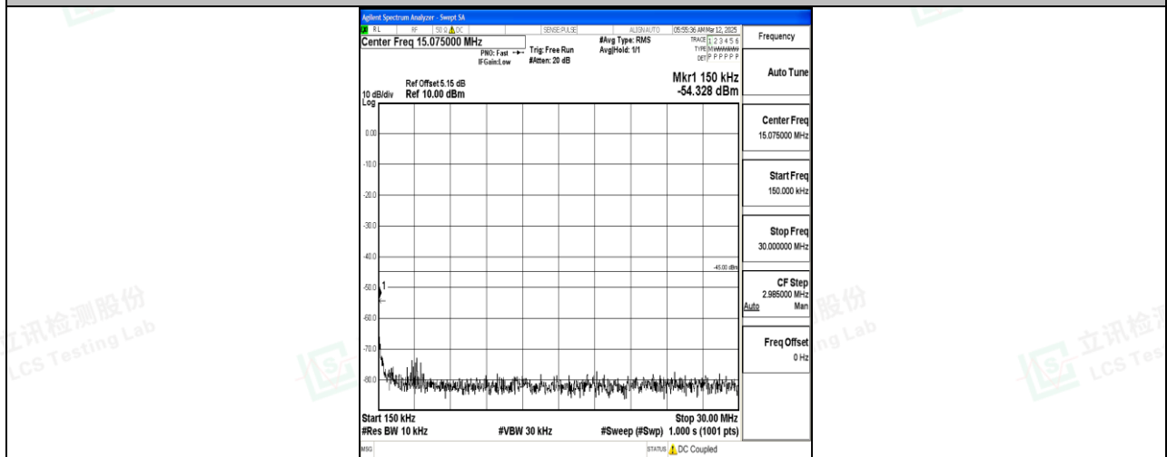
Band7_10MHz_QPSK_21100_1RB#0_0.15~30_0.15~30
