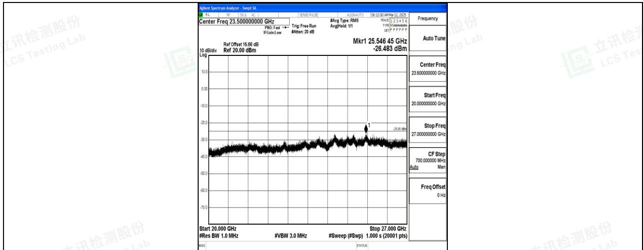
Band7_15MHz_16QAM_21100_1RB#0_20000~27000_20000~27000
