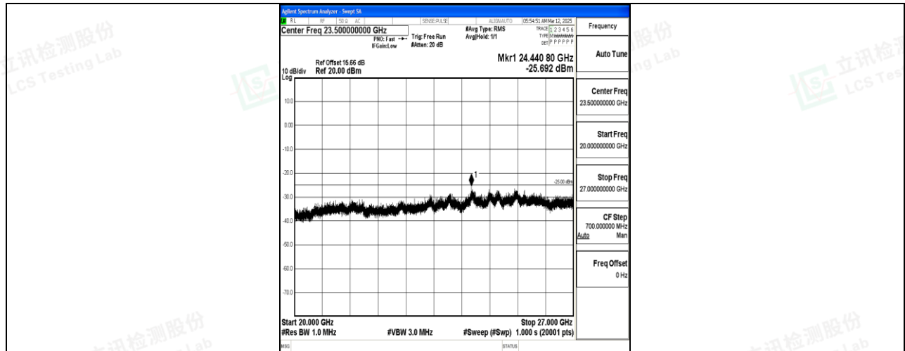
Band7_10MHz_QPSK_20800_1RB#0_20000~27000_20000~27000
