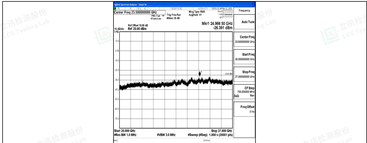
Band7_5MHz_16QAM_20775_1RB#0_20000~27000_20000~27000
