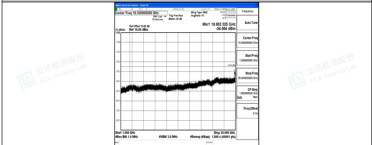
Band7_5MHz_16QAM_20775_1RB#0_1000~20000_1000~20000
