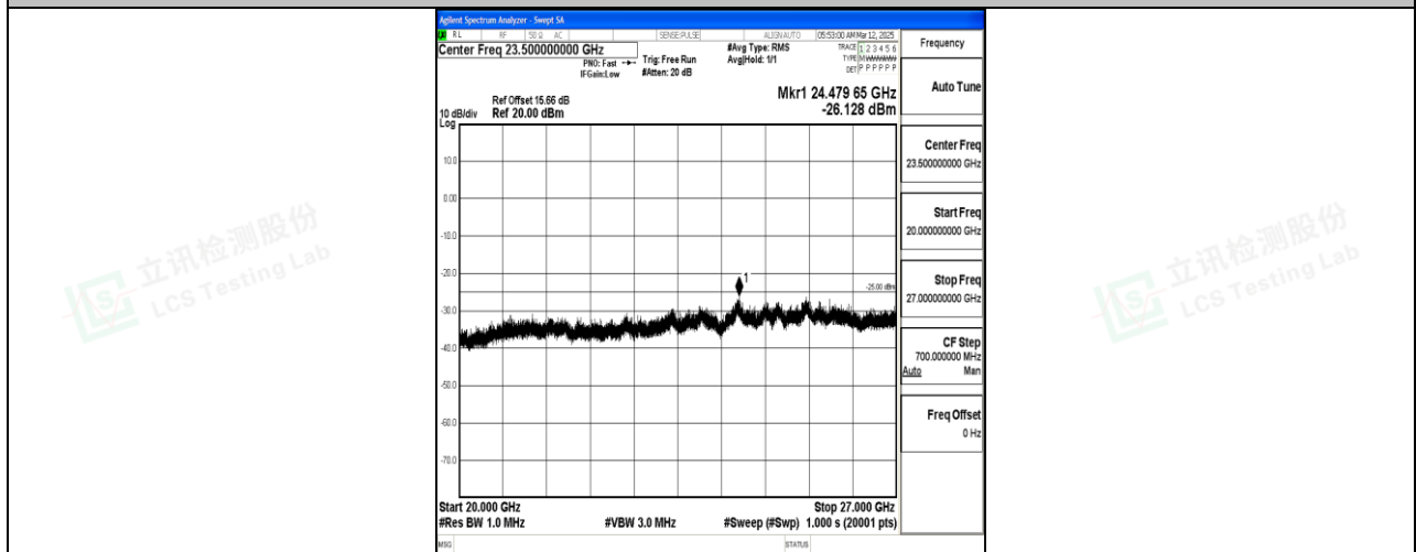
Band7_5MHz_QPSK_21425_1RB#0_20000~27000_20000~27000
