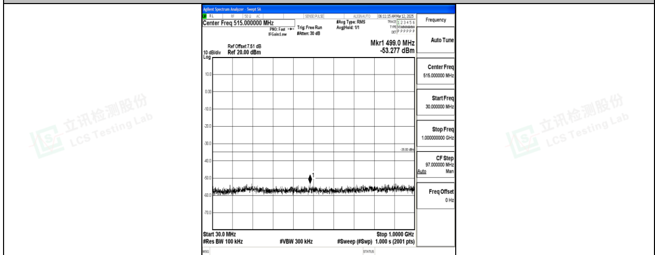
Band7_15MHz_QPSK_21100_1RB#0_30~1000_30~1000
