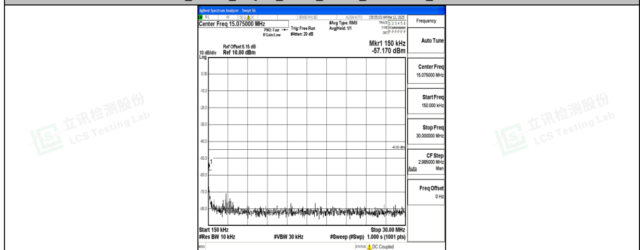
Band7_10MHz_16QAM_20800_1RB#0_0.15~30_0.15~30
