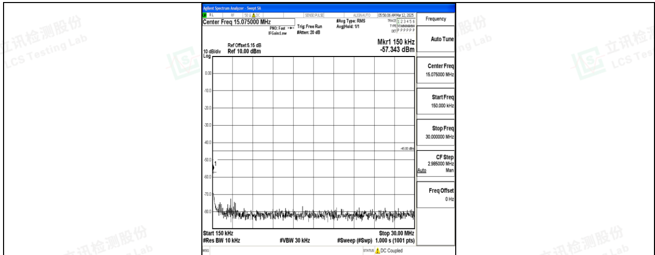
Band7_10MHz_16QAM_21100_1RB#0_0.15~30_0.15~30
