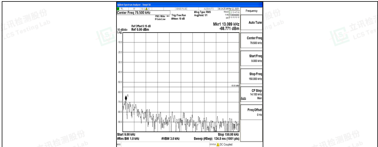
Band7_20MHz_QPSK_21100_1RB#0_0.009~0.15_0.009~0.15
