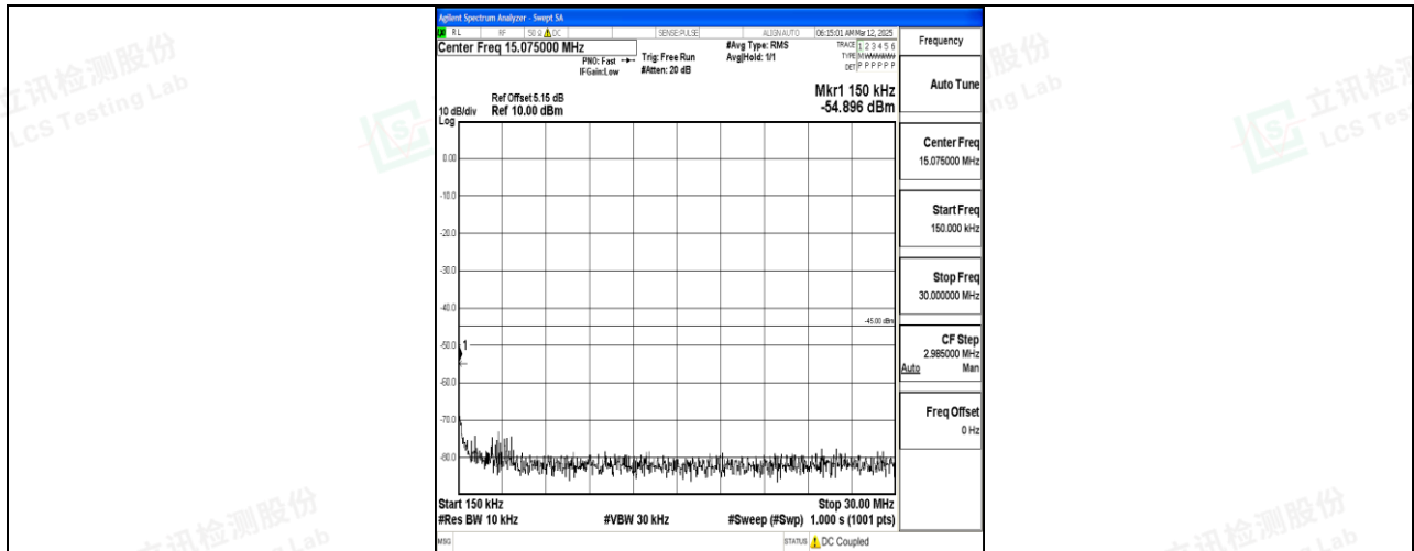
Band7_20MHz_16QAM_21100_1RB#0_0.15~30_0.15~30
