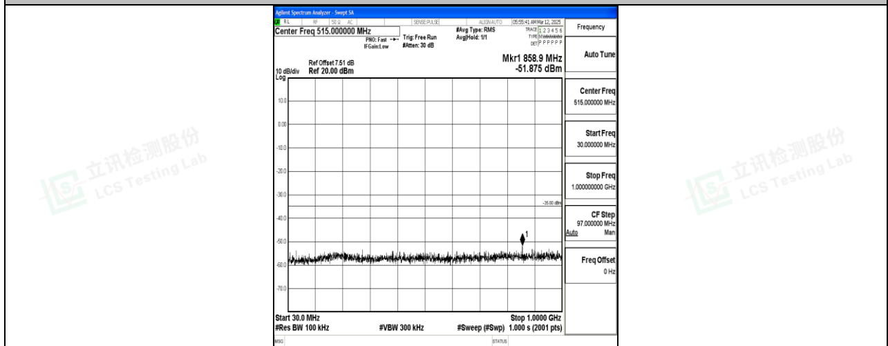
Band7_10MHz_QPSK_21100_1RB#0_30~1000_30~1000
