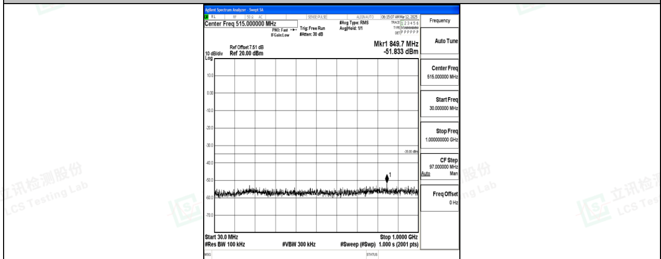
Band7_20MHz_16QAM_21100_1RB#0_30~1000_30~1000
