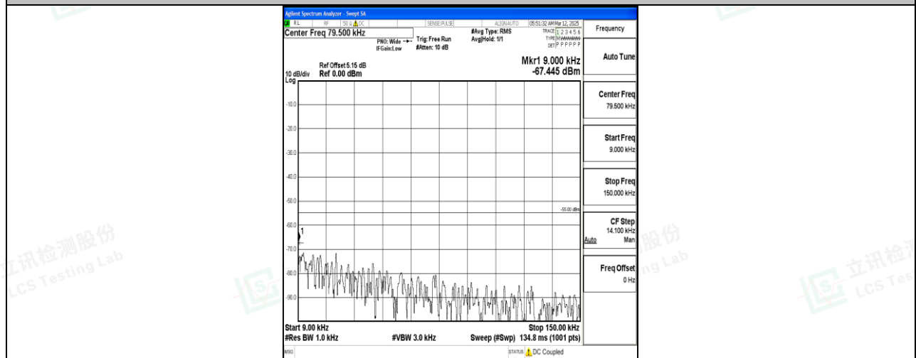
Band7_5MHz_QPSK_21100_1RB#0_0.009~0.15_0.009~0.15
