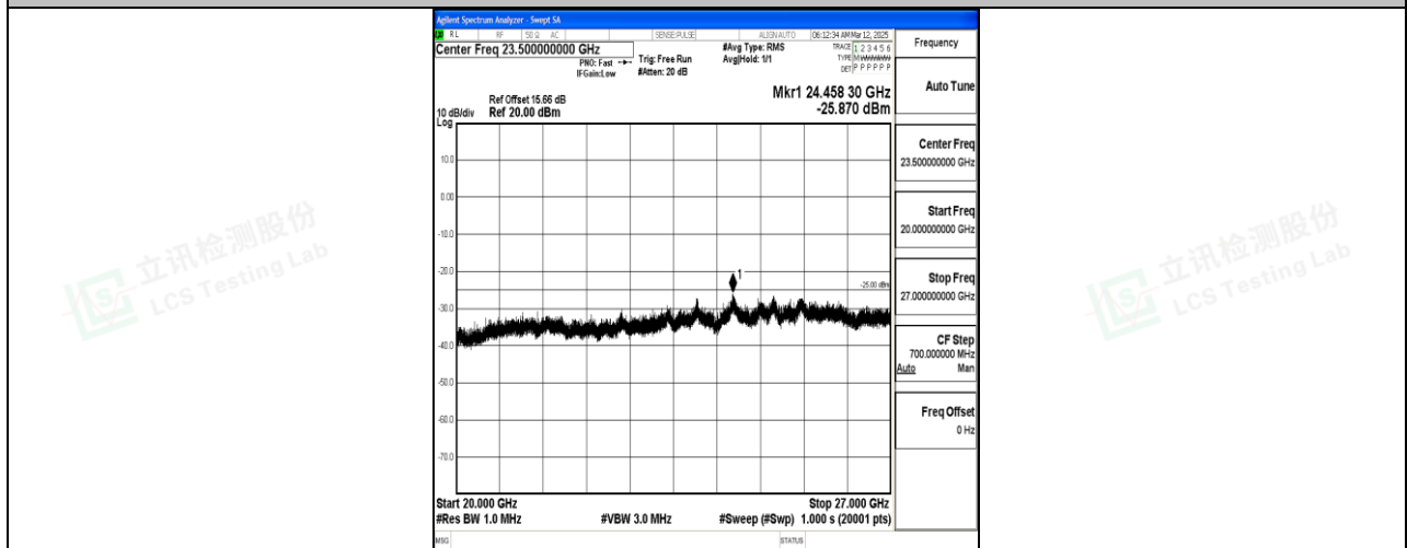
Band7_15MHz_QPSK_21375_1RB#0_20000~27000_20000~27000
