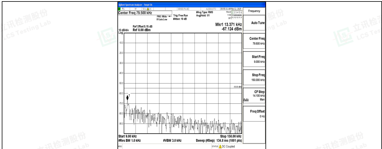
Band7_10MHz_QPSK_21100_1RB#0_0.009~0.15_0.009~0.15
