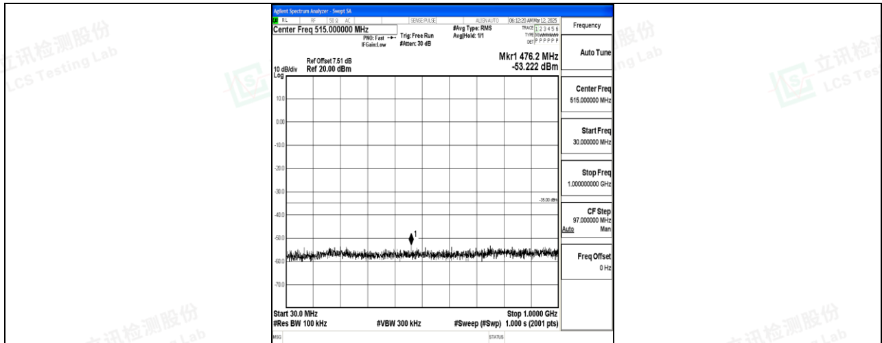
Band7_15MHz_QPSK_21375_1RB#0_30~1000_30~1000
