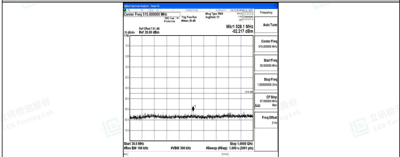
Band7_20MHz_QPSK_20850_1RB#0_30~1000_30~1000
