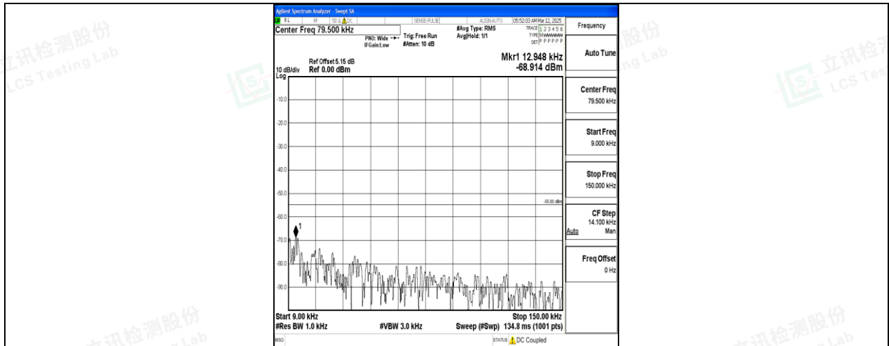
Band7_5MHz_16QAM_21100_1RB#0_0.009~0.15_0.009~0.15
