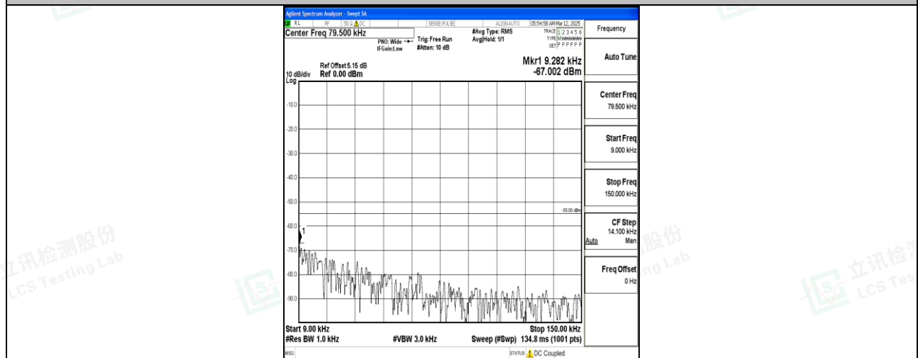
Band7_10MHz_16QAM_20800_1RB#0_0.009~0.15_0.009~0.15
