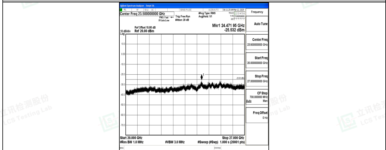
Band7_15MHz_QPSK_21100_1RB#0_20000~27000_20000~27000
