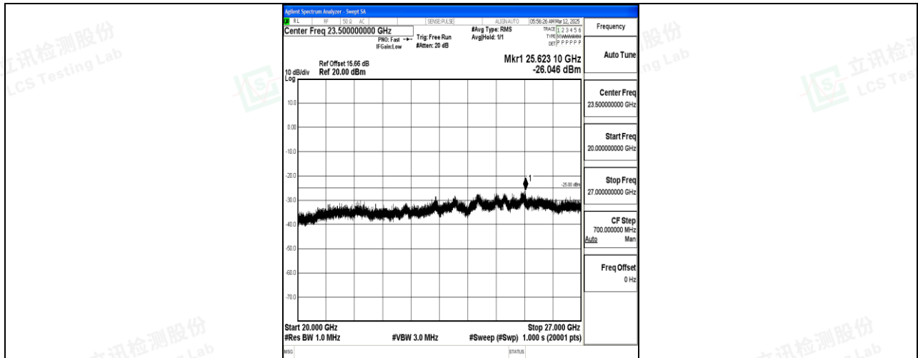
Band7_10MHz_16QAM_21100_1RB#0_20000~27000_20000~27000
