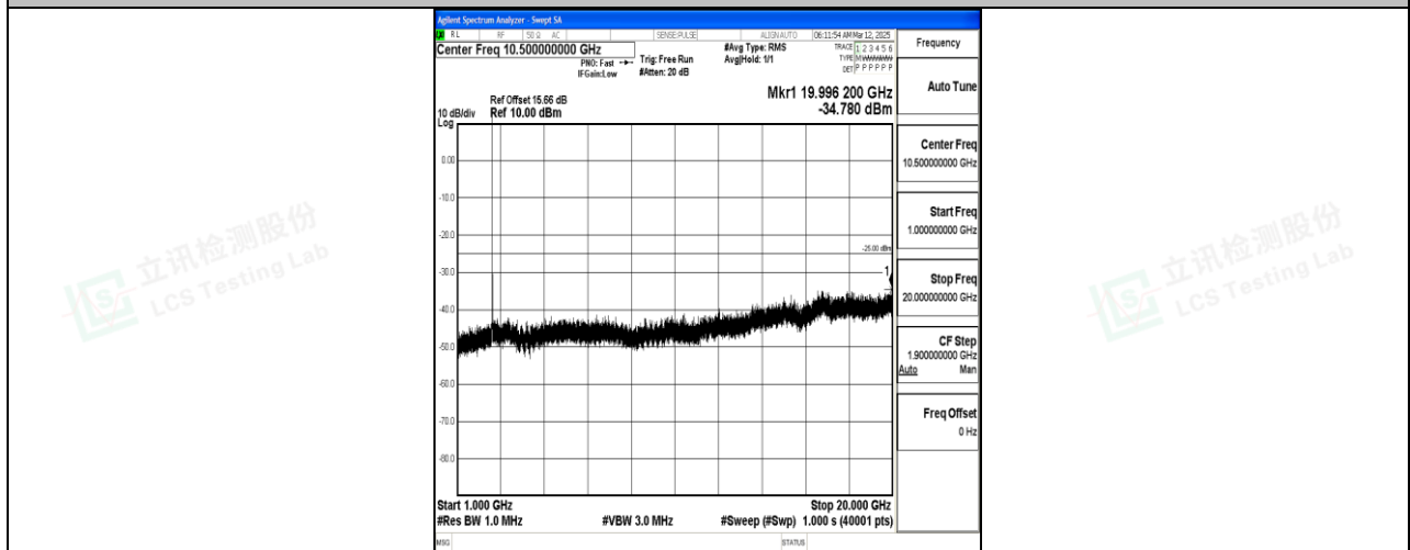
Band7_15MHz_16QAM_21100_1RB#0_1000~20000_1000~20000
