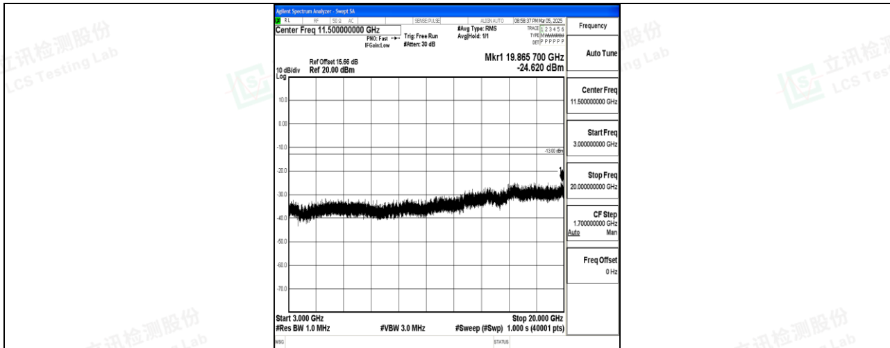
Band4_20MHz_16QAM_20175_1RB#0_3000~20000_3000~20000
