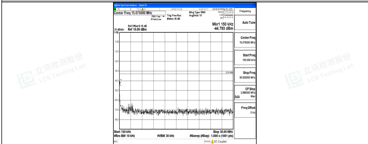
Band4_20MHz_QPSK_20300_1RB#0_0.15~30_0.15~30
