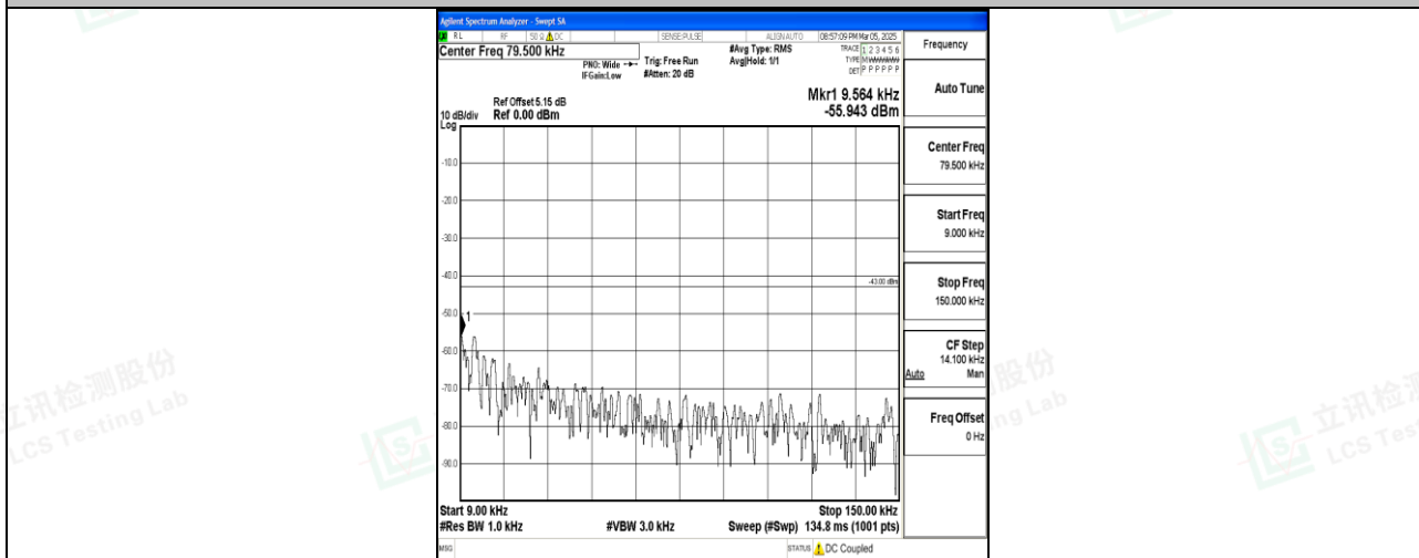
Band4_20MHz_16QAM_20050_1RB#0_0.009~0.15_0.009~0.15
