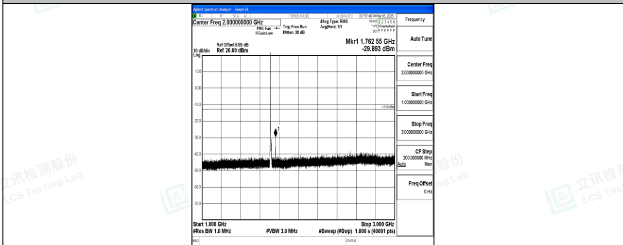
Band4_5MHz_16QAM_19975_1RB#0_1000~3000_1000~3000
