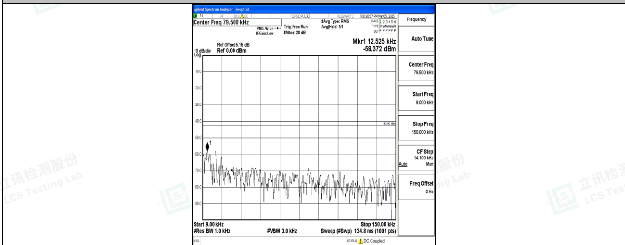
Band4_10MHz_QPSK_20350_1RB#0_0.009~0.15_0.009~0.15
