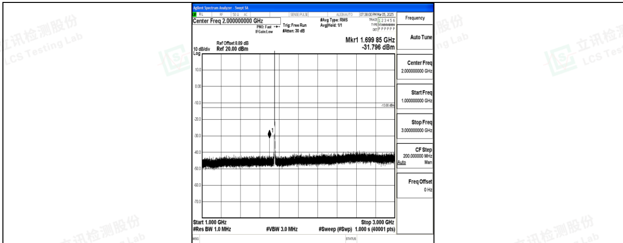
Band4_3MHz_16QAM_20385_1RB#0_1000~3000_1000~3000
