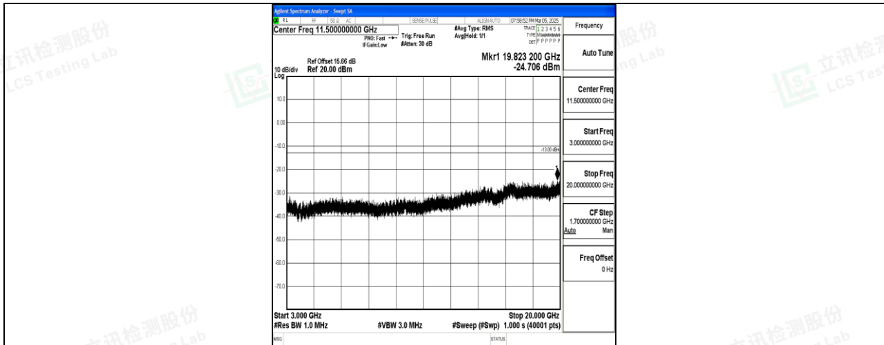
Band4_5MHz_16QAM_20175_1RB#0_3000~20000_3000~20000
