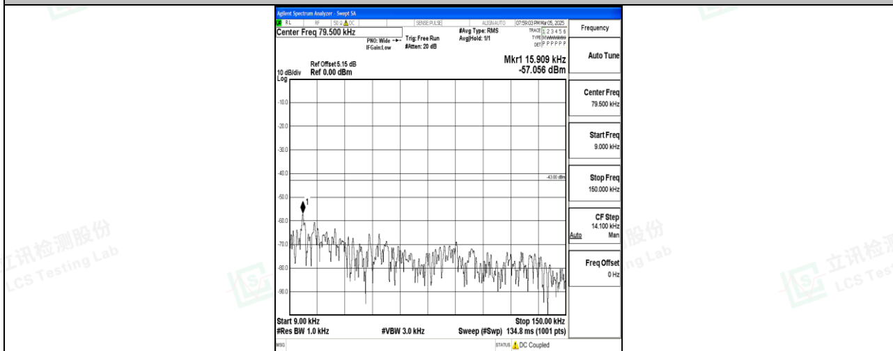
Band4_5MHz_QPSK_20375_1RB#0_0.009~0.15_0.009~0.15
