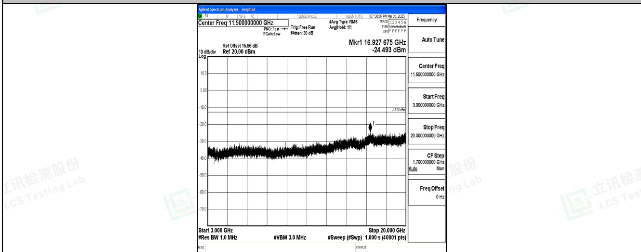
Band4_3MHz_16QAM_20385_1RB#0_3000~20000_3000~20000
