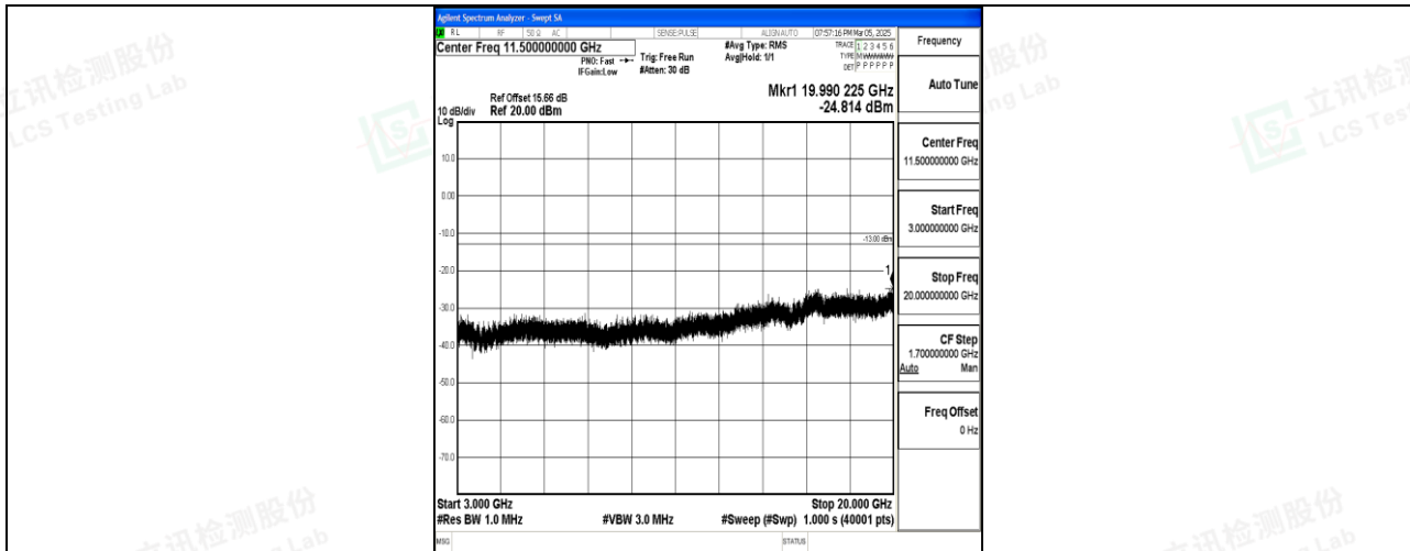
Band4_5MHz_QPSK_19975_1RB#0_3000~20000_3000~20000
