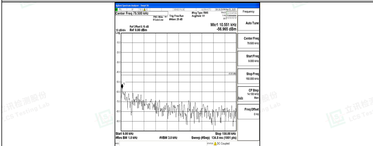
Band4_10MHz_16QAM_20000_1RB#0_0.009~0.15_0.009~0.15
