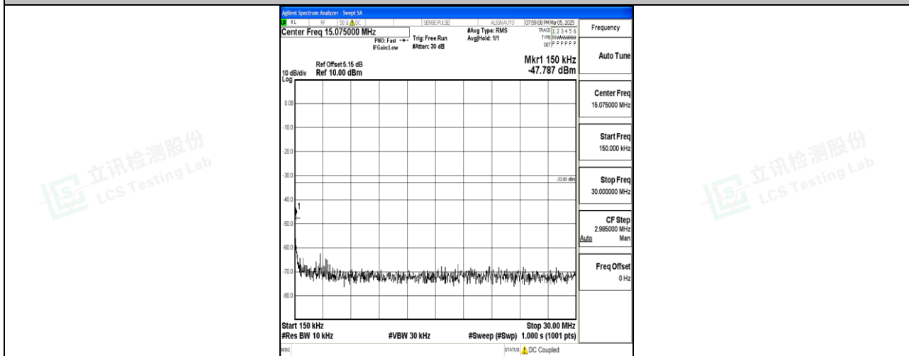
Band4_5MHz_QPSK_20375_1RB#0_0.15~30_0.15~30
