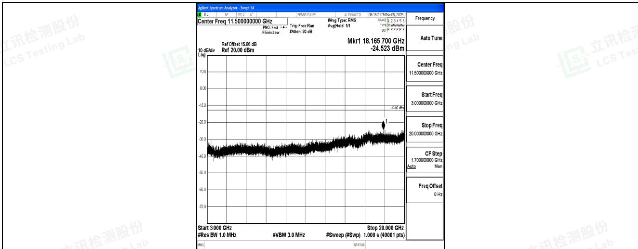
Band4_10MHz_QPSK_20000_1RB#0_3000~20000_3000~20000
