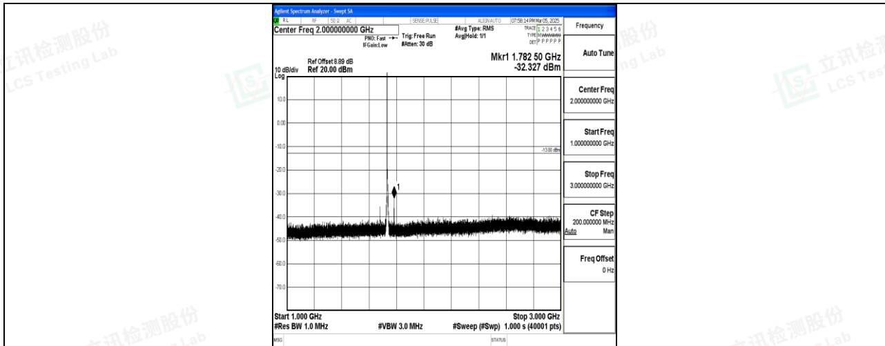
Band4_5MHz_QPSK_20175_1RB#0_1000~3000_1000~3000
