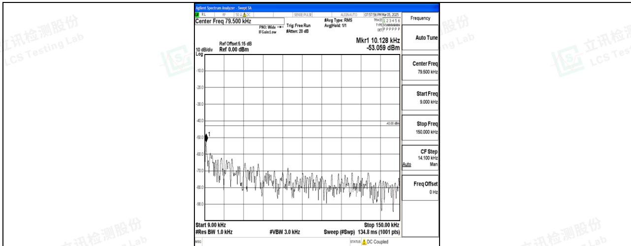
Band4_5MHz_QPSK_20175_1RB#0_0.009~0.15_0.009~0.15
