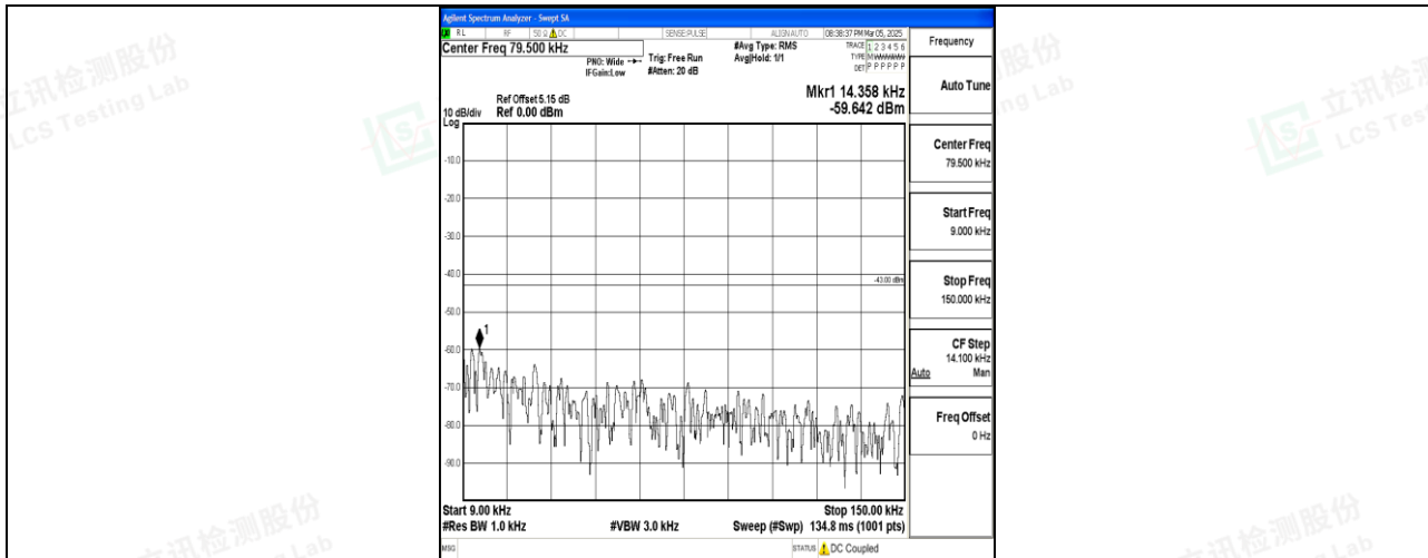
Band4_15MHz_QPSK_20175_1RB#0_0.009~0.15_0.009~0.15
