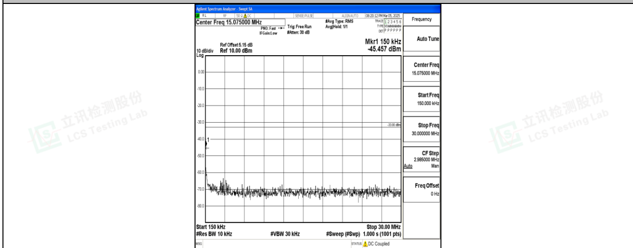
Band4_10MHz_QPSK_20350_1RB#0_0.15~30_0.15~30
