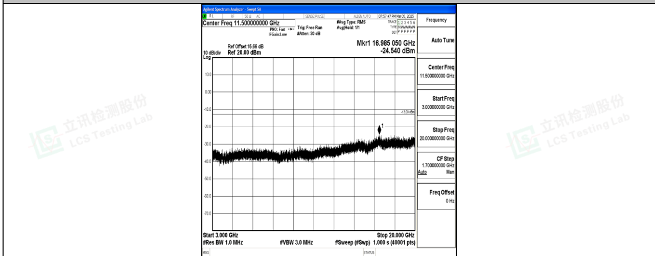
Band4_5MHz_16QAM_19975_1RB#0_3000~20000_3000~20000
