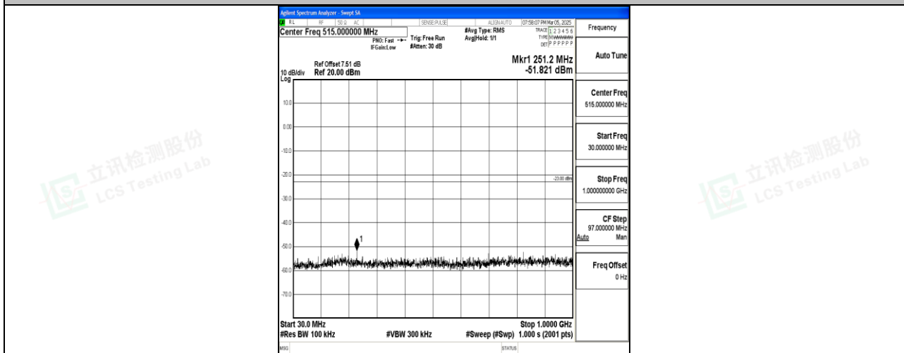
Band4_5MHz_QPSK_20175_1RB#0_30~1000_30~1000
