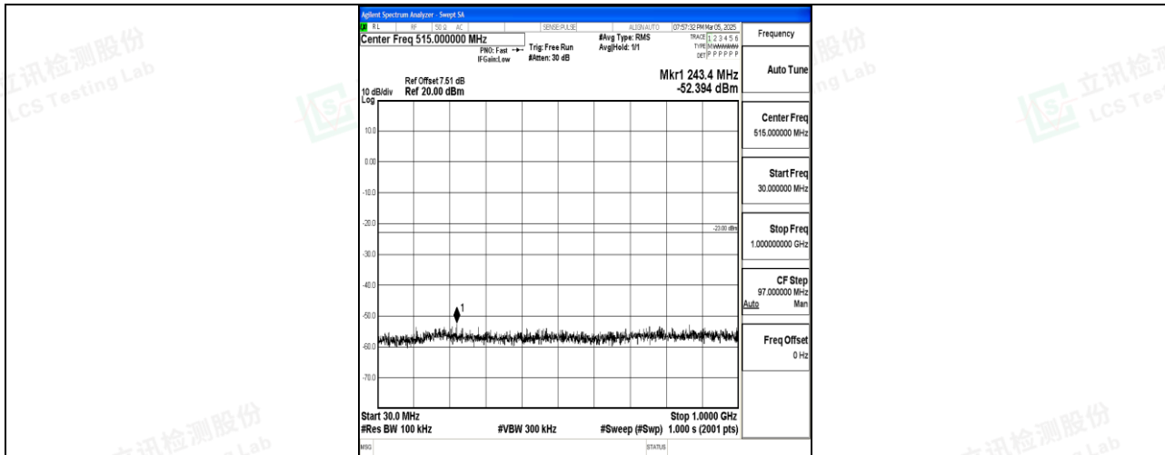
Band4_5MHz_16QAM_19975_1RB#0_30~1000_30~1000
