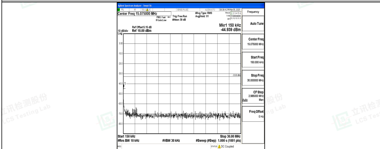
Band4_15MHz_QPSK_20175_1RB#0_0.15~30_0.15~30
