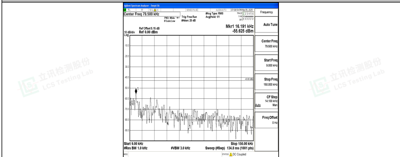
Band4_1.4MHz_16QAM_20175_1RB#0_0.009~0.15_0.009~0.15
