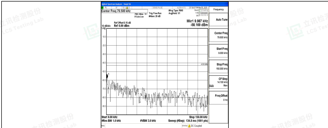
Band4_3MHz_QPSK_20175_1RB#0_0.009-0.15_0.009-0.15
