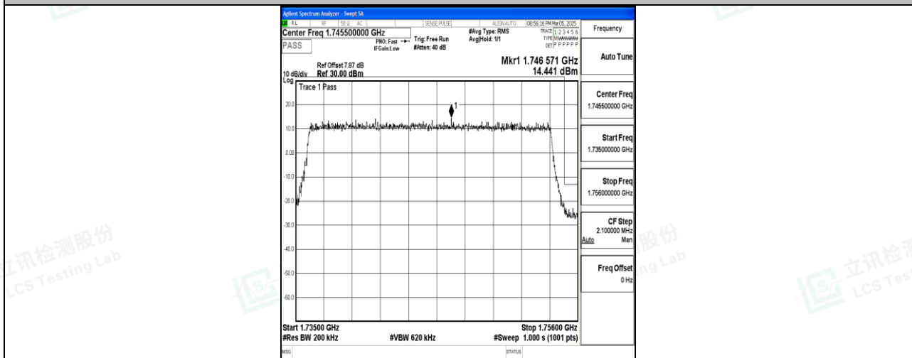
Band4_20MHz_QPSK_20300_100RB#0
