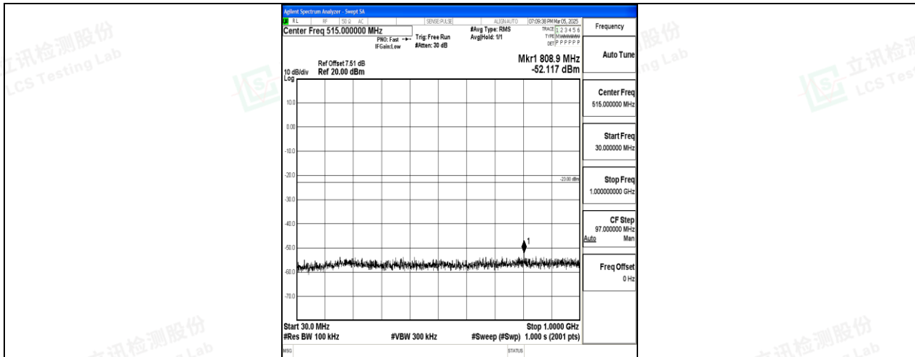
Band4_1.4MHz_QPSK_20393_1RB#0_30~1000_30~1000
