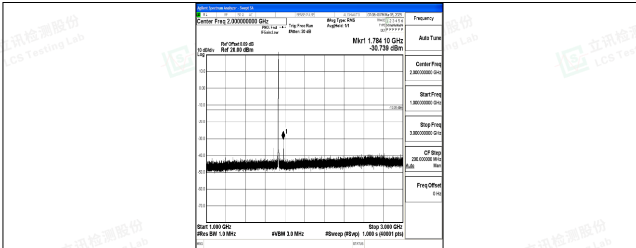
Band4_1.4MHz_QPSK_20175_1RB#0_1000~3000_1000~3000
