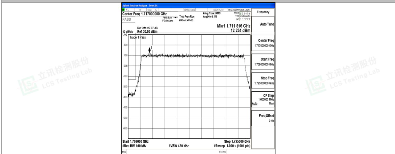
Band4_15MHz_16QAM_20025_75RB#0
