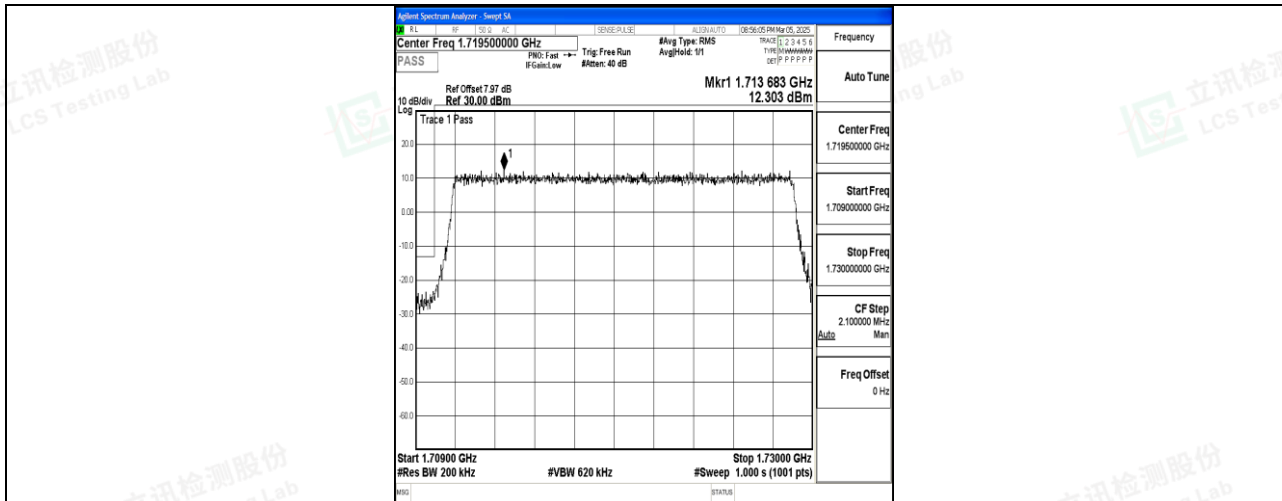
Band4_20MHz_16QAM_20050_100RB#0
