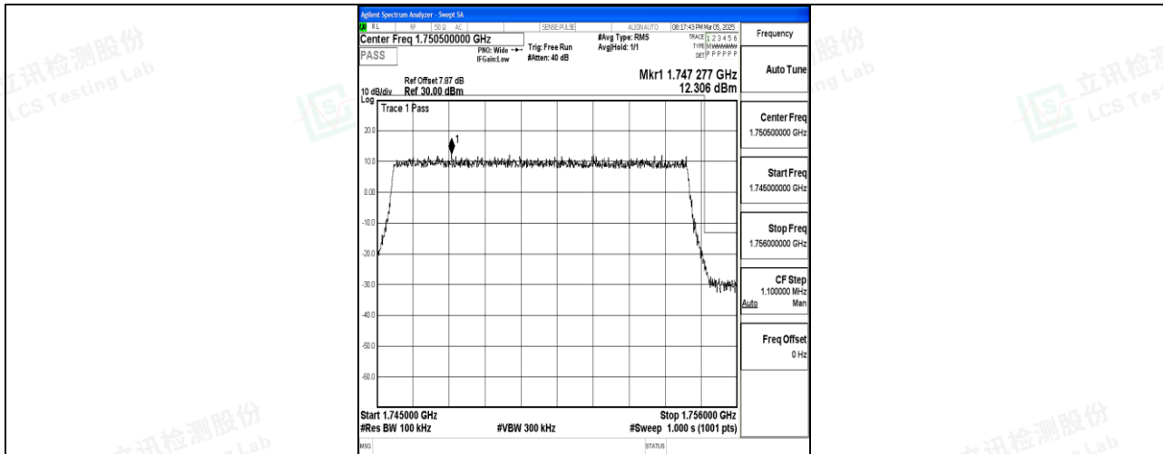
Band4_10MHz_16QAM_20350_50RB#0
