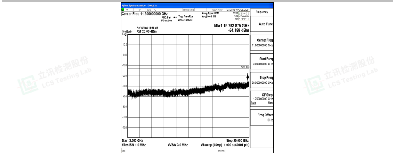
Band4_1.4MHz_QPSK_20393_1RB#0_3000~20000_3000~20000
