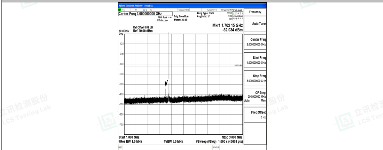
Band4_1.4MHz_QPSK_20393_1RB#0_1000~3000_1000~3000
