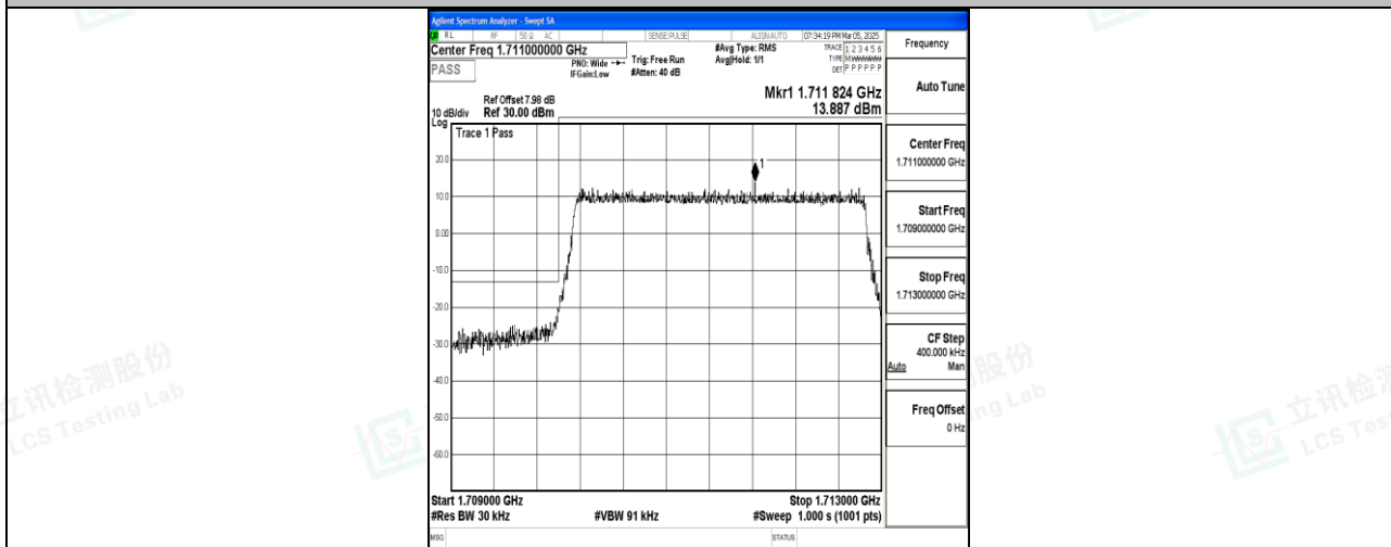
Band4_3MHz_QPSK_19965_15RB#0
