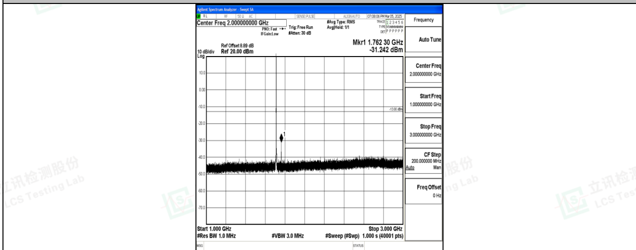
Band4_1.4MHz_16QAM_19957_1RB#0_1000~3000_1000~3000
