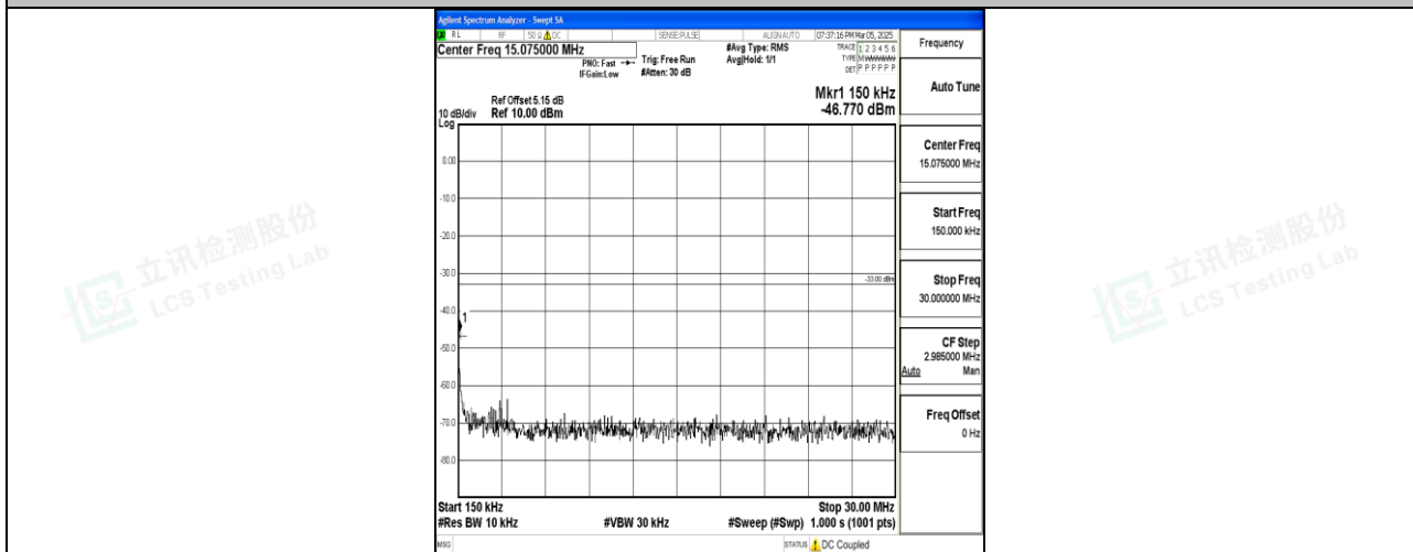
Band4_3MHz_QPSK_20385_1RB#0_0.15~30_0.15~30
