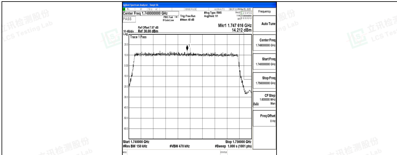
Band4_15MHz_QPSK_20325_75RB#0
