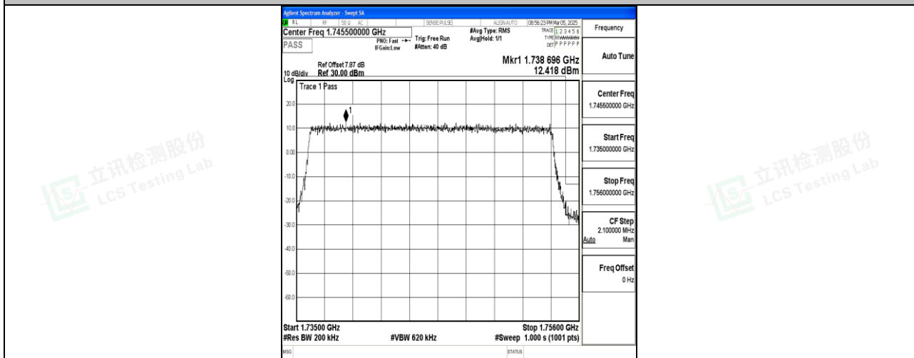
Band4_20MHz_16QAM_20300_100RB#0
