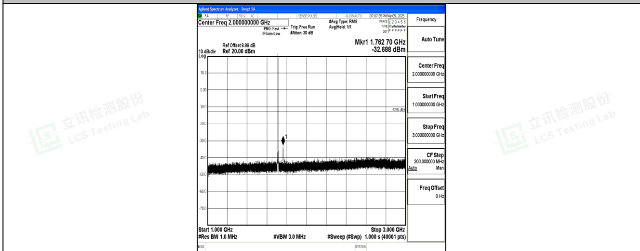
Band4_1.4MHz_QPSK_19957_1RB#0_1000~3000_1000~3000
