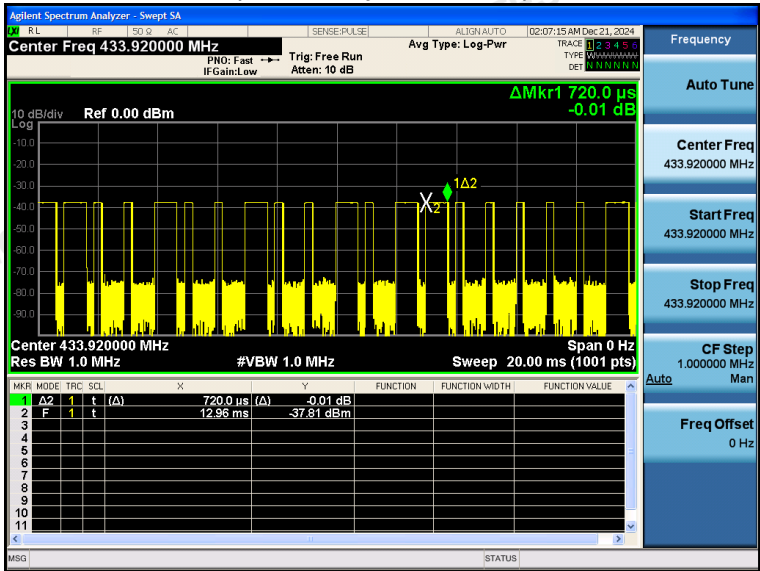
(Time per burst: 0.72ms*12pcs)
