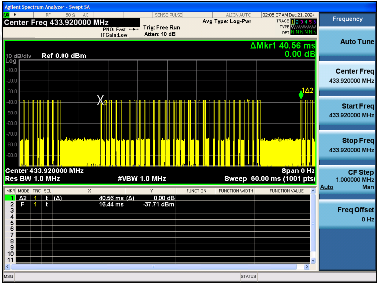
(Transmit cycle 40.56ms)
