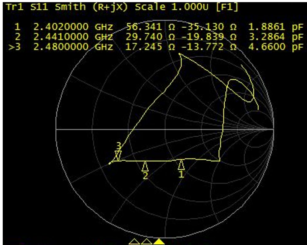
Smith Chart
