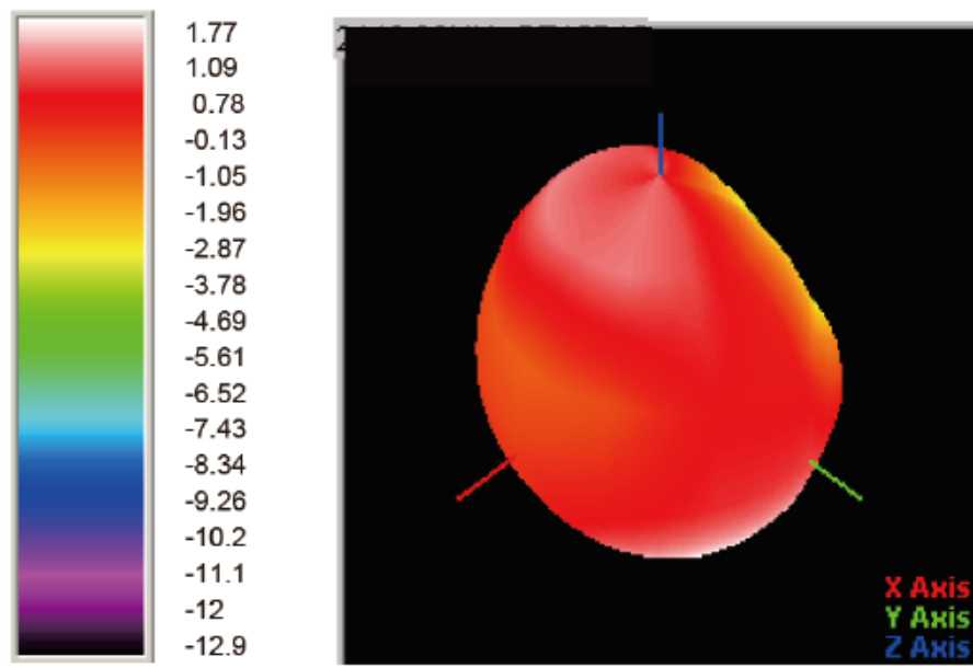
© 3D Gain Pattern (2500 MHz) Unit: dBi
