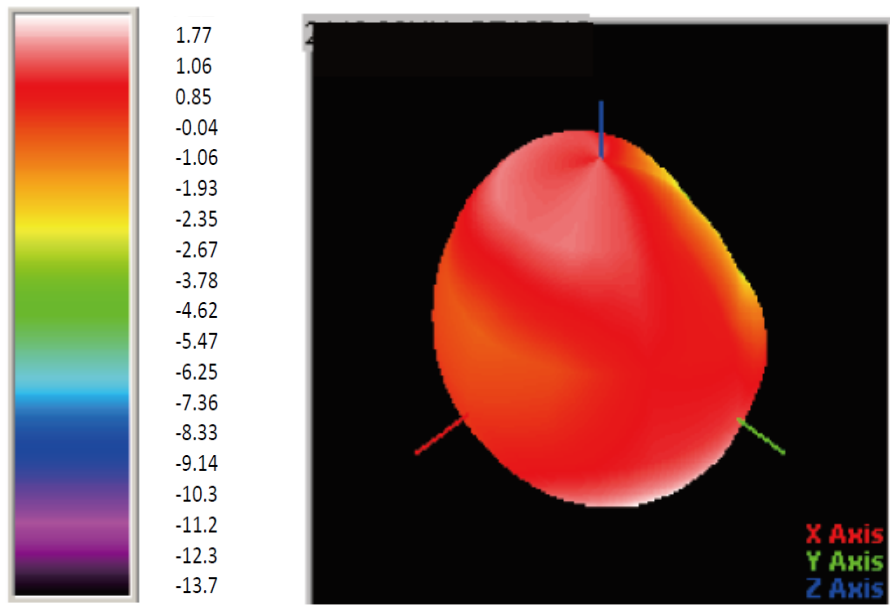
© 3D Gain Pattern (2500 MHz) Unit: dBi
