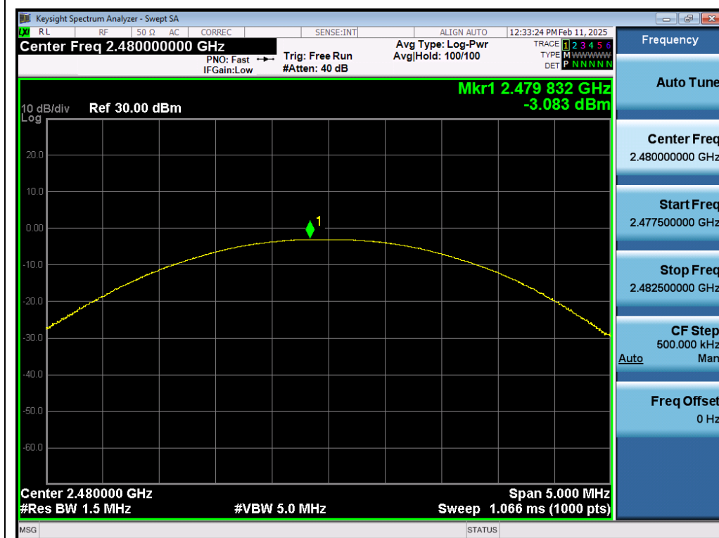
Test_Graph_EDR_ANT1_2480_2Mbps_Peak Power
