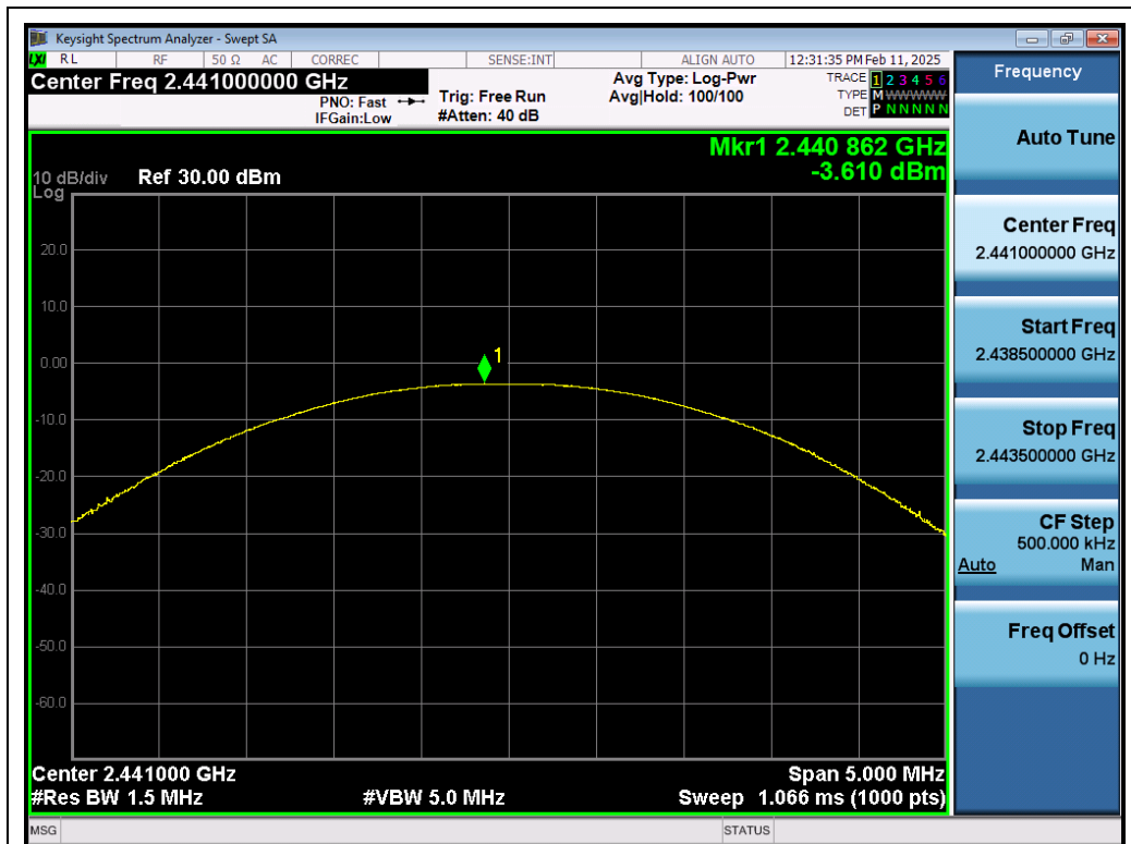
Test_Graph_EDR_ANT1_2441_2Mbps_Peak Power
