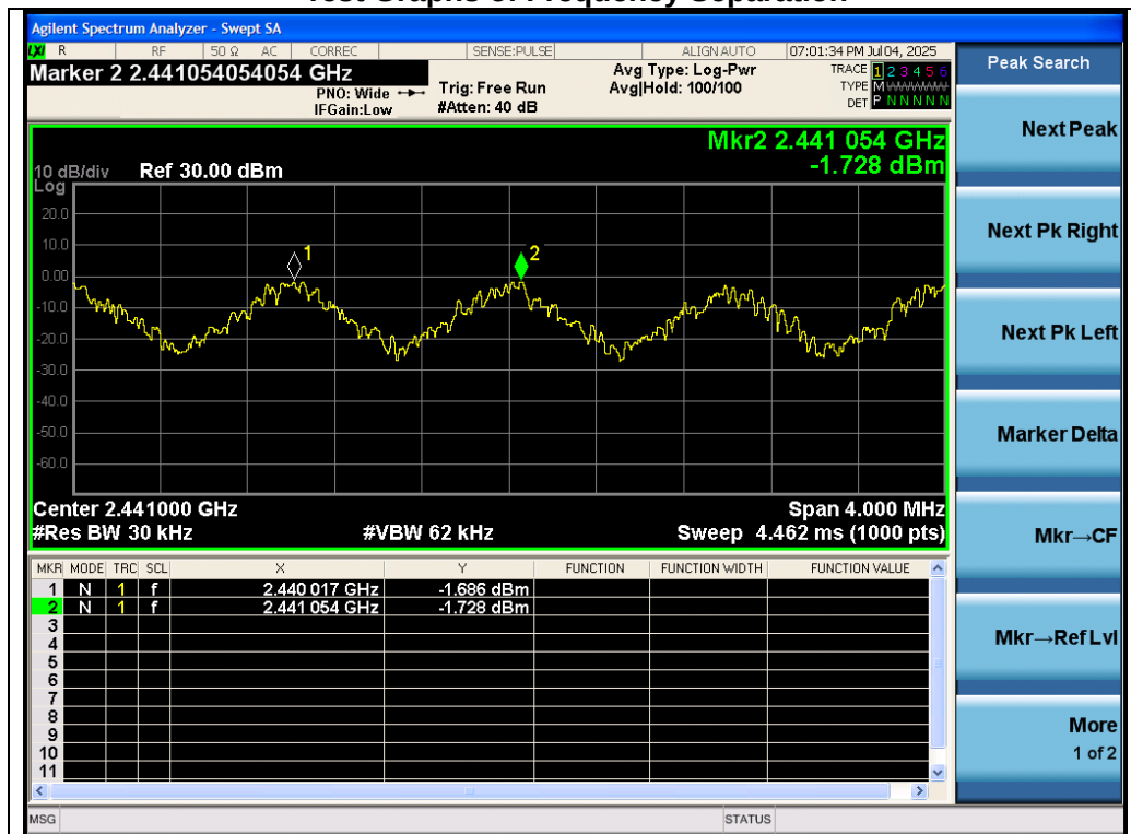
Test_Graph_BR_HOP_ANT1_NA_1Mbps_Hopping Separation
