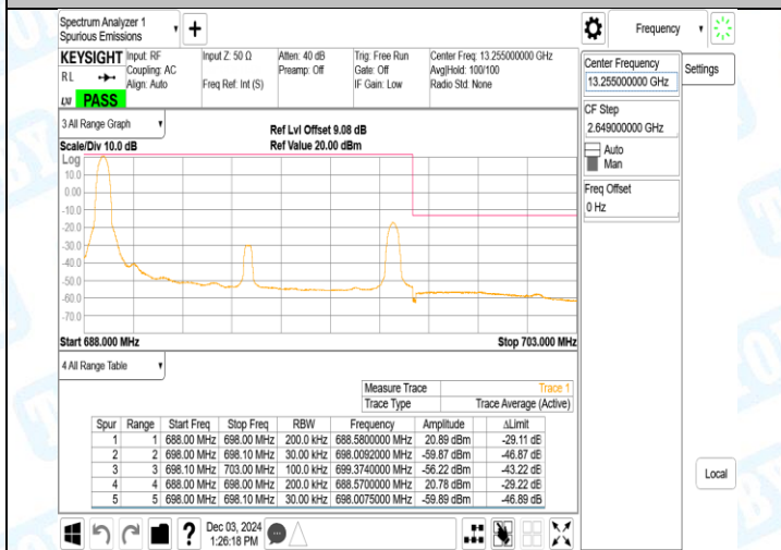
Band71_15MHz_QPSK_133197_1RB#0
