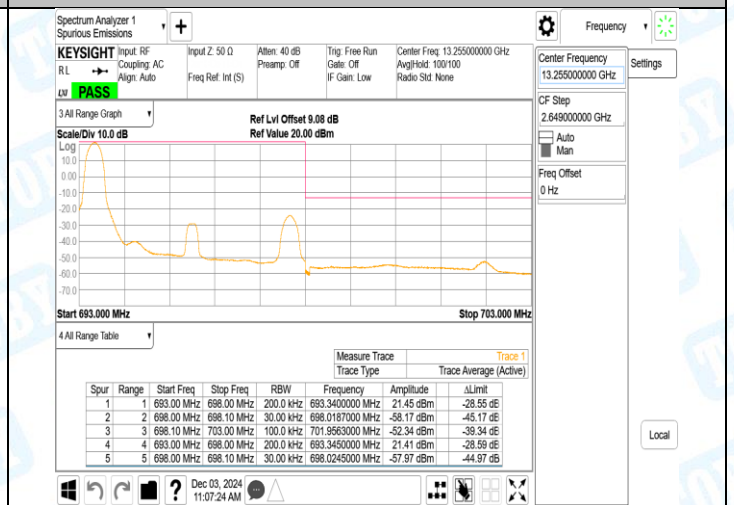
Band71_5MHz_16QAM_133447_25RB#0
