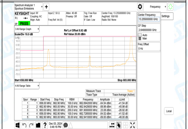
Band71_20MHz_QPSK_133372_1RB#0
