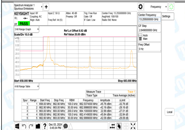
Band71_20MHz_16QAM_133372_1RB#0
