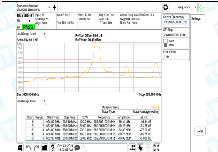
Band71_5MHz_16QAM_133147_25RB#0
