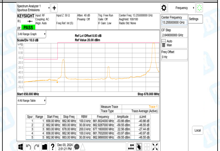
Band71_15MHz_16QAM_133397_1RB#74
