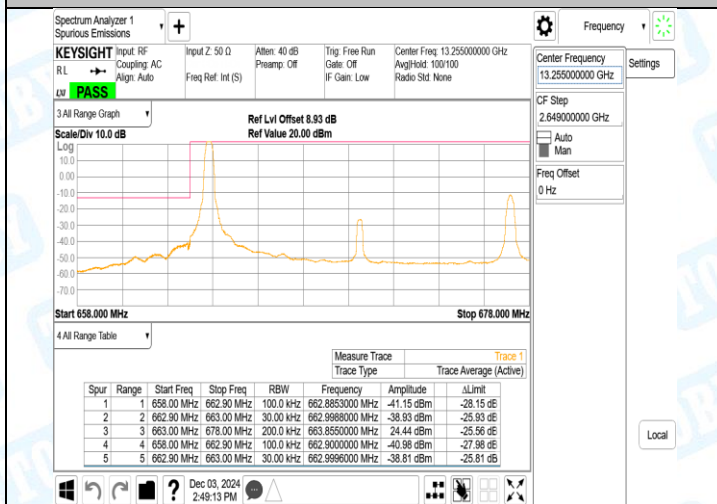
Band71_15MHz_QPSK_133197_75RB#0
