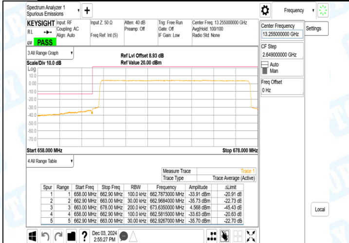
Band71_15MHz_QPSK_133397_1RB#74
