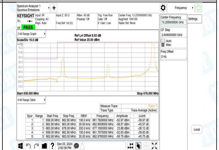
Band71_15MHz_QPSK_133397_1RB#0
