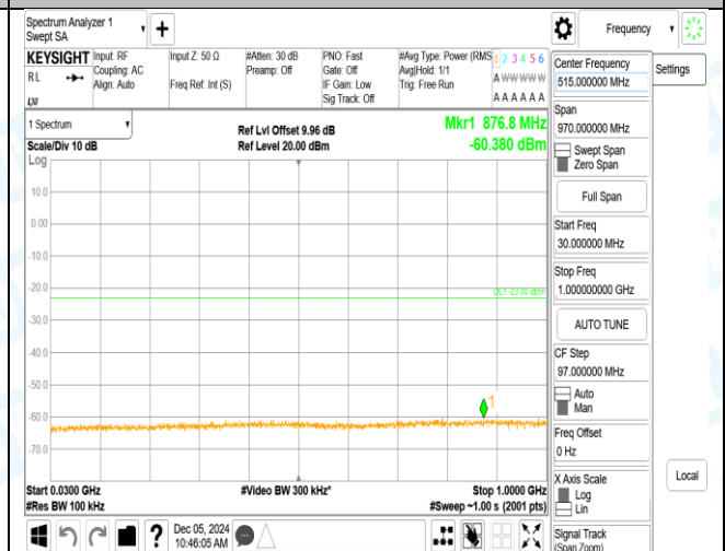
Band66_20MHz_16QAM_132072_1RB#0_3000~20000_3000~20000
