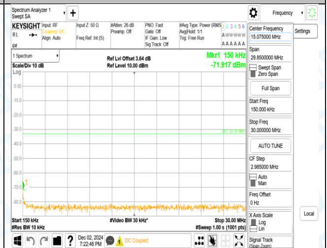
Band66_3MHz_16QAM_132657_1RB#14_1000-3000_1000-3000
