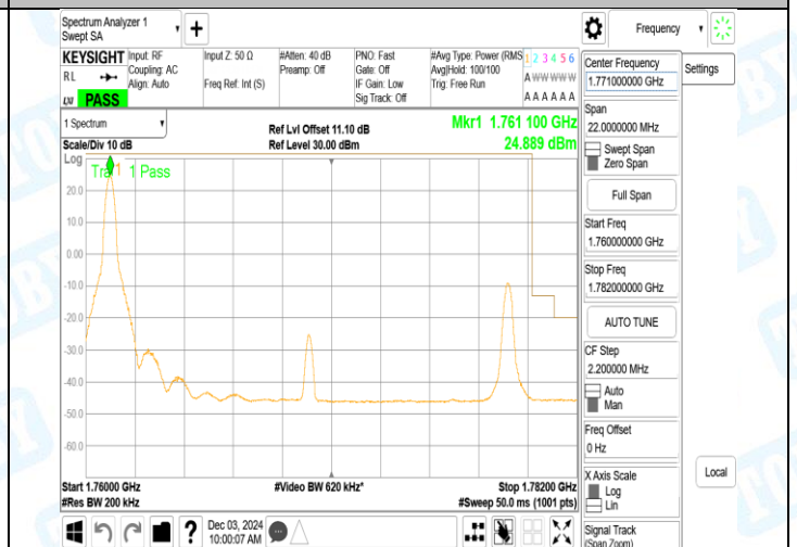
Band66_20MHz_QPSK_132572_100RB#0
