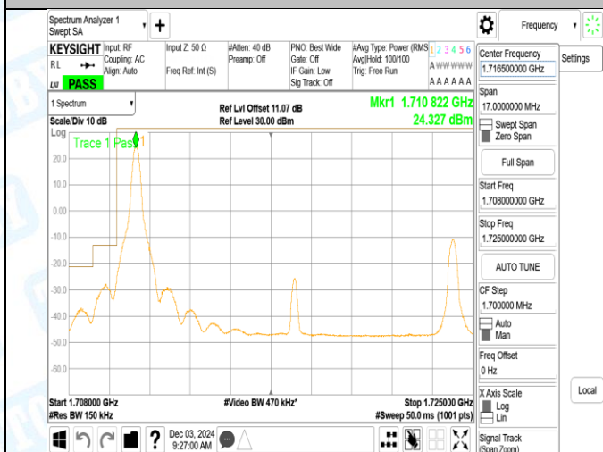
Band66_15MHz_QPSK_132047_75RB#0
