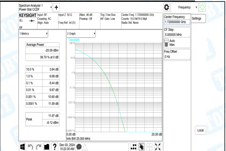
Band66-20MHz-QPSK-132322-100RB#0-PASS
