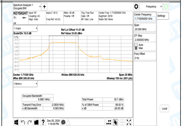
Band66-10MHz-16QAM-132622-27RB#0-PASS
