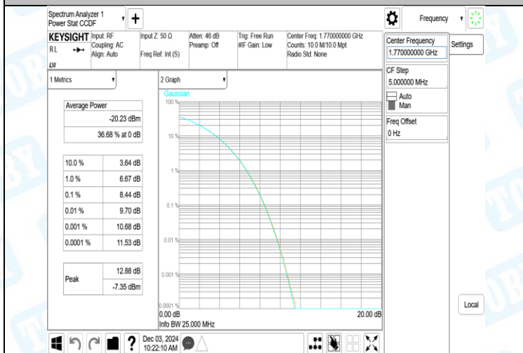
Band66-20MHz-16QAM-132072-1RB#0-PASS
