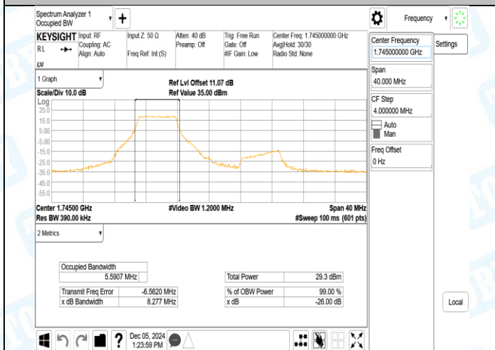
Band66-20MHz-16QAM-132322-27RB#0-PASS
