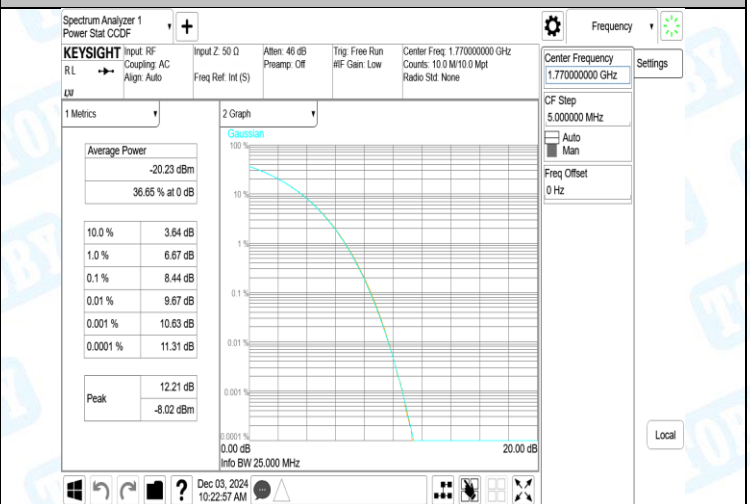
Band66-20MHz-16QAM-132072-27RB#0-PASS
