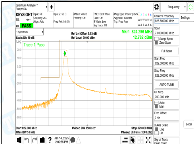
Band5_5MHz_QPSK_20425_25RB#0
