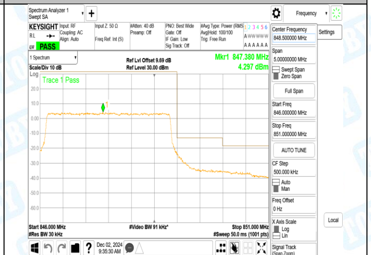
Band5_3MHz_16QAM_20415_1RB#14
