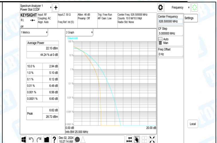
Band5-5MHz-16QAM-20525-25RB#0-PASS
