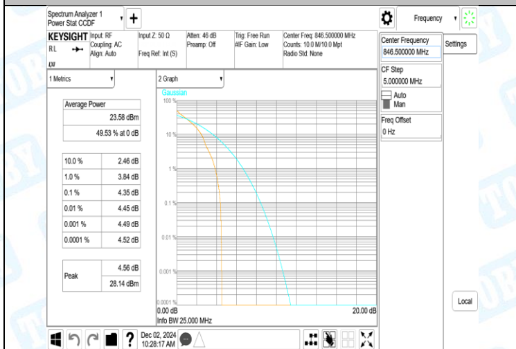
Band5-5MHz-16QAM-20425-1RB#0-PASS
