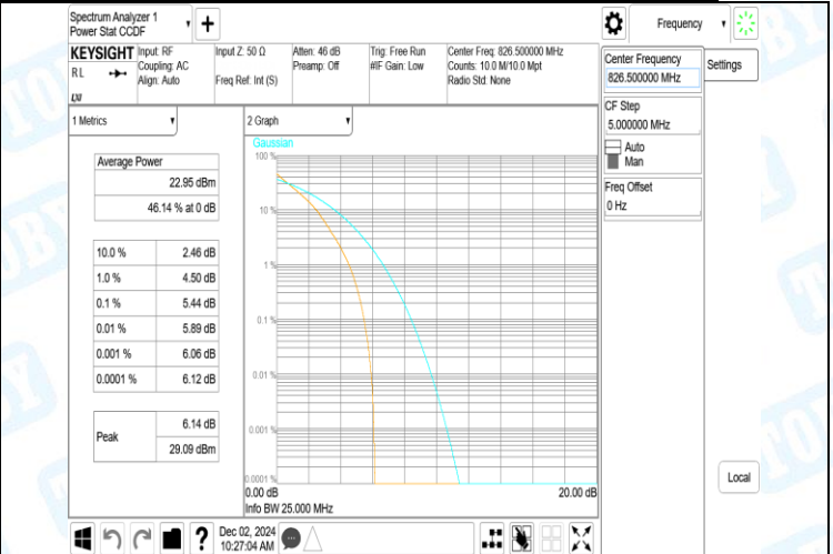
Band5-5MHz-QPSK-20525-25RB#0-PASS
