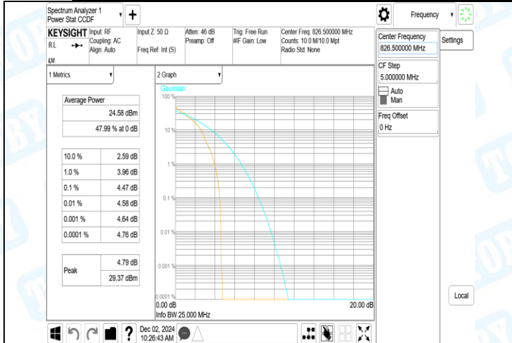
Band5-5MHz-QPSK-20525-1RB#0-PASS
