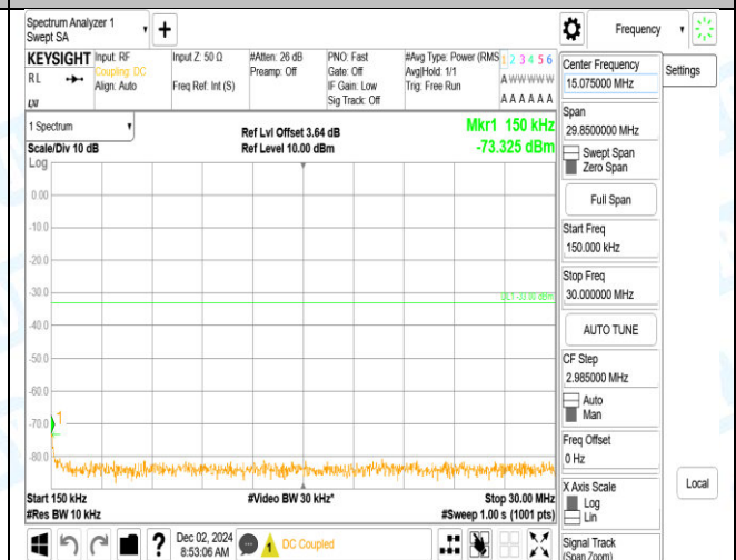
Band4_20MHz_QPSK_20300_100RB#0_1000-3000_1000-3000
