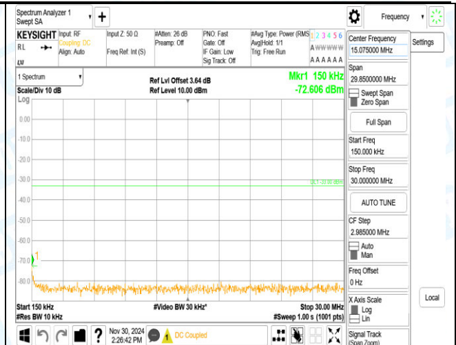
Band4_10MHz_QPSK_20350_1RB#0_1000-3000_1000-3000
