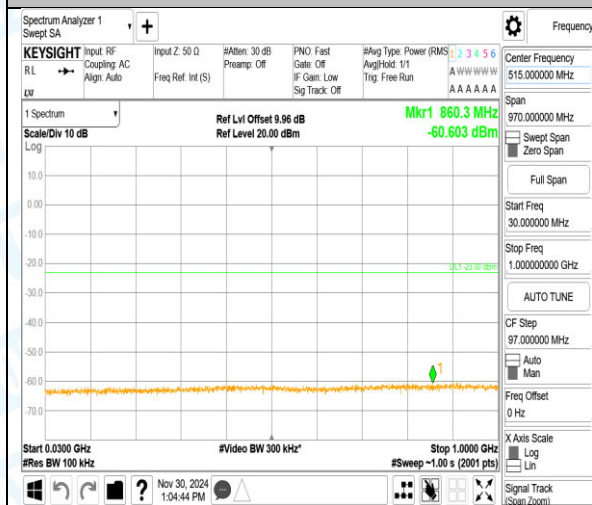
Band4_3MHz_16QAM_20175_1RB#0_3000~20000_3000~20000
