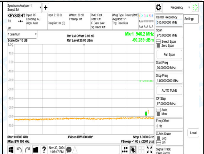
Band4_3MHz_16QAM_20175_1RB#14_3000-20000_3000-20000
