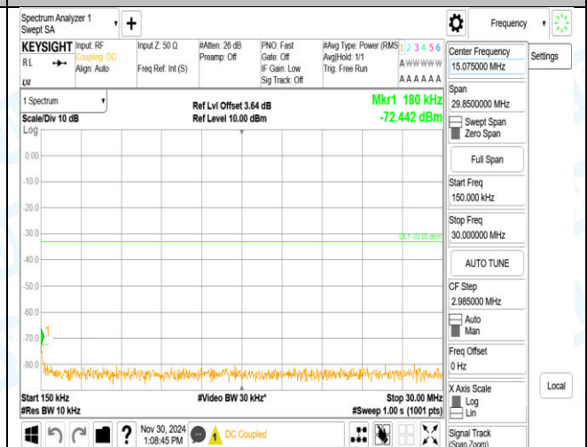
Band4_3MHz_16QAM_20175_15RB#0_1000-3000_1000-3000
