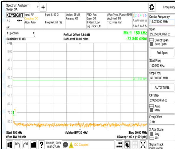
Band4_1.4MHz_QPSK_19957_1RB#5_1000-3000_1000-3000
