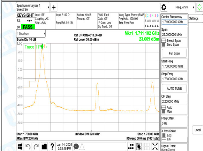
Band4_20MHz_16QAM_20050_1RB#0
