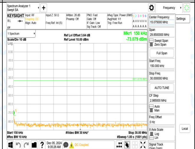
Band4_1.4MHz_QPSK_19957_6RB#0_1000-3000_1000-3000
