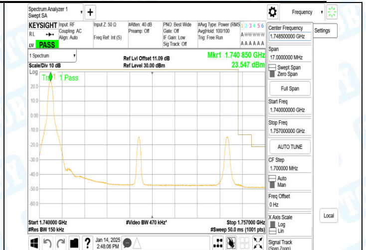
Band4_15MHz_QPSK_20325_75RB#0
