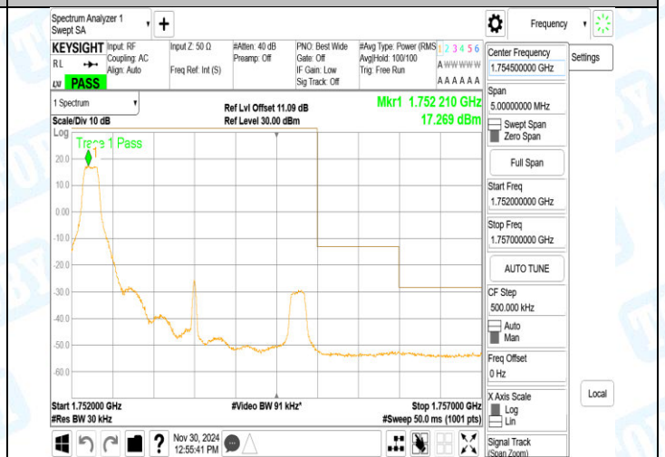
Band4_3MHz_QPSK_20385_15RB#0
