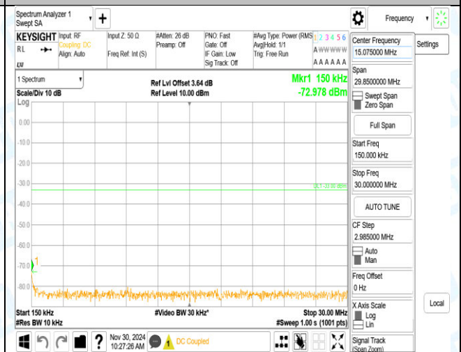
Band2_10MHz_16QAM_18650_1RB#49_1000-3000_1000-3000
