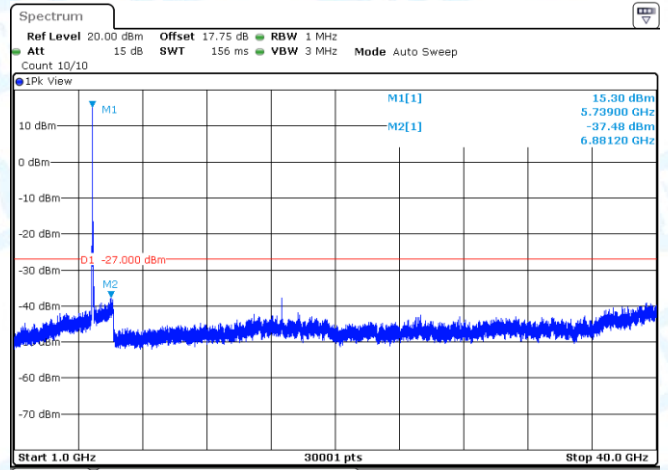
11AX20SISO-Ant1-5745-1000~40000-PASS
