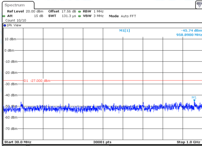
11AC20SISO-Ant1-5500-30~1000-PASS
