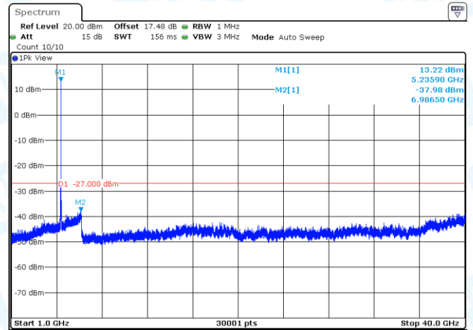
11AX20SISO-Ant1-5200-1000~40000-PASS
