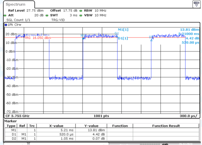
NTNV-11N40SISO-Ant1-5755
